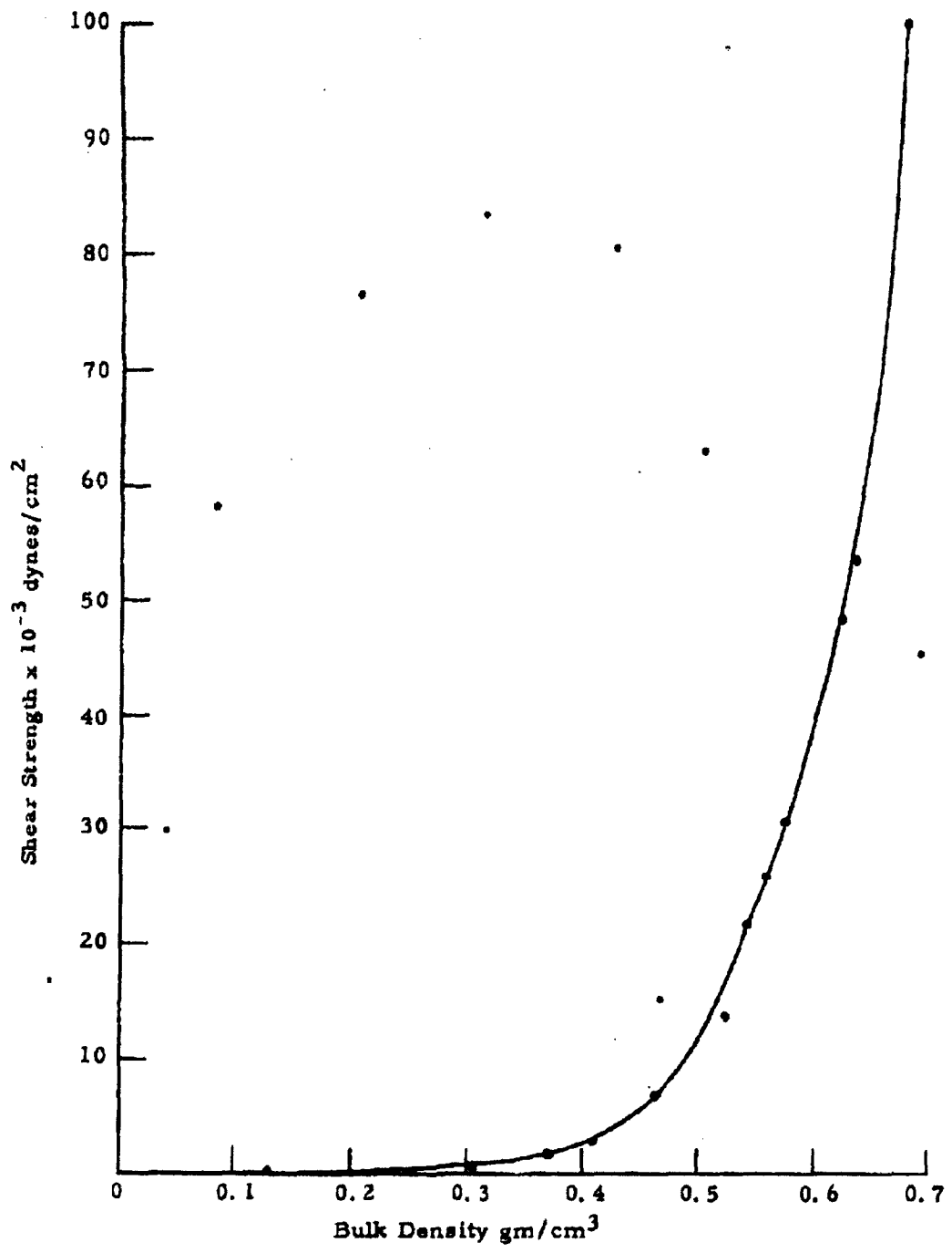
Figure 3.6 Shear Strength of Talc Powder as a Function of Bulk Density
