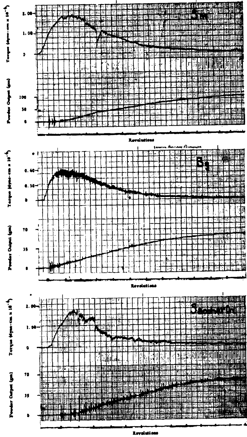
Figure 3.15 Screw Feeder Torque and Output Data for Sm , Bg , and Saccharin Powders
