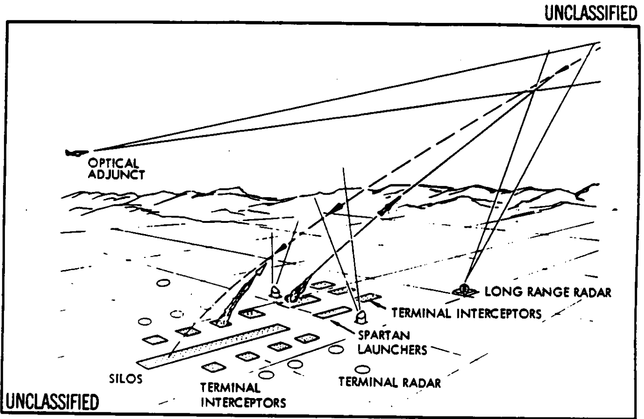
Figure 5.3-1. (U) Closely Spaced Basing Defense System
