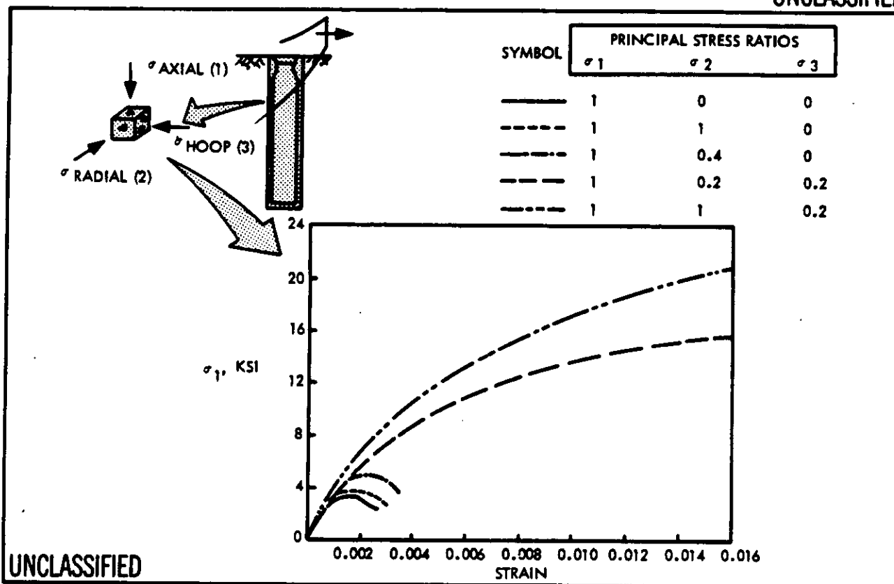
Figure 5.1.1-1. (U) Effect of Confining Stresses on Stress-Strain Properties of Concrete
