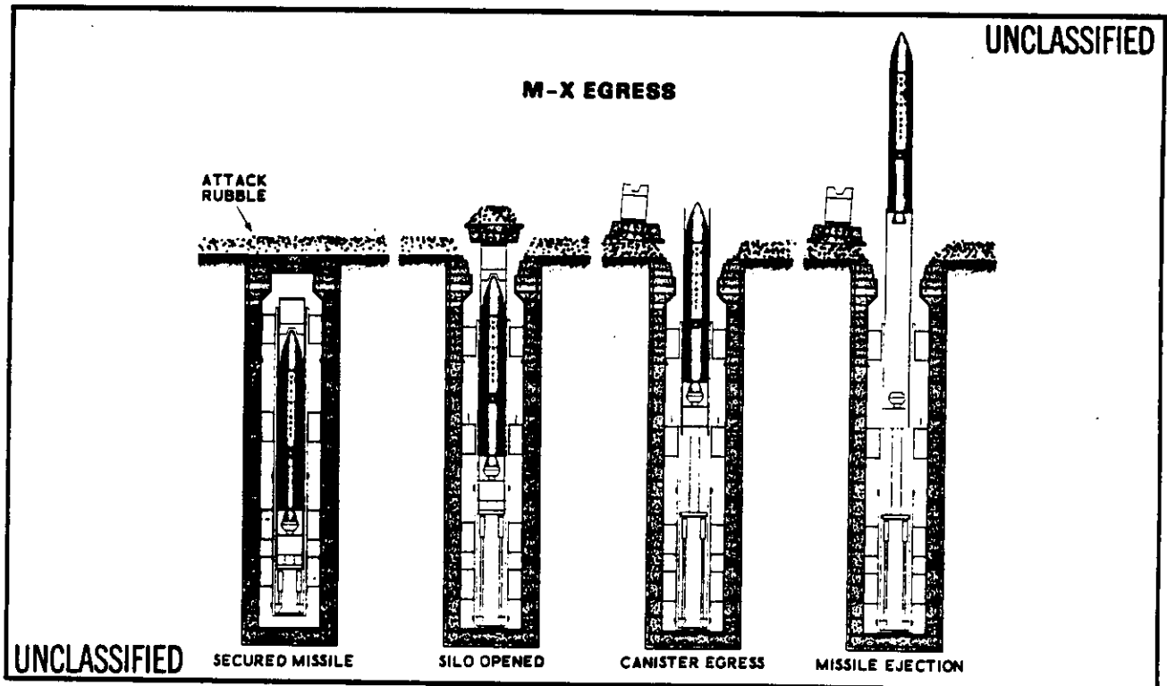
Figure 5.1.1-6 (U) Egress Sequence
