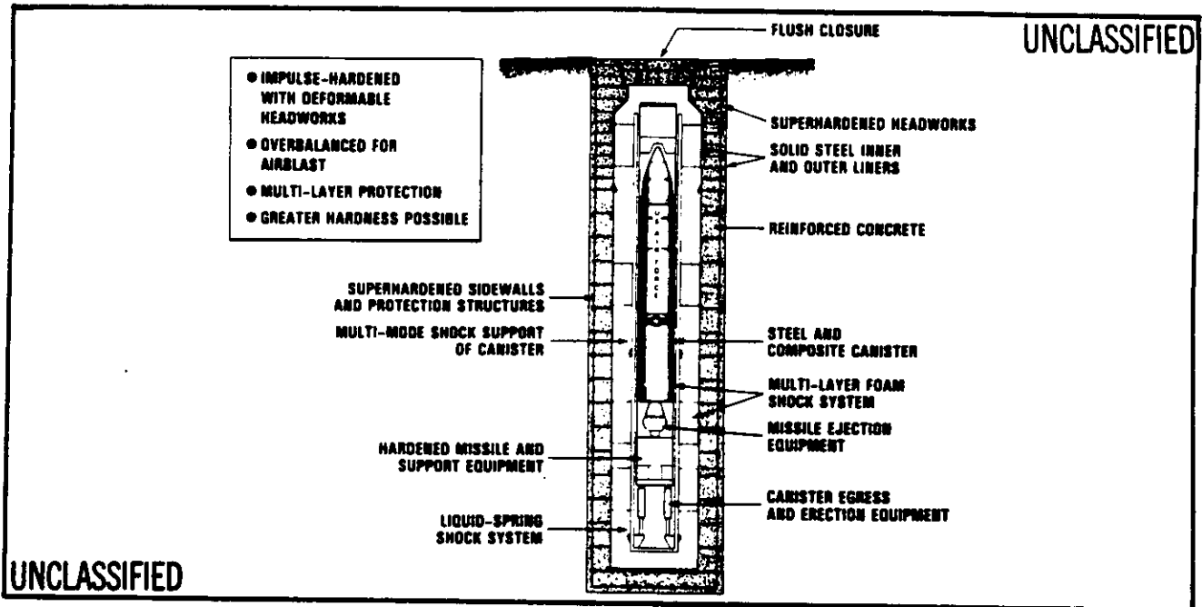
Figure 5.1.1-5 (U) Superhard Silo
