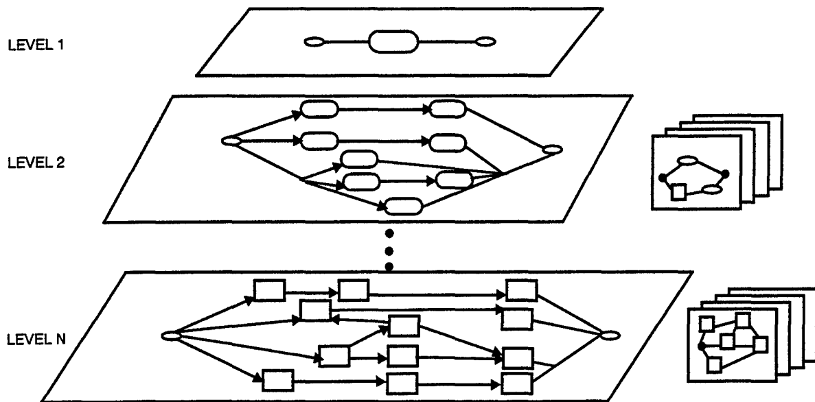
Figure 2. Hierarchical Planning
