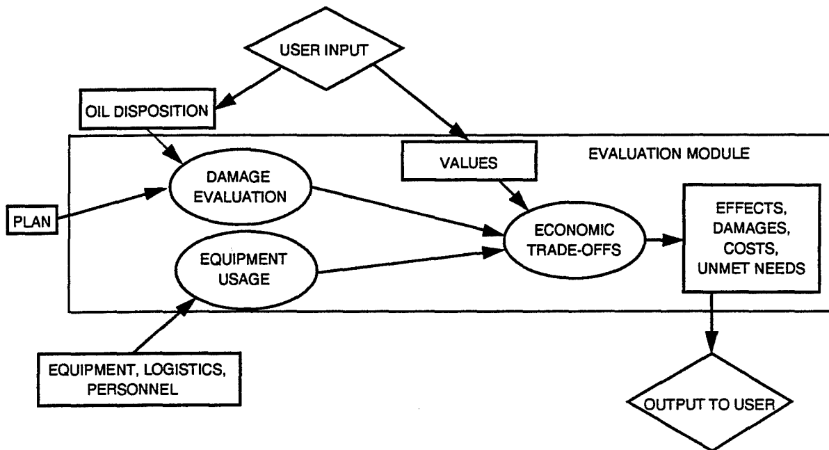
Figure 3. Evaluation Module
