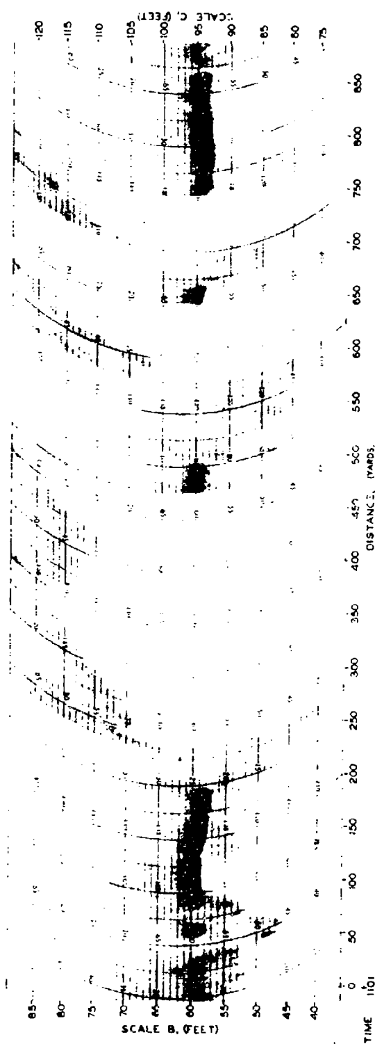
Figure 50. NK fathometer record, USS BOARFISH under-ice dive.
