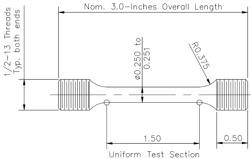
Figure 3–6. Round tensile specimen used for room-temperature and elevated-temperature tensile tests.
