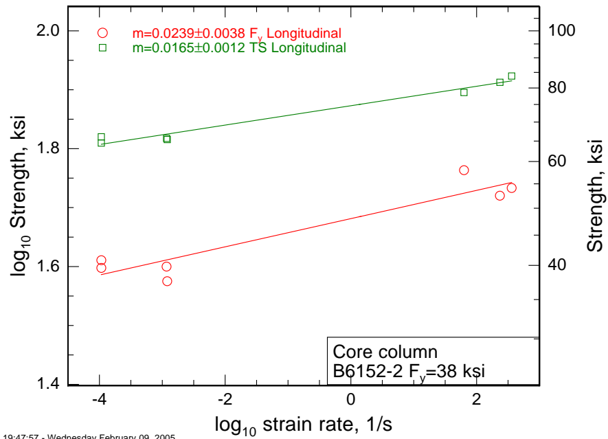
Figure A-76. Strain rate sensitivity for F_y = 36 ksi box column B6152-FL longitudinal.
