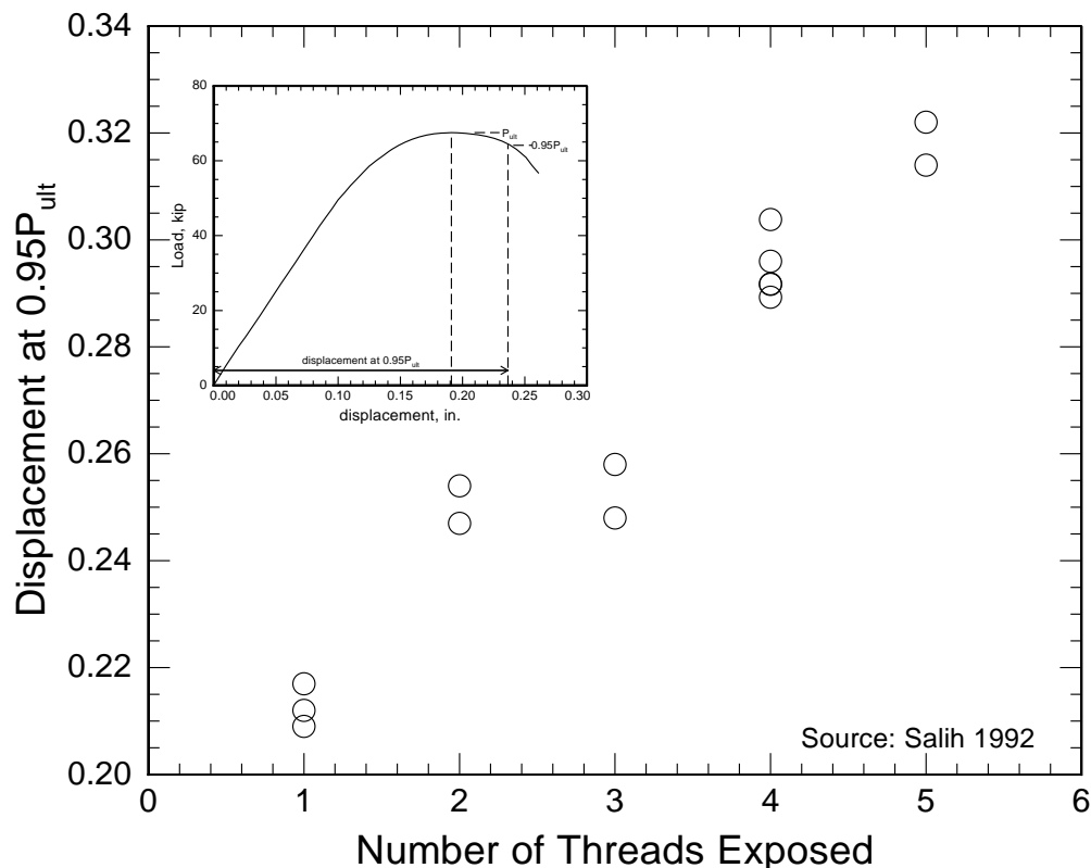
Figure 3–30. Displacement near failure of A 325 bolts as a function of number of threads exposed.
