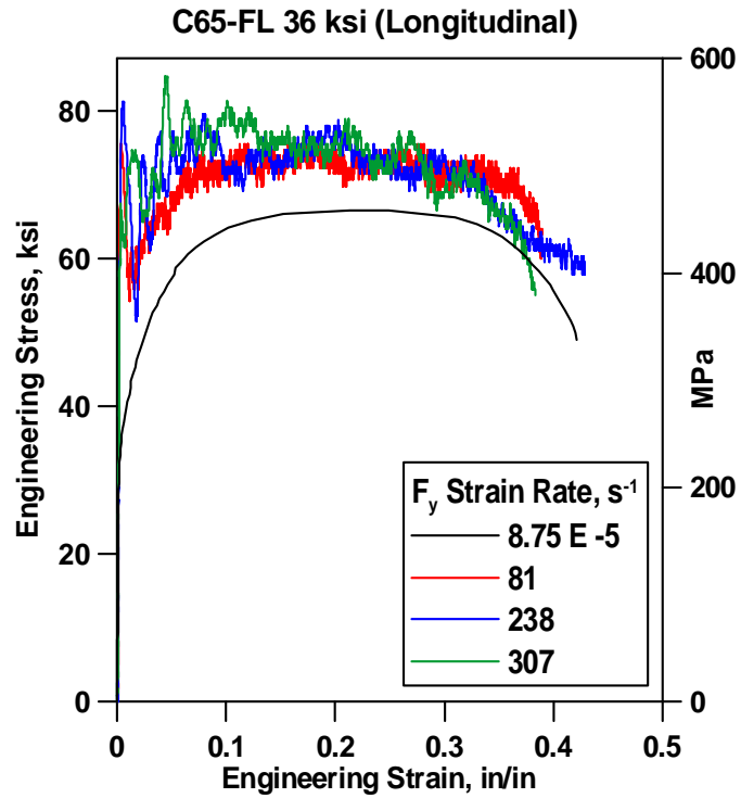
Figure A-44. Stress-strain curves for F_y = 36 ksi core wide-flange C65-FL longitudinal.
