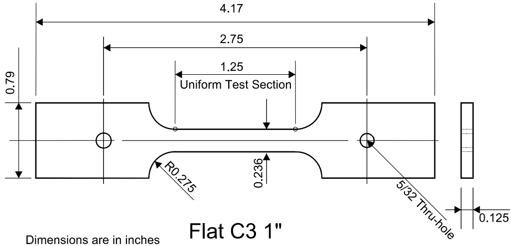
Figure 3–5. Flat tensile test specimen used for some creep and elevated-temperature tests.
