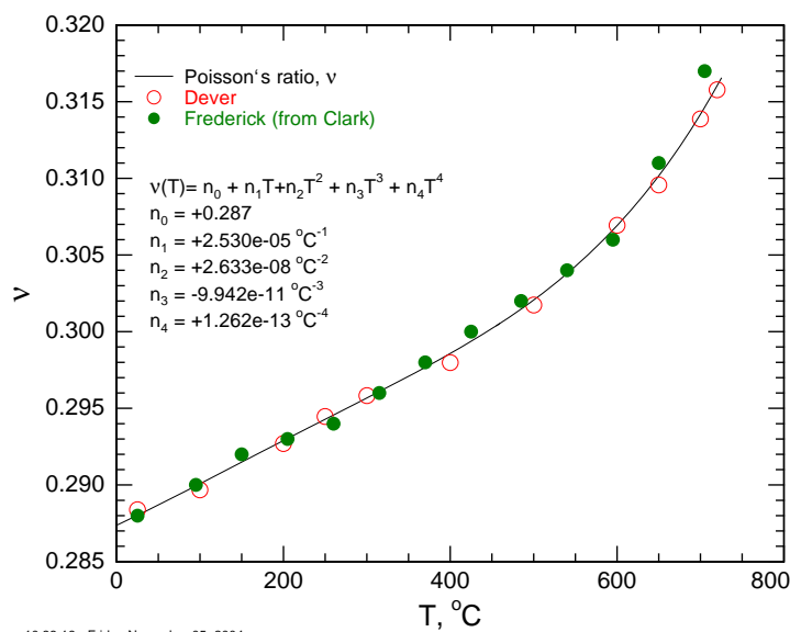
Figure 2–3. Poisson's ratio ( \nu ) as a function of temperature. The solid line is the fit of a 4th order polynomial (Eq. 2–3) for 0^\circ\text{C} < T < 725^\circ\text{C} .
