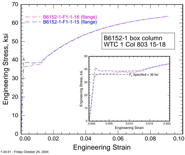
Figure A-24. Stress-strain curves for core box column B6152-1.
