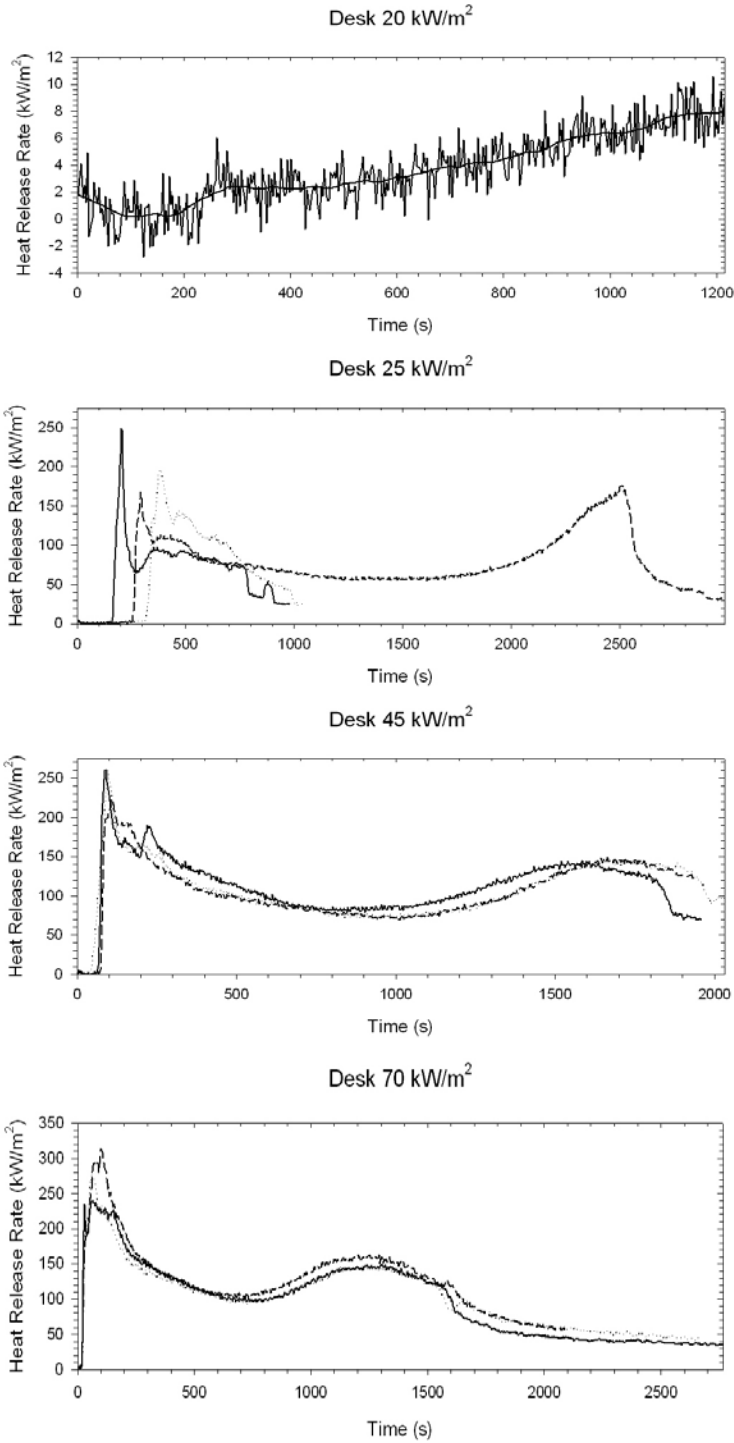
Figure A-1. Workstation desk surface heat release rate vs. time.
