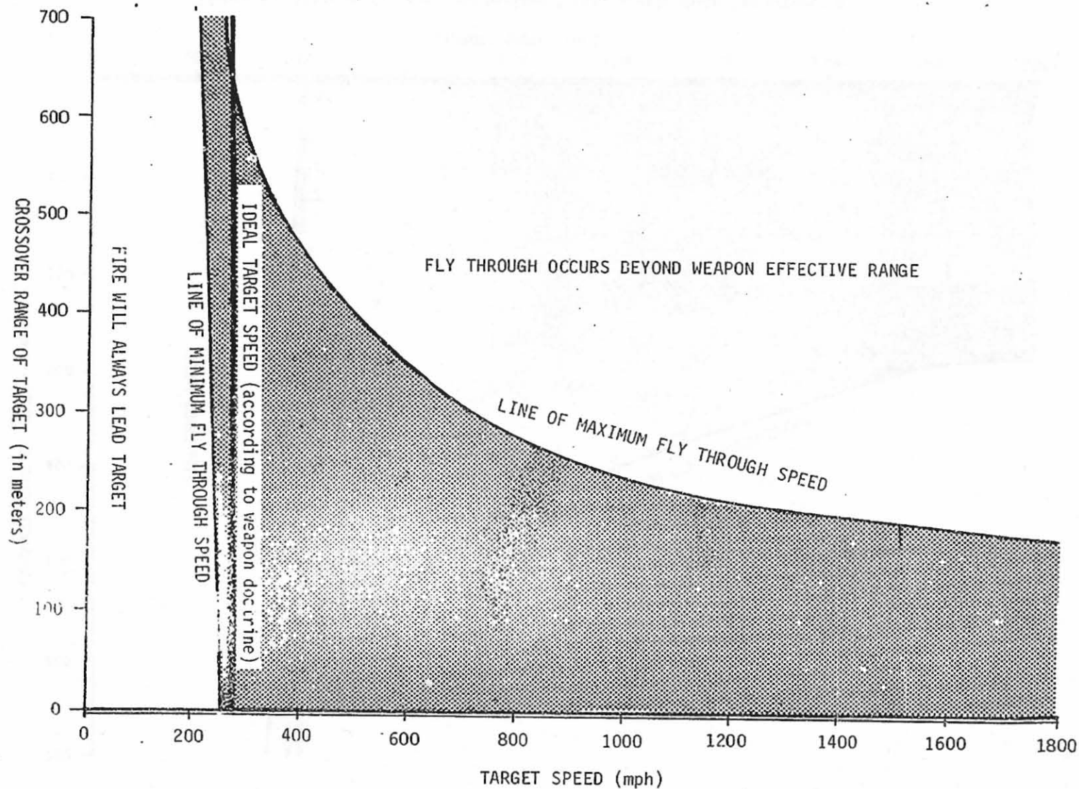
Figure 3. Minimum, Optimum, and Maximum Target Speeds Which Can Produce a Fly Through on the 200 Speed Ring as a Function of Target Range.
