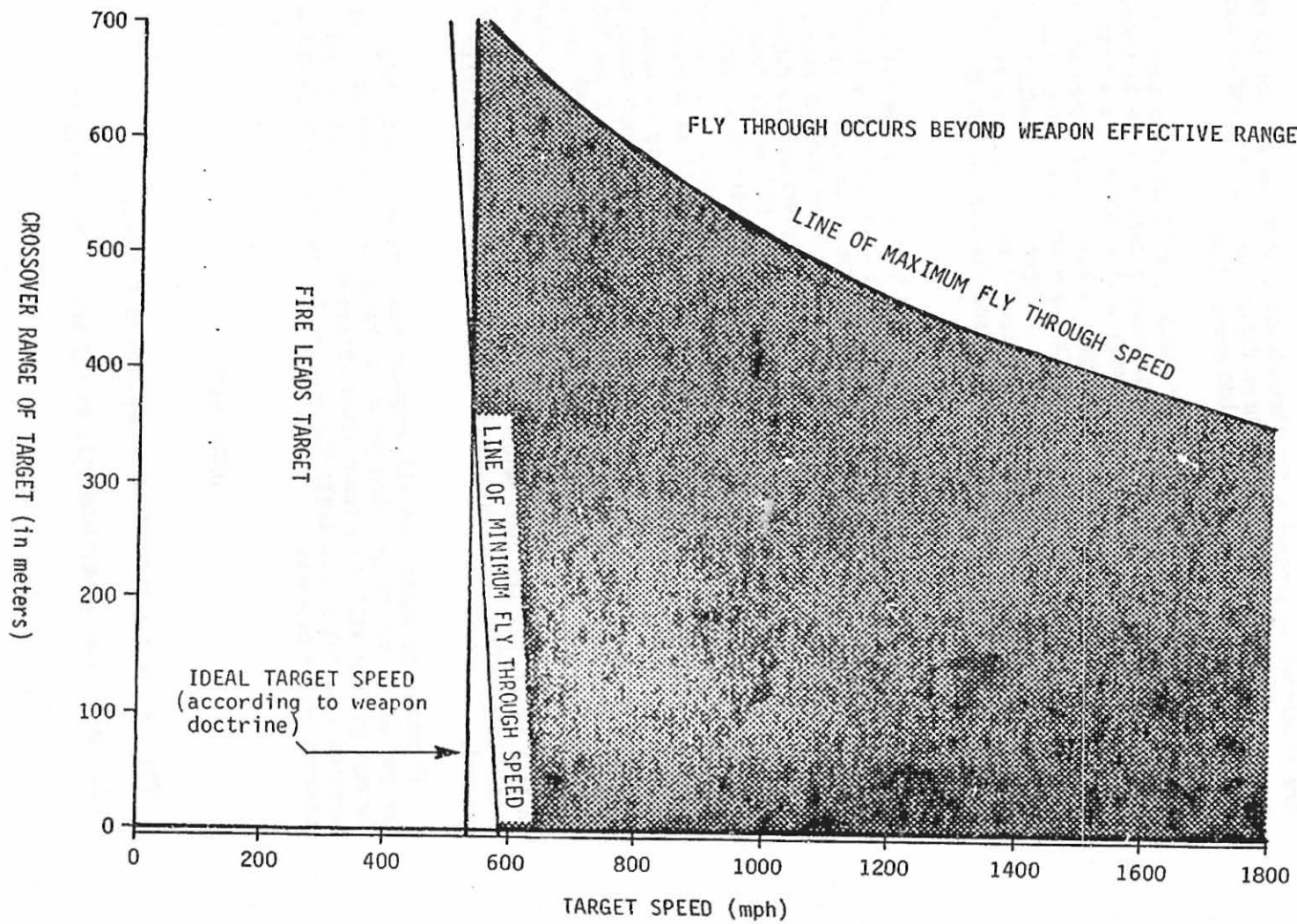
Figure 5. Minimum, Optimum, and Maximum Target Speeds Which Can Produce a Fly Through on the 400 Speed Ring as a Function of Target Range.
