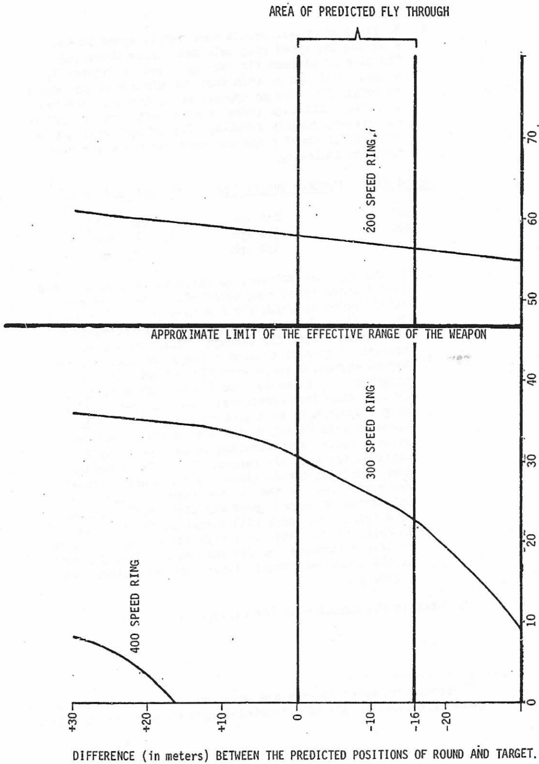
Figure 6. Predicted Results in Tracking a 460mph Target With the 200, 300, and 400 Speed Rings.
