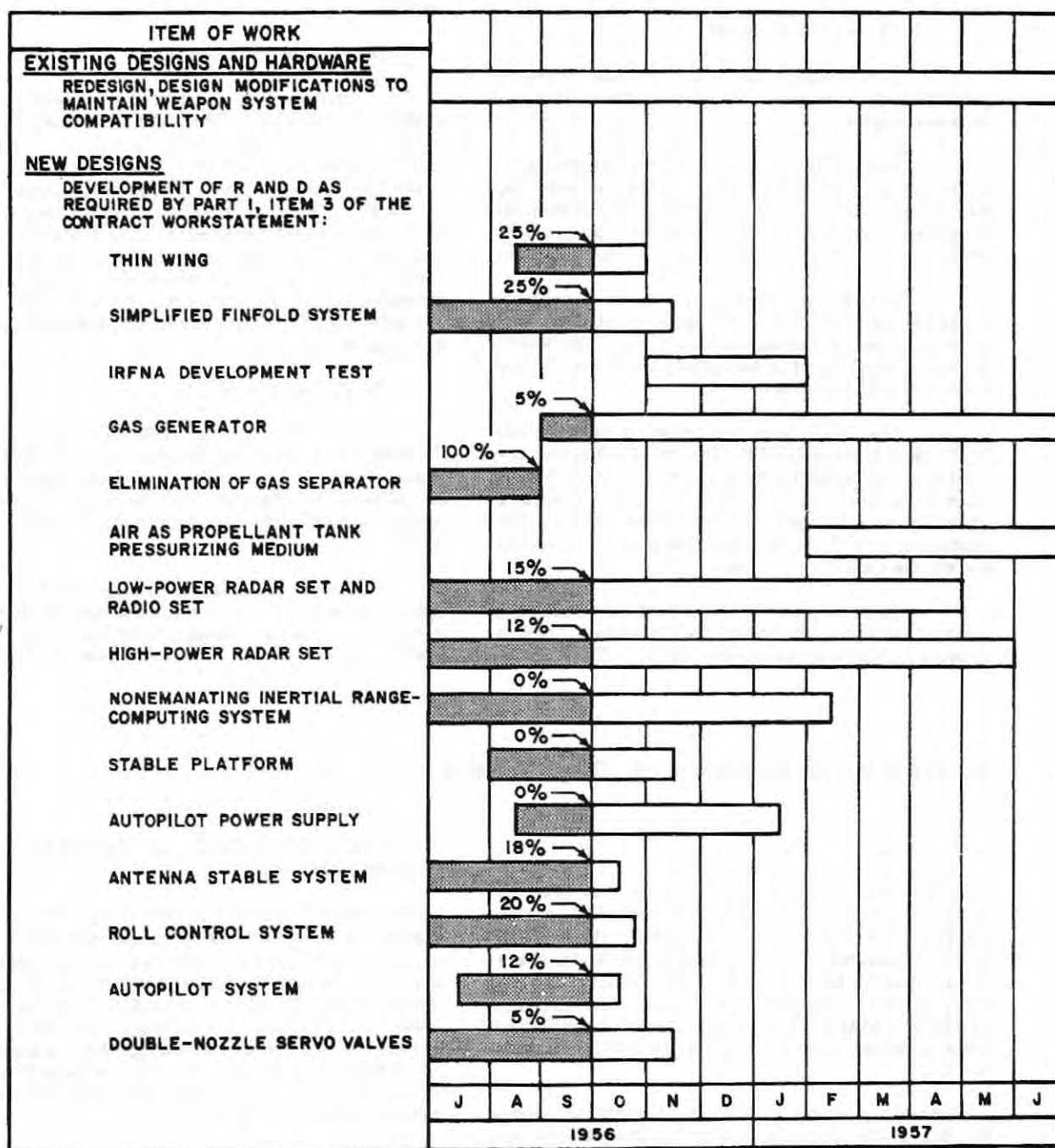
Figure 20. Ground Support Equipment Improvements
