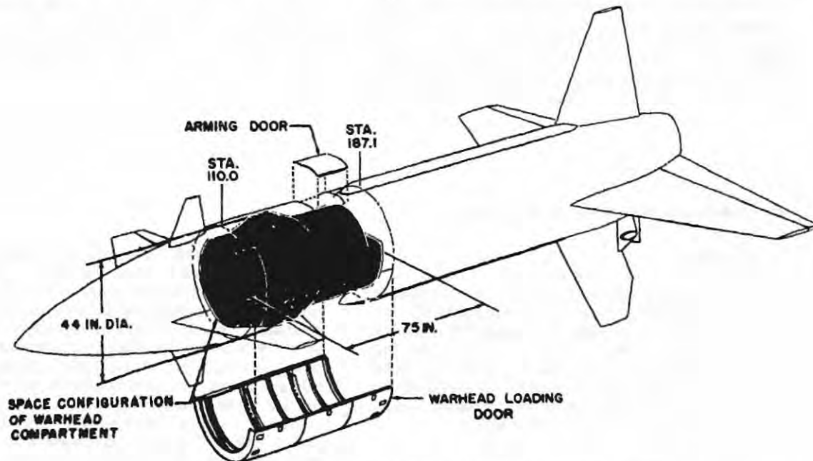
Figure 15. Configuration of GAM-63 Warhead Compartment
