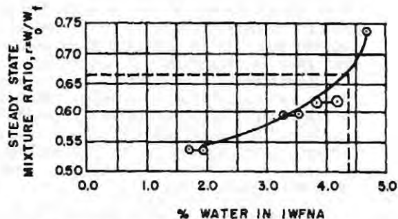
Figure 10. Limit of Steady State Operation at -33°F with Gas Generator HGP-81
