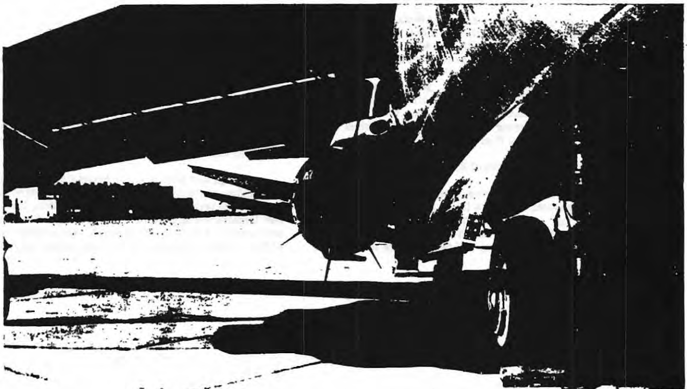
Figure 16. Rascal Missile Attached to DB-47 Director Aircraft
