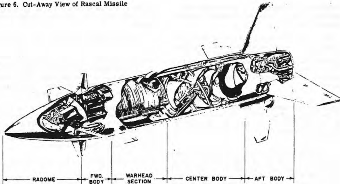
Figure 7. Structural Components of Rascal Missile
