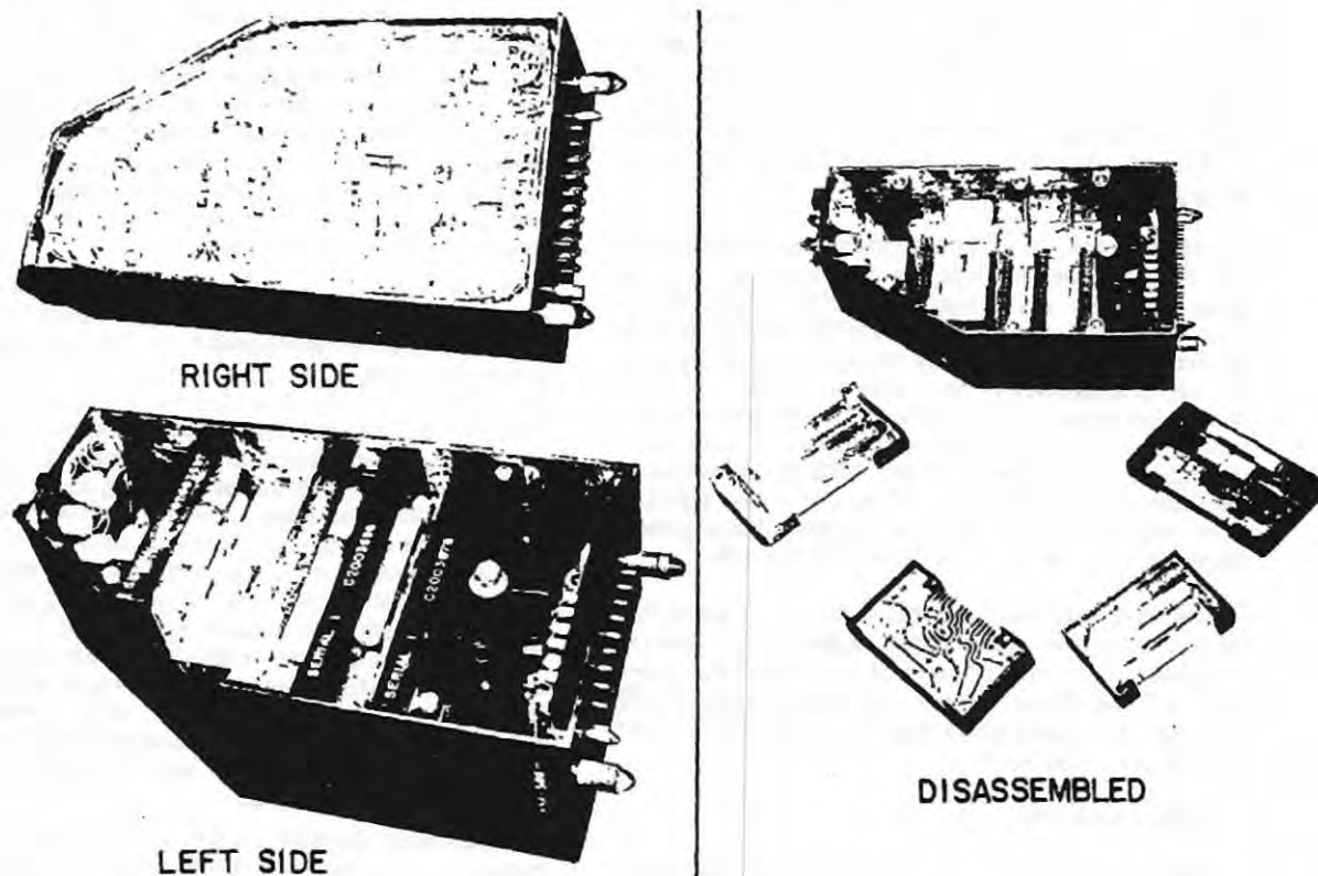
Figure 14. Repackaged Pitch Amplifier
