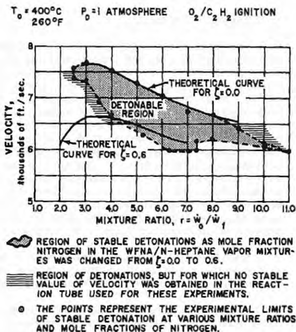
Figure 12. Detonability Region For WFNA/n - Heptane/Nitrogen Vapor Mixtures
