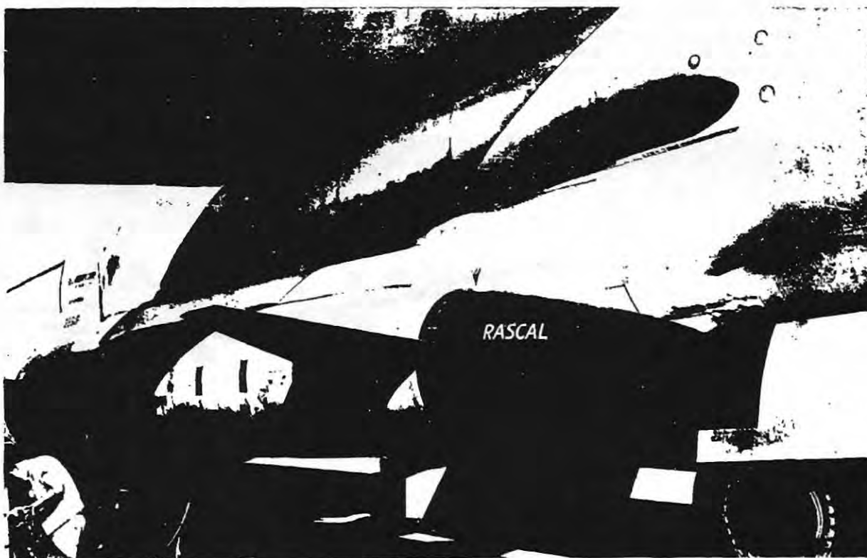
Figure 4. Dye Pattern on DB-47 after Testing New Gutter Drain
