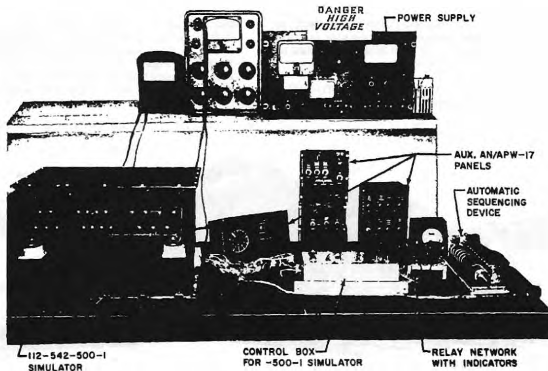
Figure 17. Setup for Life Testing GAM-63 Group Simulator
