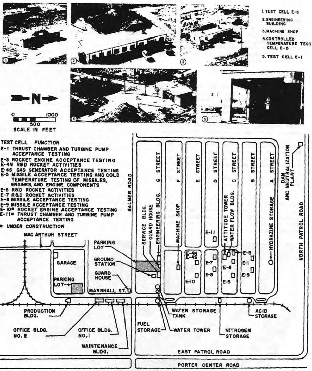
Figure 25. Plan View and Typical Installations at AF Plant No. 38
