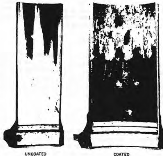
Figure 8. Comparison of Erosion in Coated and Uncoated Thrust Chambers
