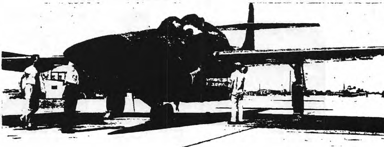
Figure 19. Preflight Preparation of JF-89 Research Airplane
