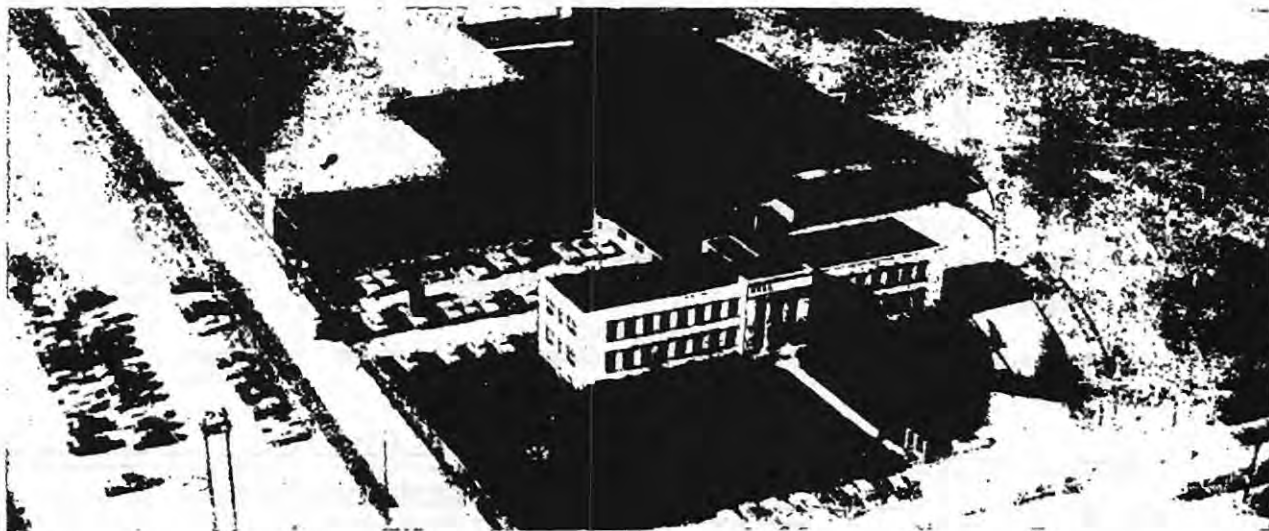
Figure 26. Contractor - Operated Logistics Depot, AF Plant No. 40
