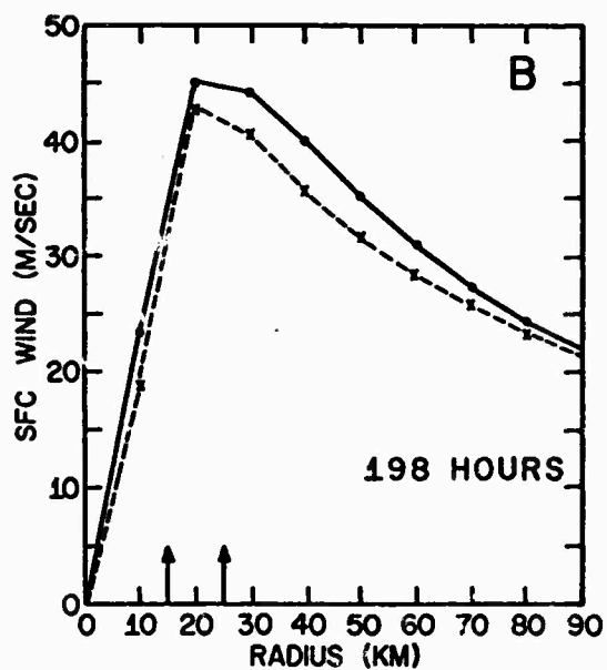
Figure C-22. Comparison of surface wind profiles for Experiment M7 (solid), and the control experiment (dashed), as a function of time. Arrows indicate grid points at which enhanced heating was applied.
