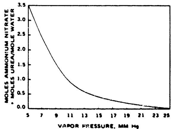
FIG. C-5. Vapor Pressure of Ammonium Nitrate/Urea/Water Solutions at Temperatures Near 26°C.
