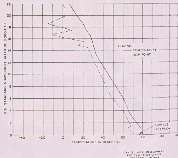
Fig. 8 Radiosonde Observation, Silver Hill, Washington, D. C., 2200 EST, August 15, 1952
