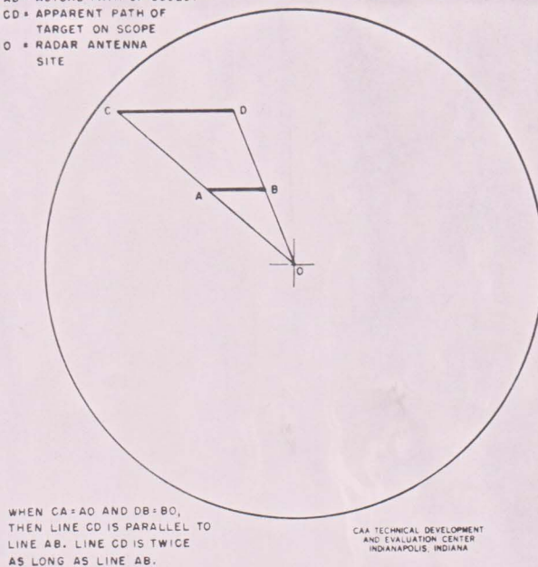
Fig. 13 Plan View of Reflection Effect
