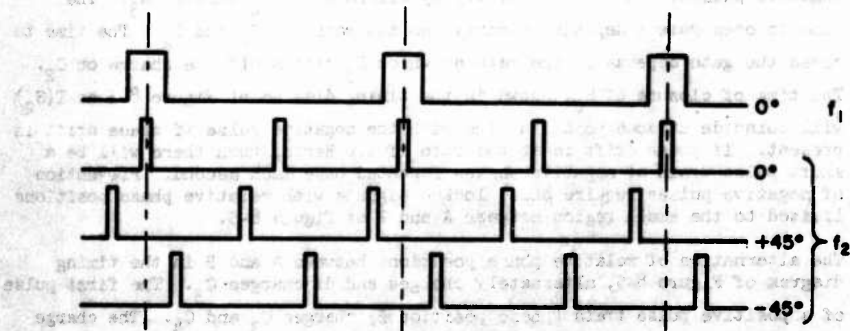
Figure 8-3. Phase-Shift Timing Diagram
