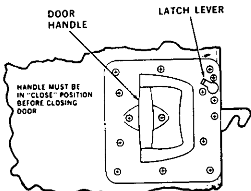
CABIN DOOR INTERIOR RELEASE HANDLE VIEW LOOKING OUTBOARD LEFT SIDE (SAME FOR RIGHT SIDE)
