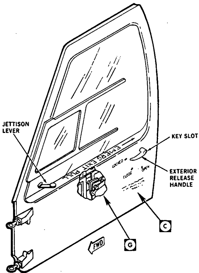
COCKPIT DOOR INTERIOR JETTISON LEVER VIEW LOOKING INBOARD LEFT SIDE (SAME FOR RIGHT SIDE)
