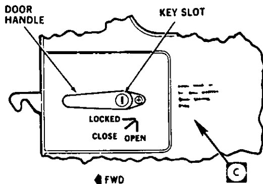
CABIN DOOR EXTERIOR RELEASE HANDLE VIEW LOOKING INBOARD LEFT SIDE (SAME FOR RIGHT SIDE)
