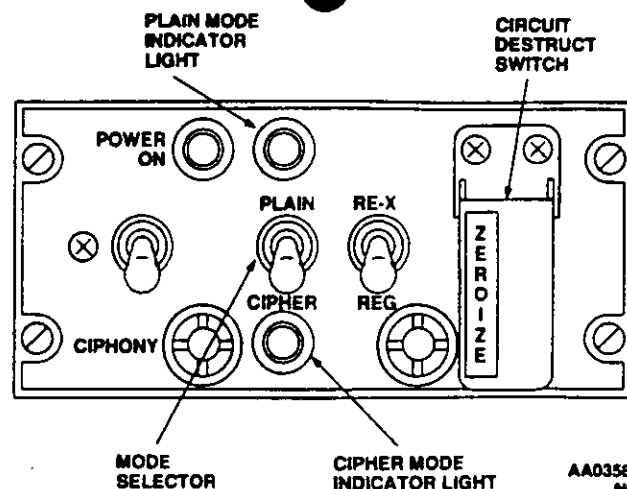
Figure 3-7. Voice Security System Control C-8157/ARC
