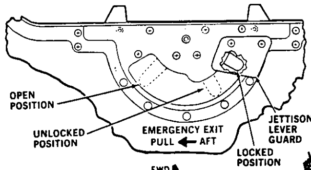
CABIN DOOR WINDOW JETTISON LEVER VIEW LOOKING OUTBOARD LEFT SIDE (RIGHT SIDE PULL → FWD)
