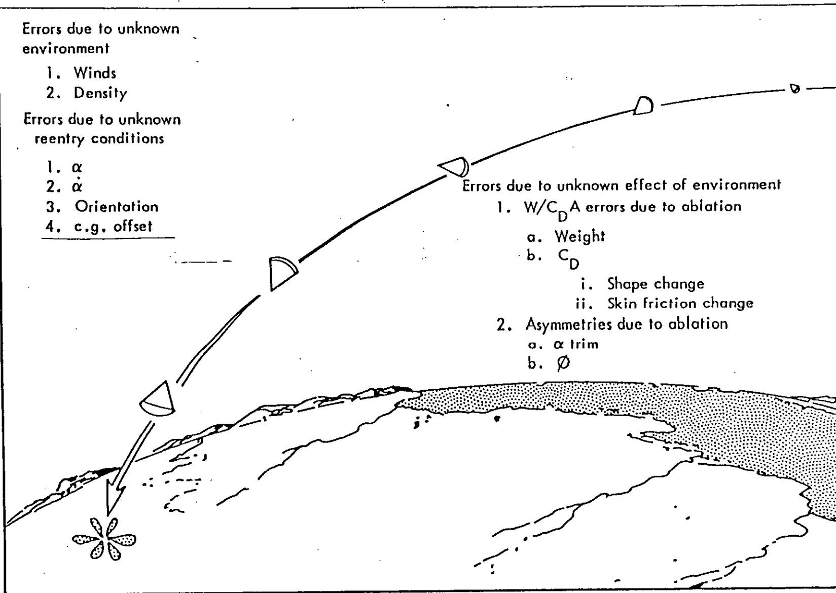
FIGURE A-5 Description of Reentry Error Contributors
