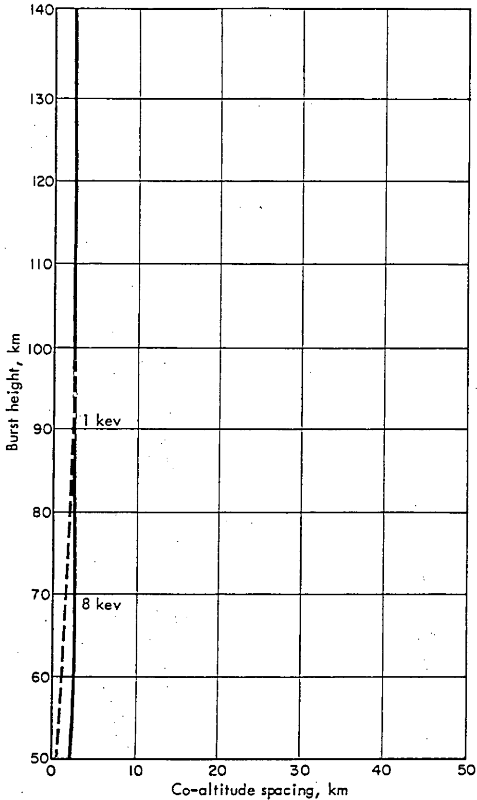
FIGURE A-29 Distance from 10-Mt Burst to 10,000 \text{ cal/cm}^2
