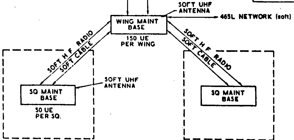
FIGURE 10 Wing Structure--Land Mobile System
