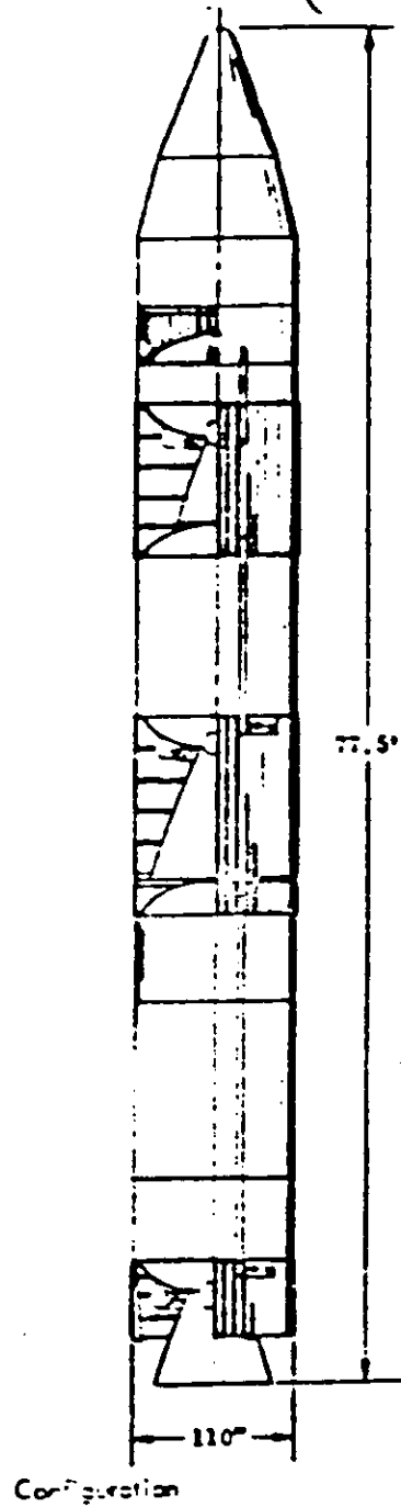
FIGURE 4 Land Mobile System Airborne Vehicle Configuration
