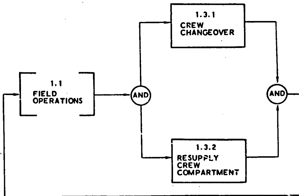
FIGURE 19 Second Level Operational Functional Flow Diagram (Block 1.3--Crew Change)
