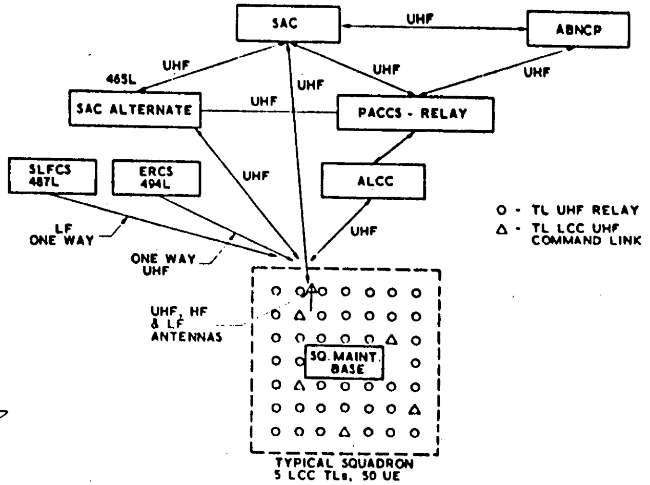
FIGURE 11 Command and Control System Summary
