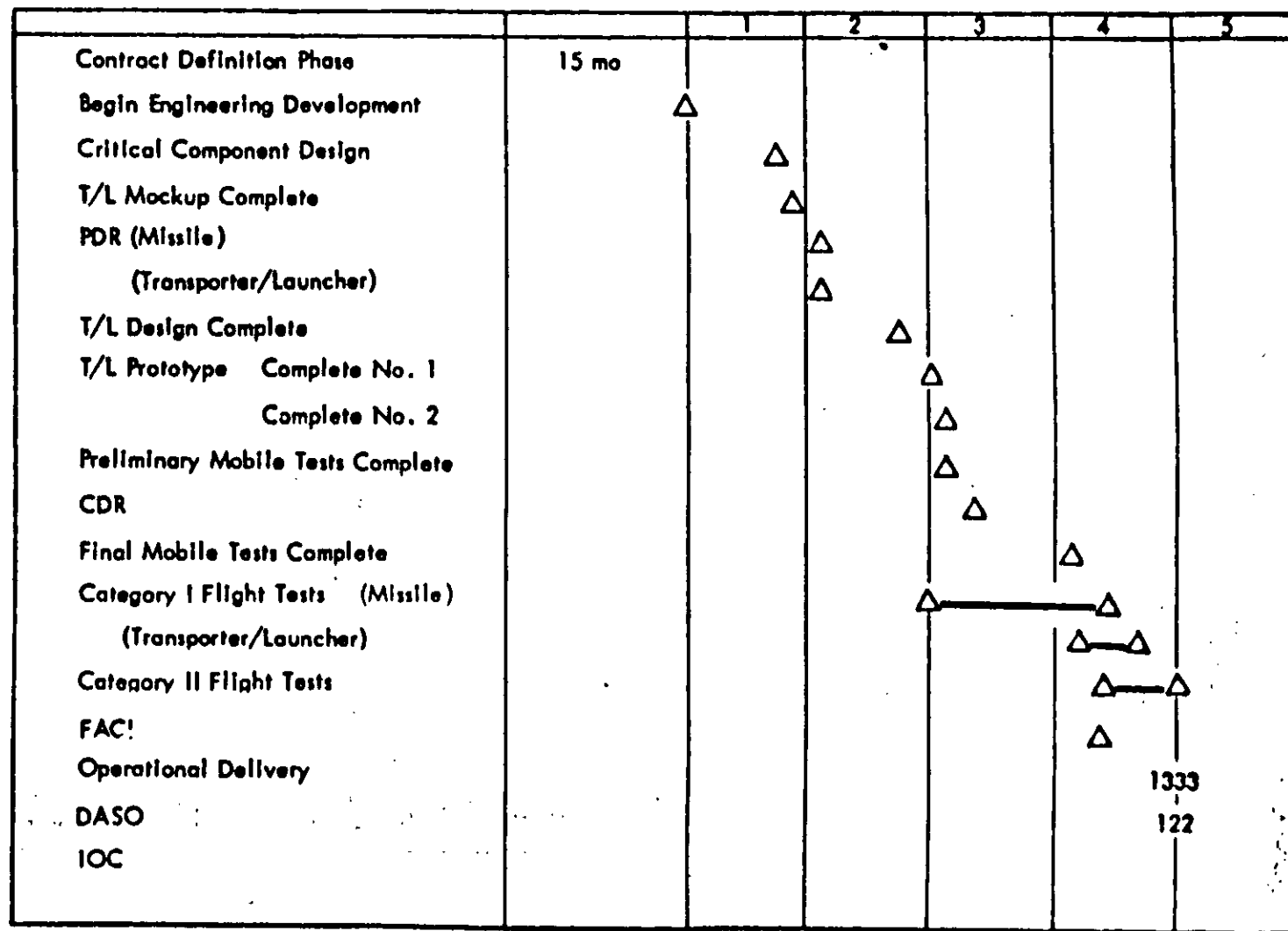
FIGURE 25 Land Mobile System Development Schedule
