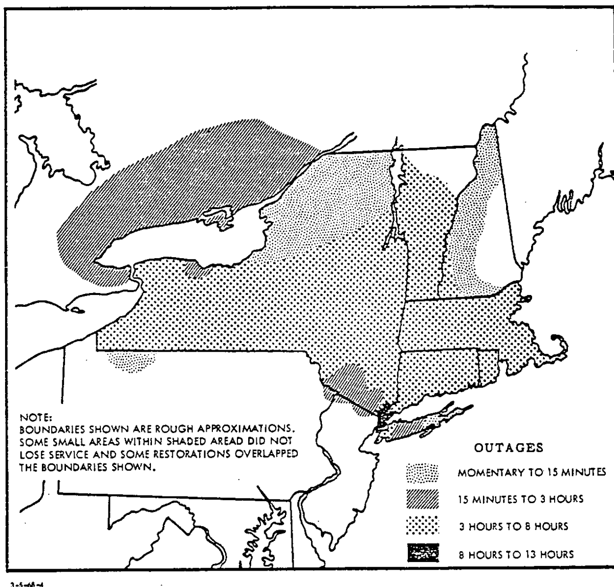
FIGURE 1 (U). Power Blackout in the Northeast, November 9, 1965, Generalized Areas of Outage (U)
