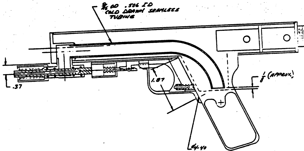
Fig. 3—Assembly Drawing of Feasibility Gun
