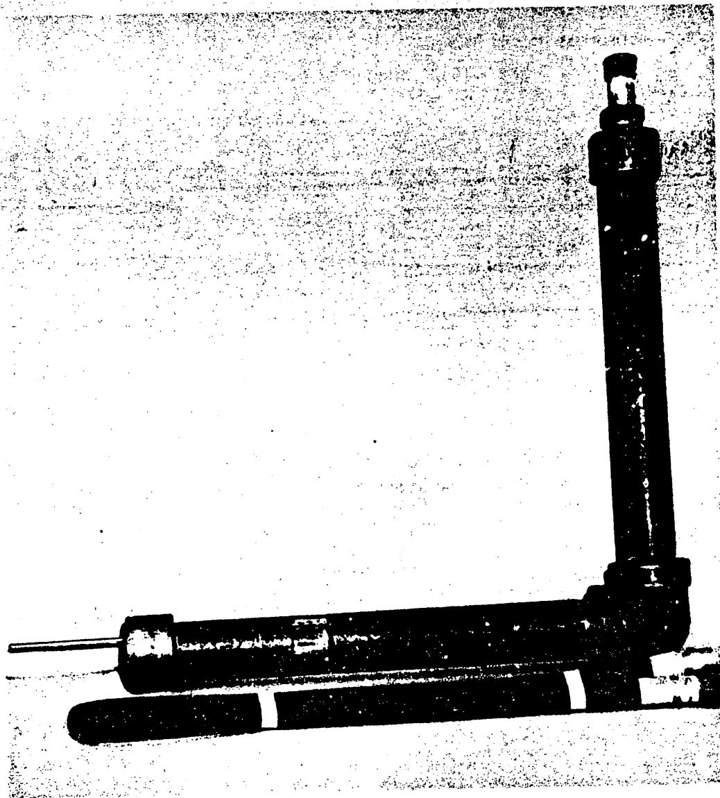
Fig. 7—Photograph of the Experimental Nozzle Apparatus
