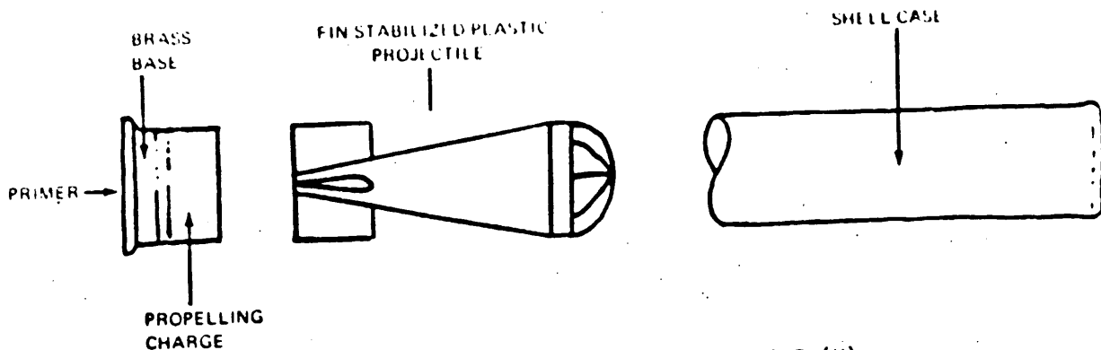
FIGURE 13. AAI SGA-100 BARRICADE PROJECTILE (U)
