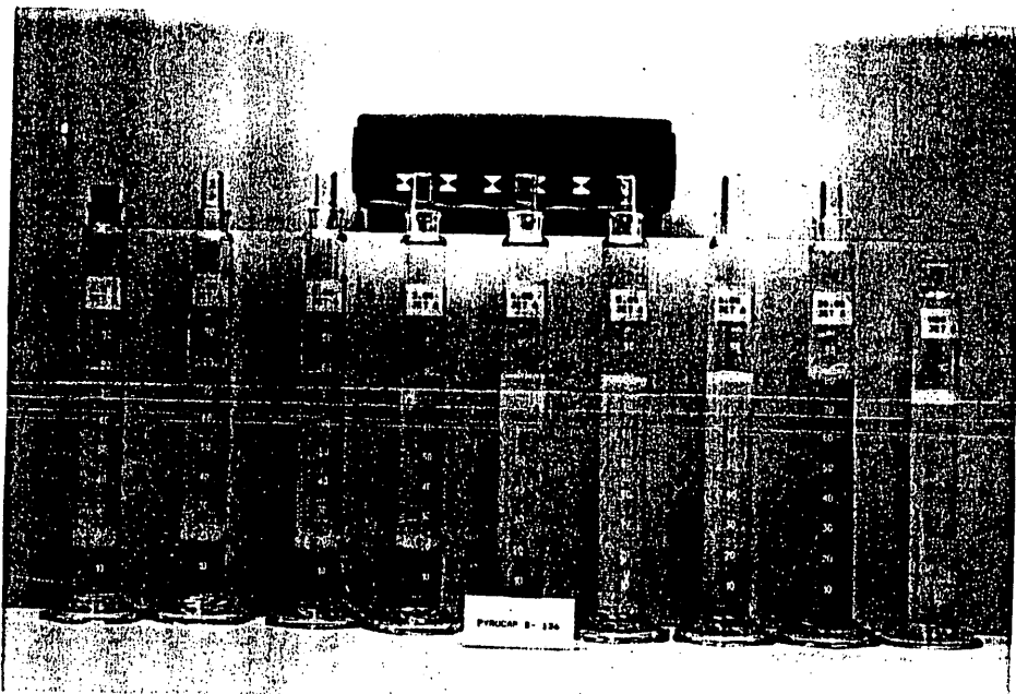
(b) Jet A and Pyrocap B-136 Solutions After Agitation
