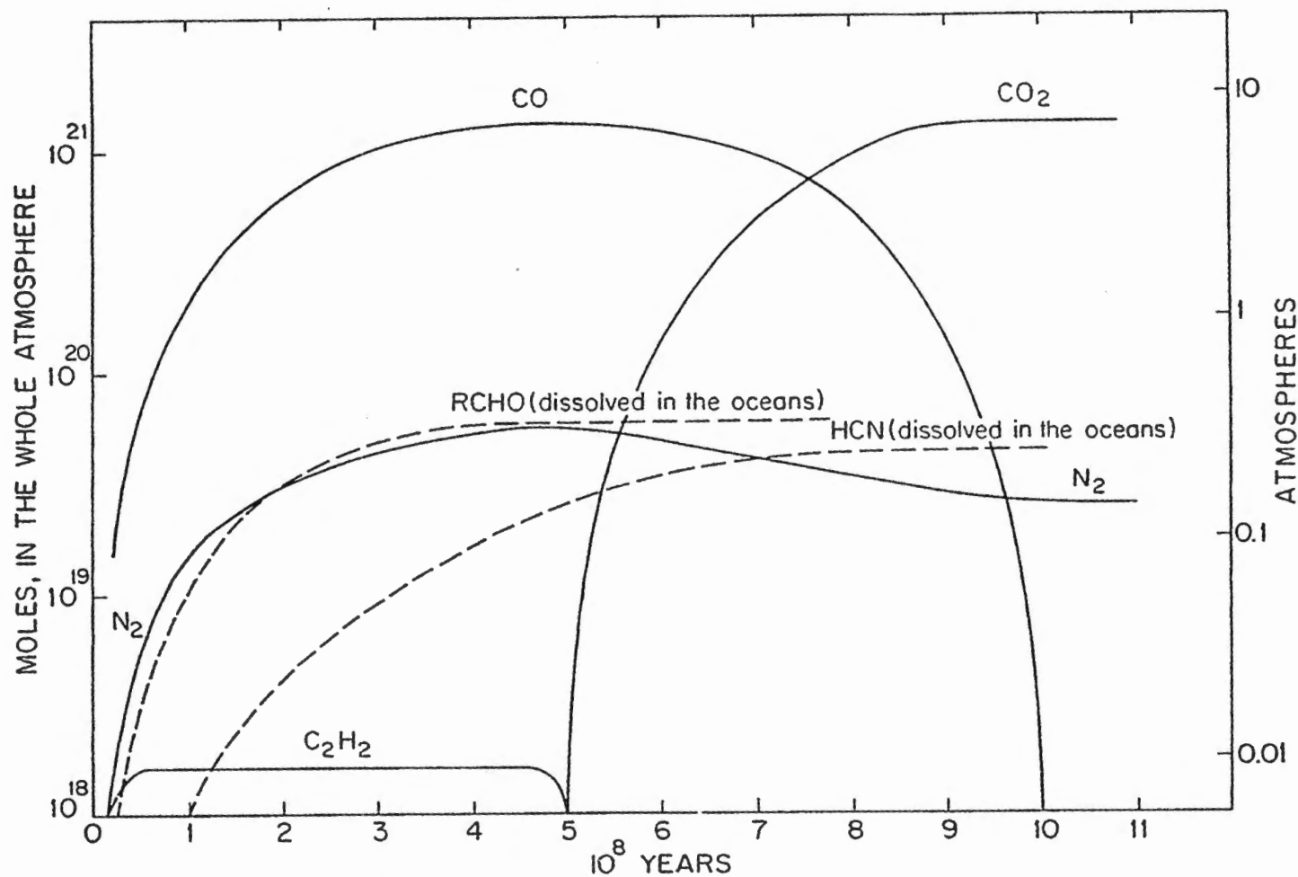
FIG. 7 VARIATION WITH TIME OF THE CONCENTRATION PROFILES OF THE MORE ABUNDANT SPECIES IN THE REDUCING ATMOSPHERE AS A RESULT OF THUNDER SHOCK WAVES, WHEN THE GREENHOUSE EFFECT OF ACETYLENE AND WATER VAPOUR WAS TAKEN INTO ACCOUNT. A STEADY RATE OF EXHALATION DURING 5 \times 10^6 /YR AND A SURFACE TEMPERATURE OF 60^\circ\text{C} WERE ASSUMED [AFTER (15)]
