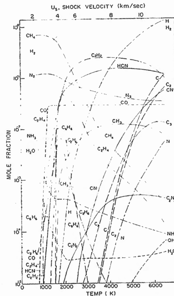
FIG. 4 EQUILIBRIUM SPECIES CONCENTRATIONS AS FUNCTIONS OF TEMPERATURE FOR A GAS MIXTURE CONSISTING OF 72% (BY VOLUME) CH_4 , 25% NH_3 AND 3% H_2O [AFTER (23)]
