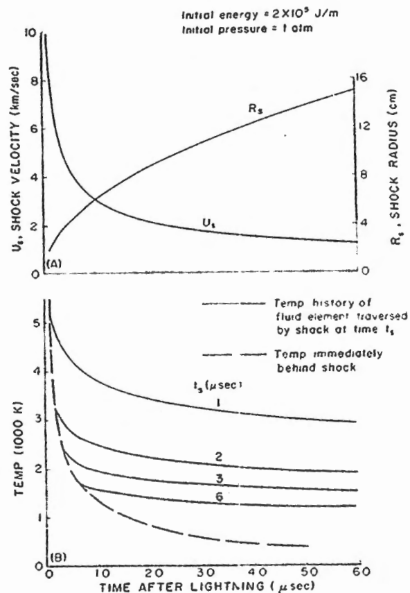
FIG. 3 APPROXIMATE DYNAMICAL BEHAVIOR OF A LIGHTNING-PRODUCED SHOCK WAVE: (A) VARIATION OF SHOCK-WAVE VELOCITY AND RADIUS WITH TIME. (B) TEMPERATURE HISTORIES IMMEDIATELY BEHIND SHOCK-WAVE AND OF FLUID ELEMENT OF FLUID [AFTER (23)]
