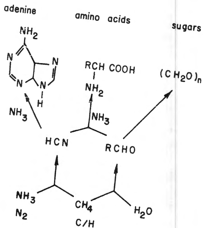
FIG. 6 A SCHEME OF CHEMICAL EVOLUTION OF BIOMONOMERS
