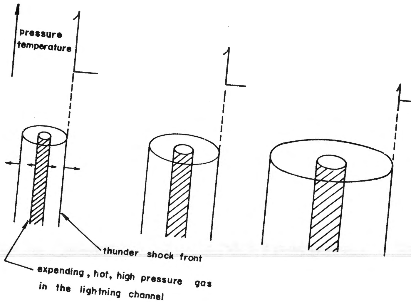
FIG. 2 A SCHEMATIC DRAWING OF A CYLINDRICAL THUNDER SHOCK WAVE
