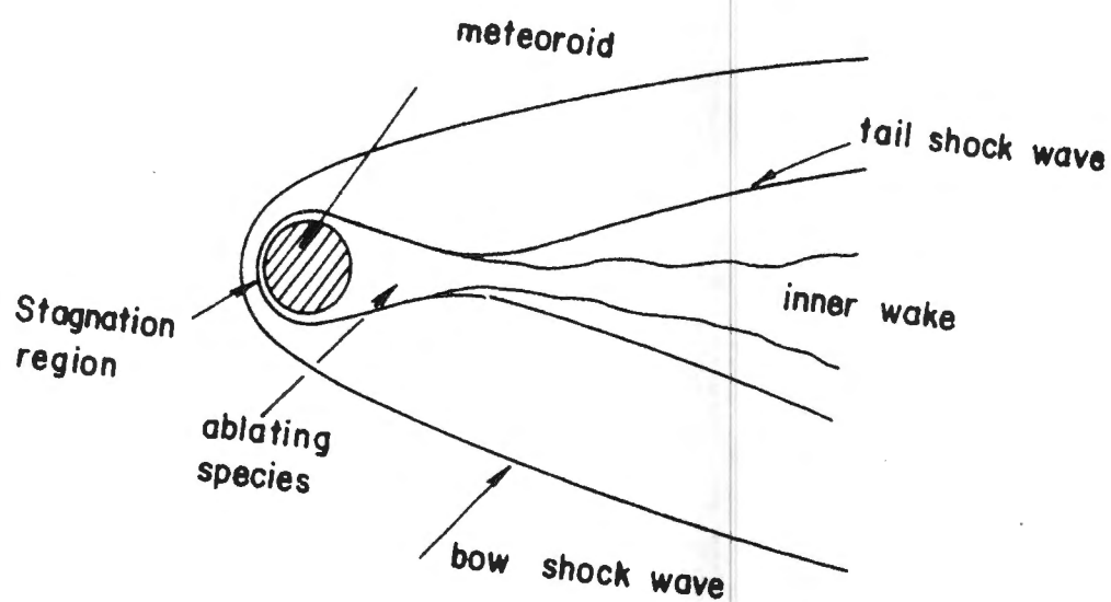
FIG. 5 SHOCK-WAVES GENERATED BY METEORITES [A. DE (2)]
