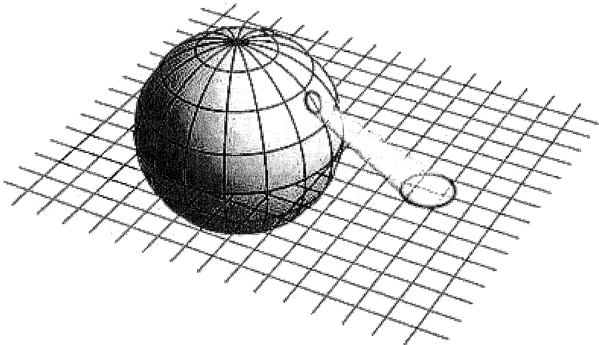
Figure 19. Stereographic Projection
