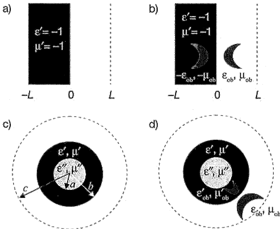
Figure 5. Complementary Media Invisibility Cloak: (a) The slab of empty space x with 0 < x < L is optically canceled by a slab of negative-index material in -L < x < 0 . (b) The same cancellation effect works with an object in 0 < x < L if the negative-index slab contains an antioject. (c) A spherical shell b < r < c is optically canceled by a negative-index shell a < r < b . If the core r < a is optically equivalent to a sphere of radius c , then this device is invisible. (d) The same as (c), but with an object in the canceled shell b < r < c . The object is cloaked: both it and the cloaking sphere are invisible.
