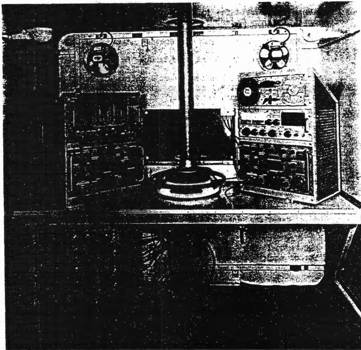
First Generation GRAB/Dyno 1 Receiving, Timing, and Recording Position inside ESV Hut
