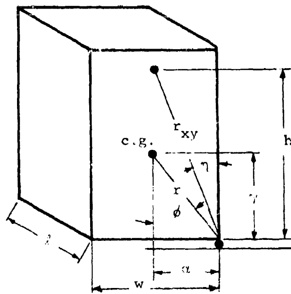
a) Geometry
