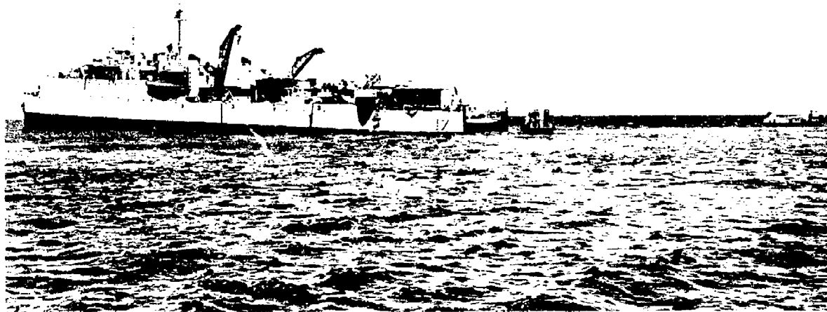
Figure 34. FLATHEAD device barge being removed from the well of USS Catamount (LSD-17), REDWING.
