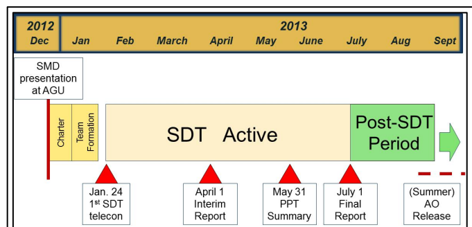
Figure 2-1. Timeline of Mars 2020 SDT Implementation Process. The process began in December 2012, with the announcement at the AGU conference that NASA would propose to fly a mission to Mars, based on the Curiosity rover design, in 2020. The SDT was formed in late January, and has completed its report on July 1, 2013, preparatory for the release of the AO for the Mars 2020 rover mission.
