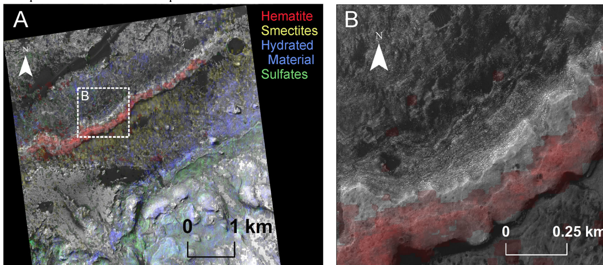
Figure 3-3. Connecting orbital data with rover-scale data improves the geologic interpretation. Mars Reconnaissance Orbiter of Mount Sharp strata planned for Curiosity rover traverse. Grayscale represents 30 cm/pixel HiRISE images, and color shows minerals from CRISM images. (A) Northwest flank of Mount Sharp, with elevation increasing from upper left to lower right. (B) Mineral occurrence and morphology at rover traverse scale enables planning of traverses and for possible contact measurements. From Fraeman et al (2013), submitted.
