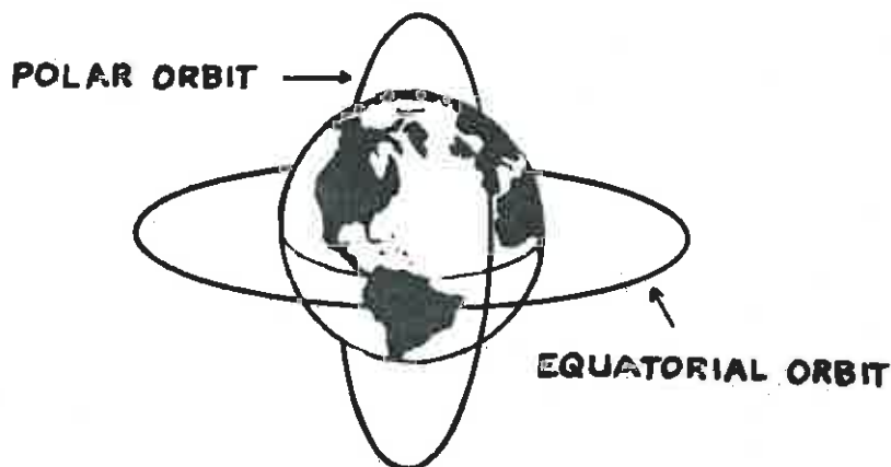
Figure 8. Satellite Orbits
