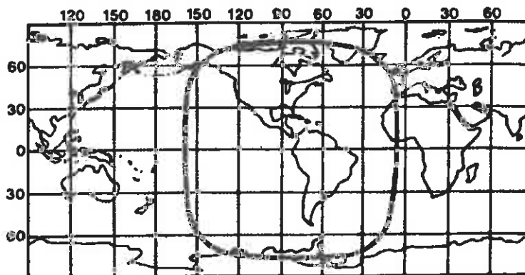
Figure 9. Maximum Earth Coverage of a Geostationary Satellite Located Over Panama 16
