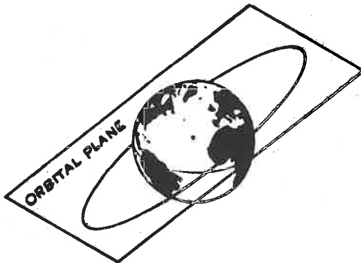
Figure 5. Orbital Plane
