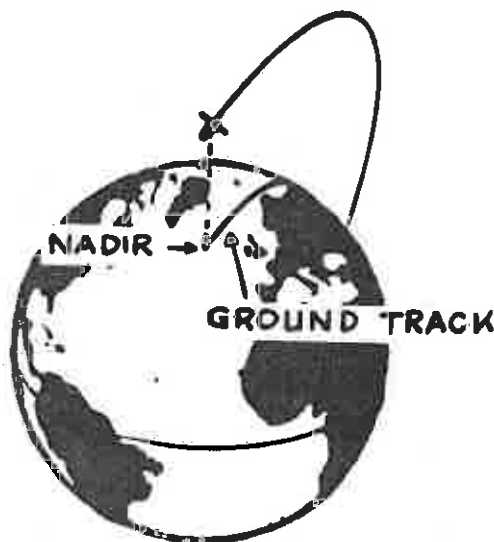
Figure 6. Satellite Ground Track
