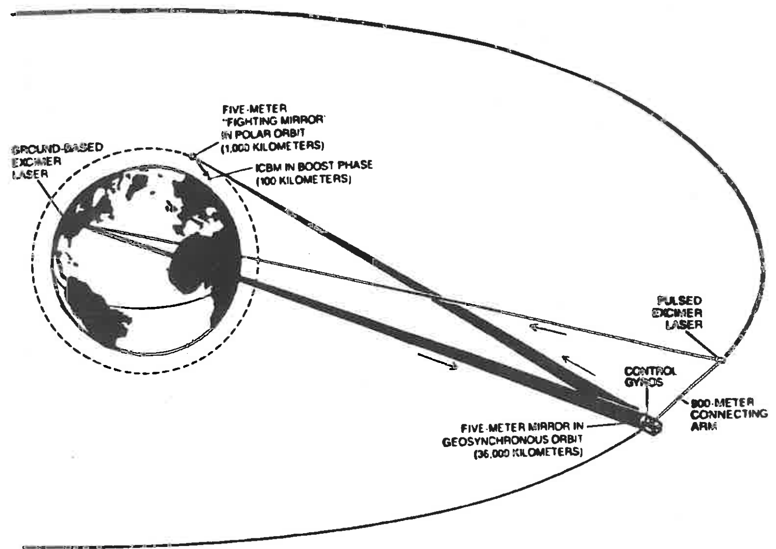
Figure 16. Ground-Based Laser BMD System
