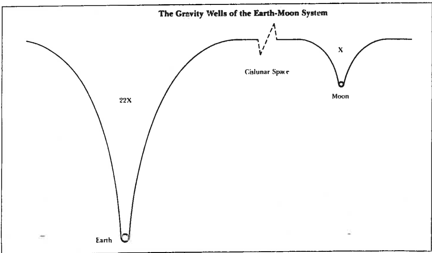
Figure 1. Gravity Wells
