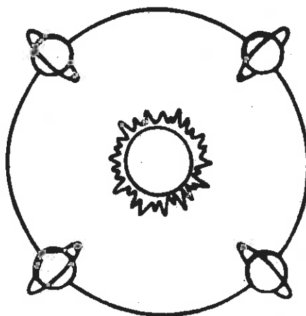
Figure 10. Annual Precession of Orbital Plane in a Sunsynchronous Orbit
