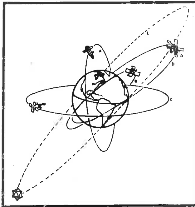
Figure 11. Military Space System Orbits 18
