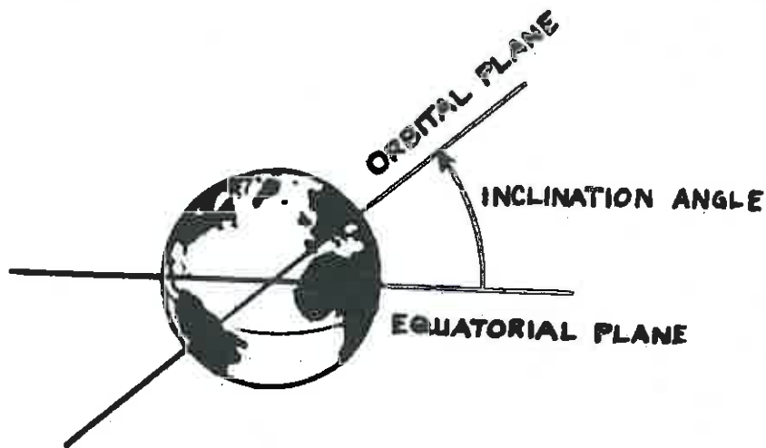
Figure 7. Inclination Angle
