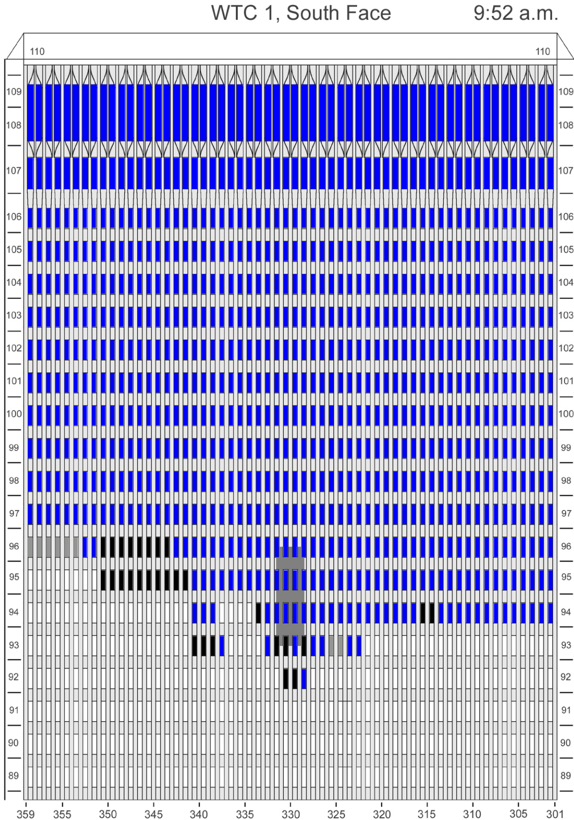
Figure E-34. Diagram of the south face of WTC 1 for floors 89 to 110 at 9:52 a.m. showing windows where smoke was observed and those that were hidden from view.
