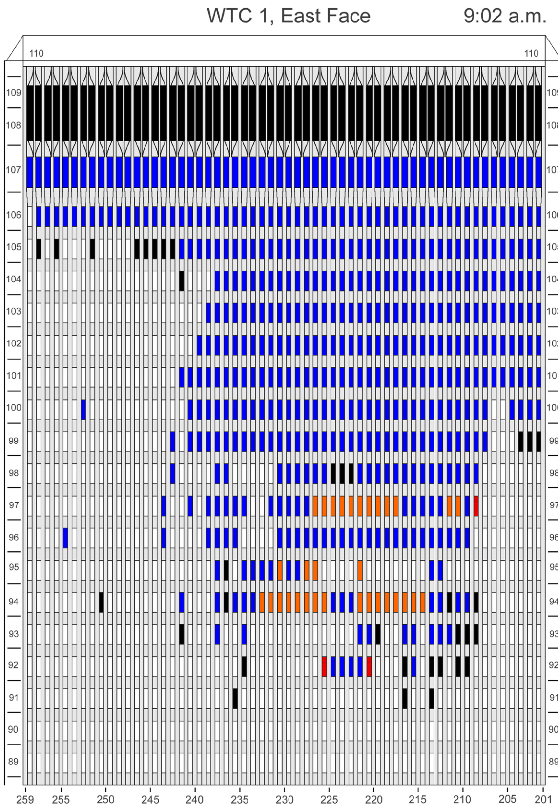
Figure D-11. Diagram of the east face of WTC 1 for floors 89 to 110 at 9:02 a.m. showing the condition of windows and locations of fires.
