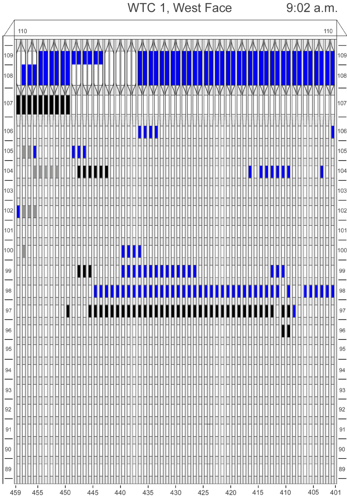
Figure F-18. Diagram of the west face of WTC 1 for floors 89 to 110 at 9:02 a.m. showing windows where smoke was observed and those that were hidden from view.
