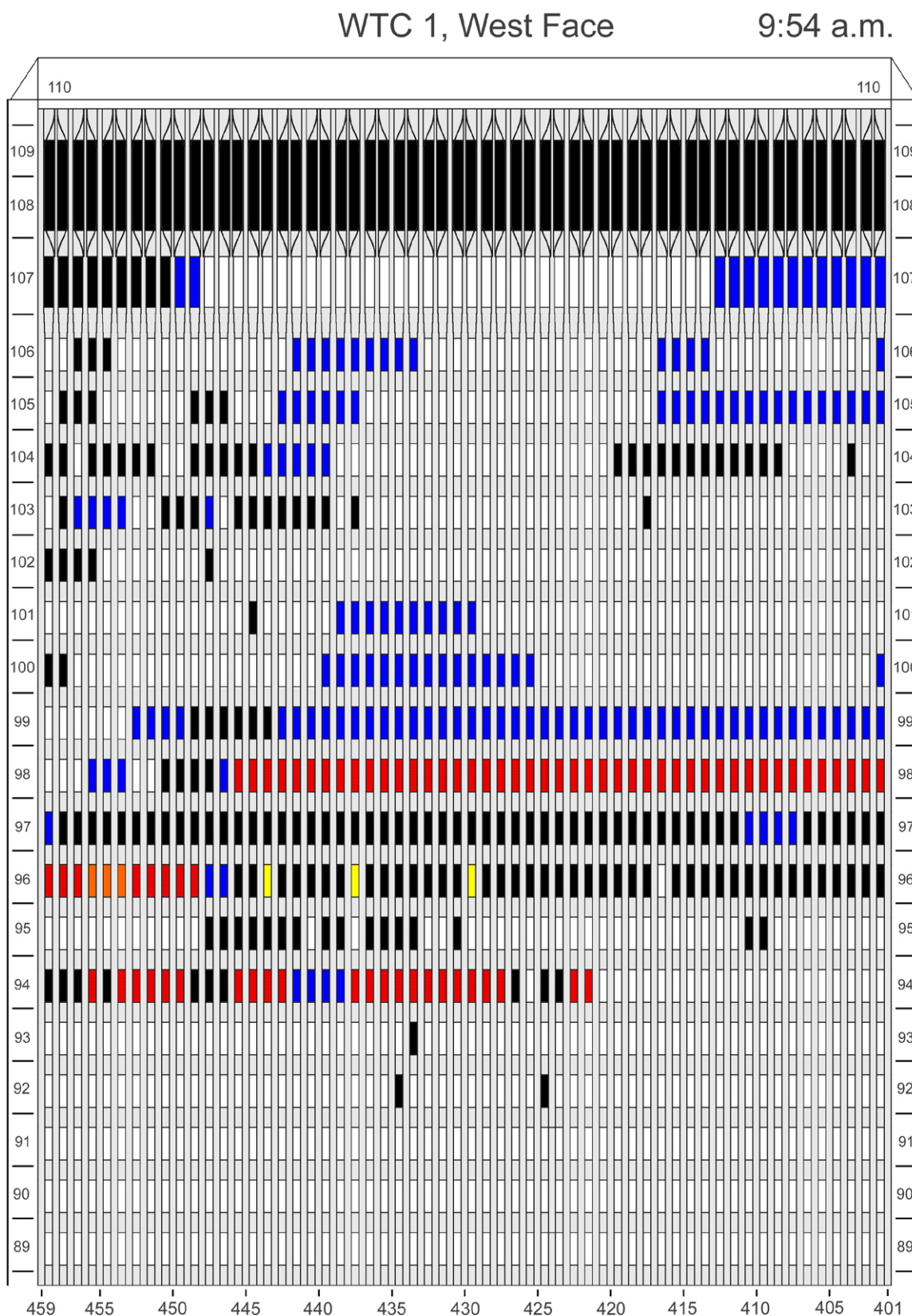
Figure F-47. Diagram of the west face of WTC 1 for floors 89 to 110 at 9:54 a.m. showing the condition of windows and locations of fires.
