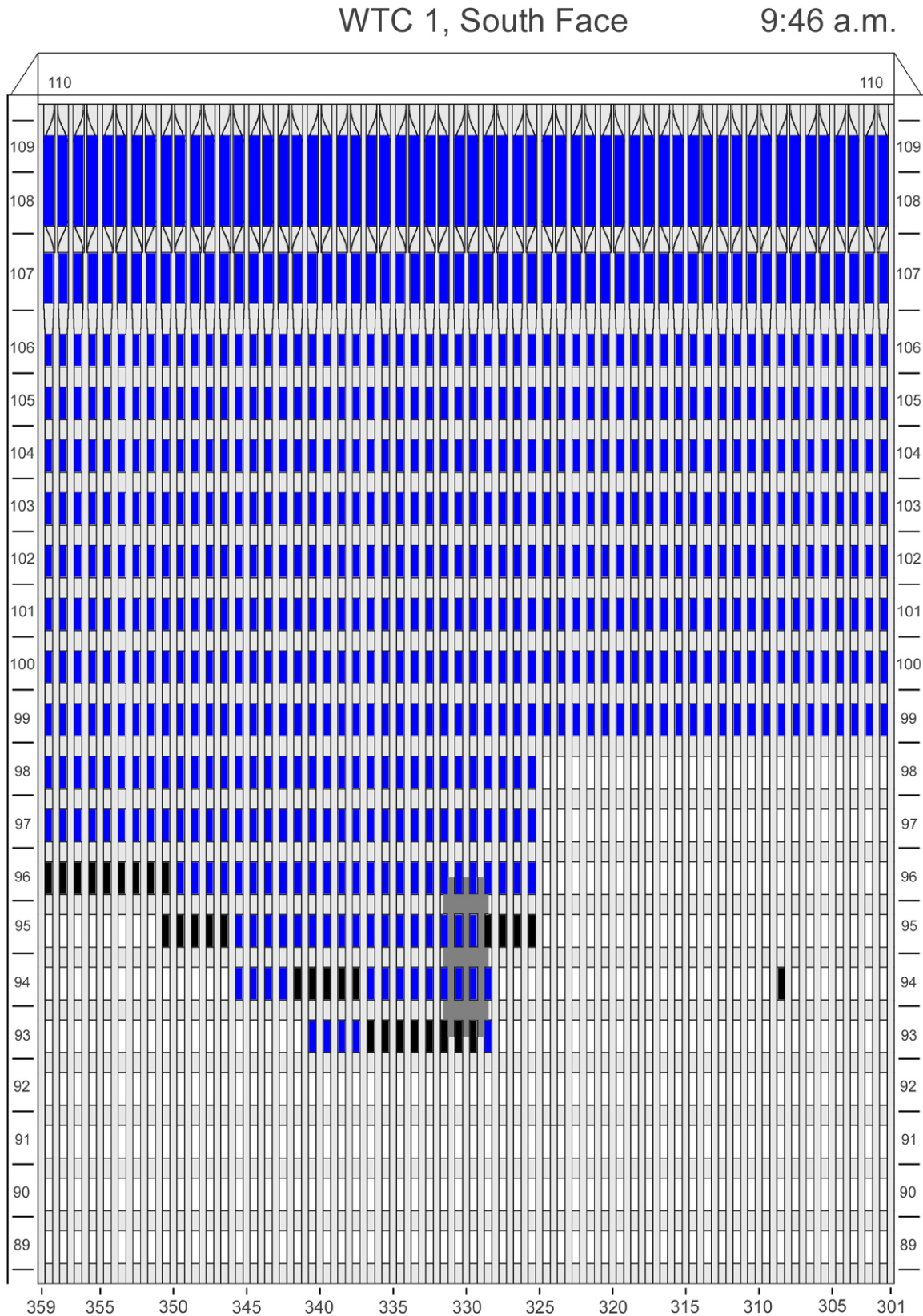
Figure E-32. Diagram of the south face of WTC 1 for floors 89 to 110 at 9:46 a.m. showing windows where smoke was observed and those that were hidden from view.
