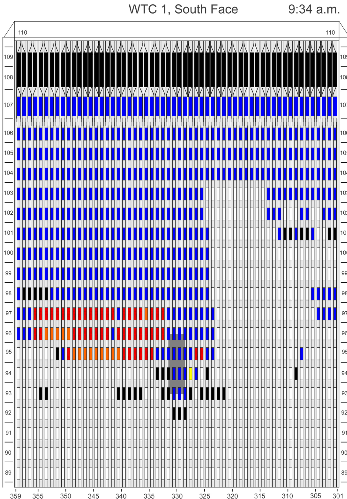
Figure E-23. Diagram of the south face of WTC 1 for floors 89 to 110 at 9:34 a.m. showing the condition of windows and locations of fires.
