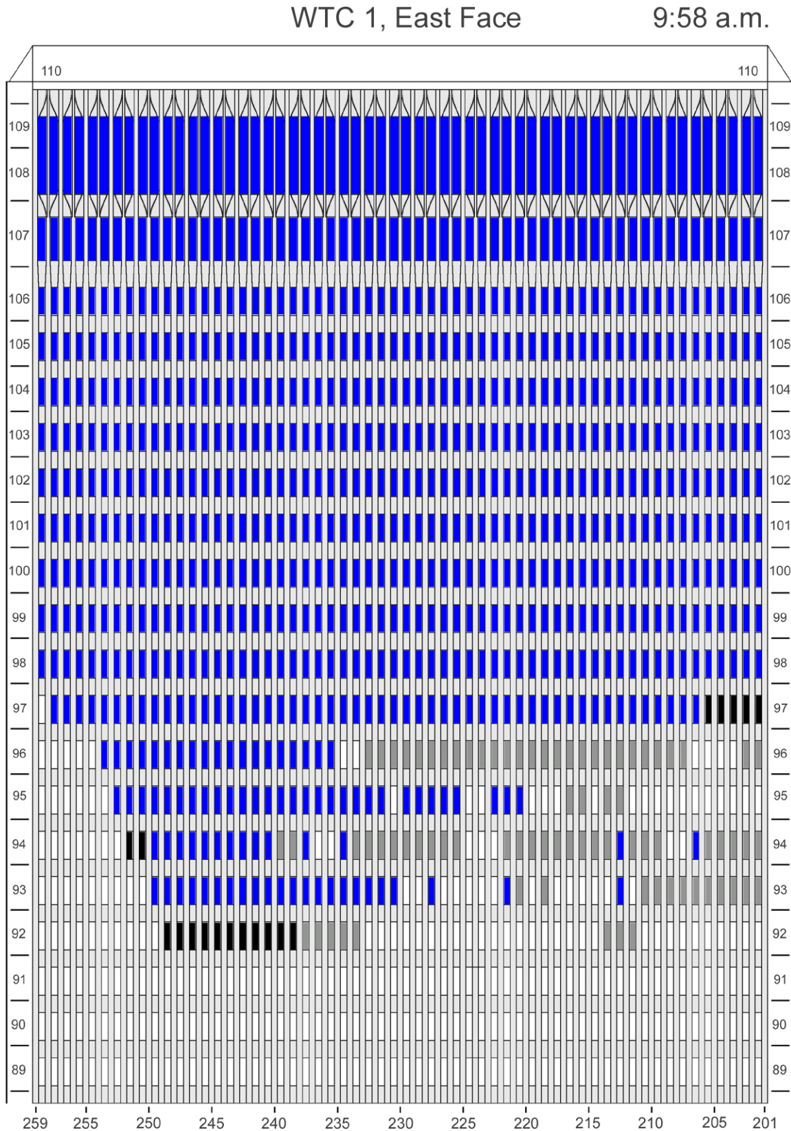
Figure D-38. Diagram of the east face of WTC 1 for floors 89 to 110 at 9:58 a.m. showing windows where smoke was observed and those that were hidden from view.
