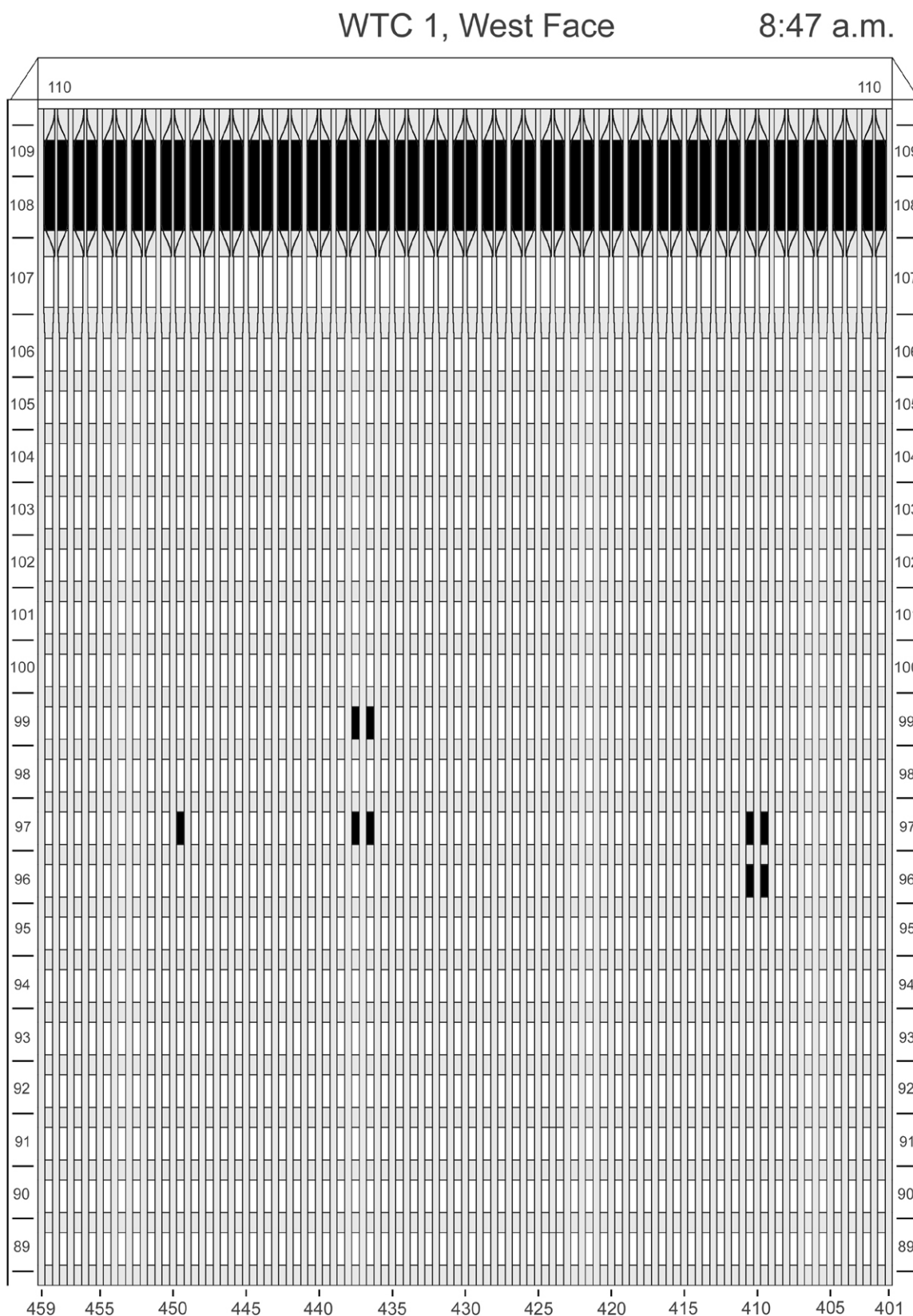
Figure F-1. Diagram of the west face of WTC 1 for floors 89 to 110 at 8:47 a.m. showing the condition of windows and locations of fires.
