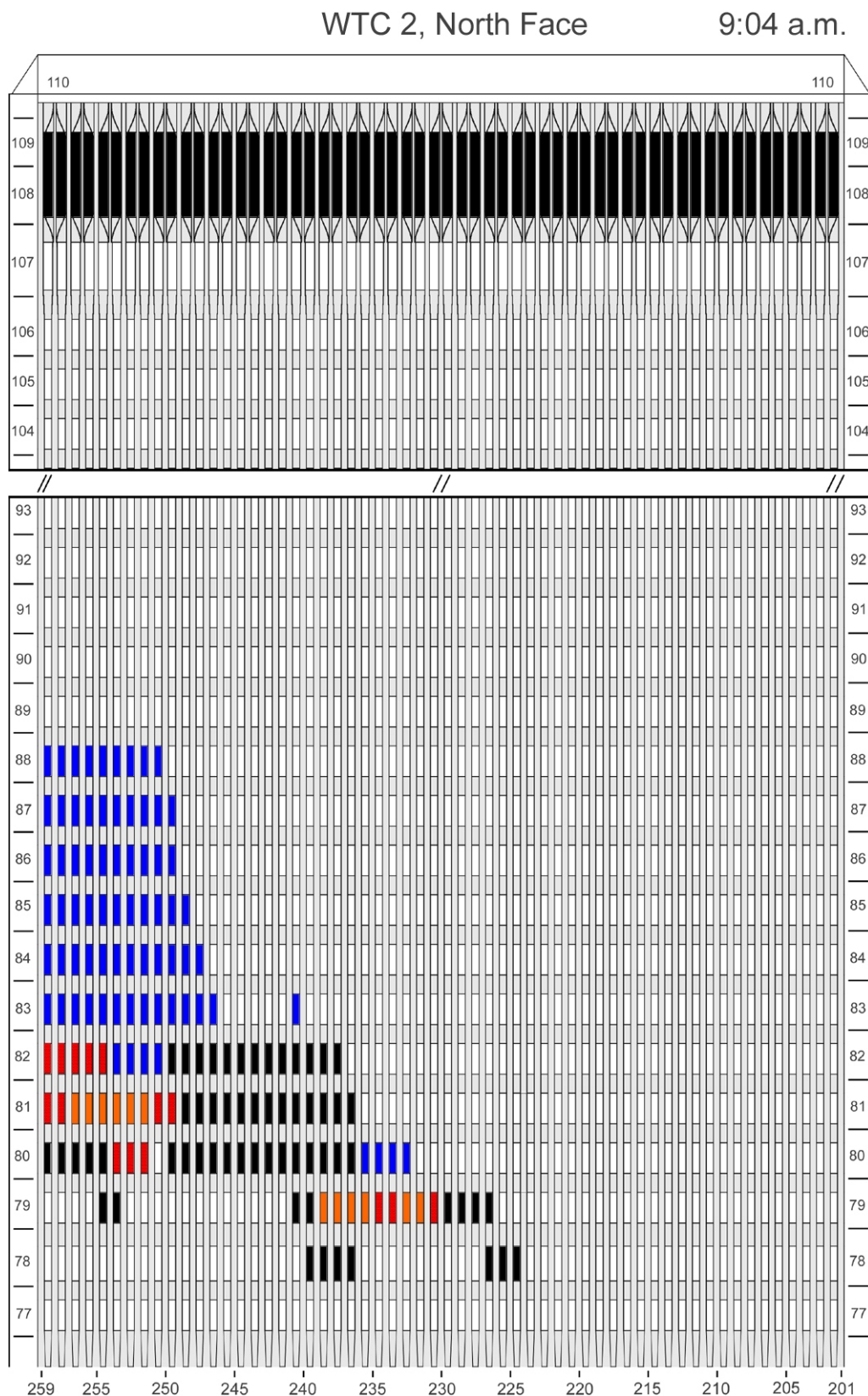
Figure G-3. Diagram of the north face of WTC 2 for floors 77 to 93 and floors 104 to 110 at 9:04 a.m. showing the condition of windows and locations of fires.
