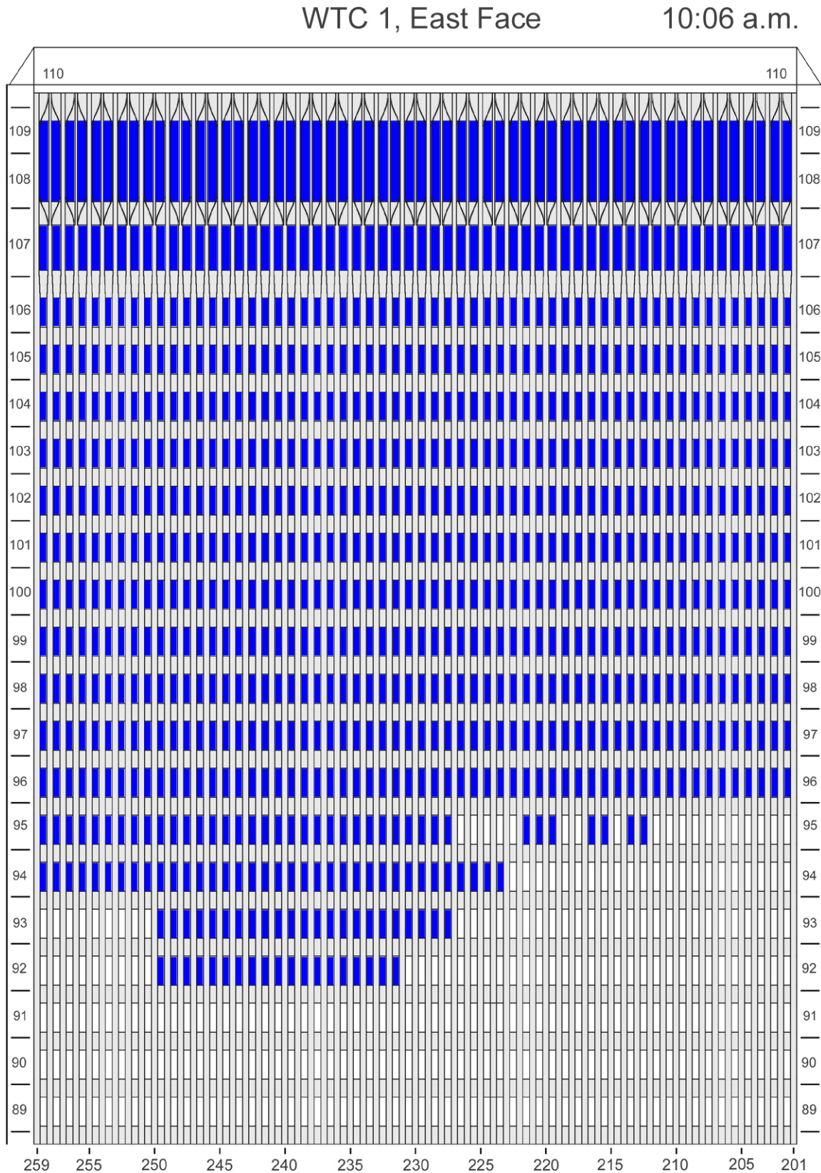
Figure D-42. Diagram of the east face of WTC 1 for floors 89 to 110 at 10:06 a.m. showing windows where smoke was observed and those that were hidden from view.
