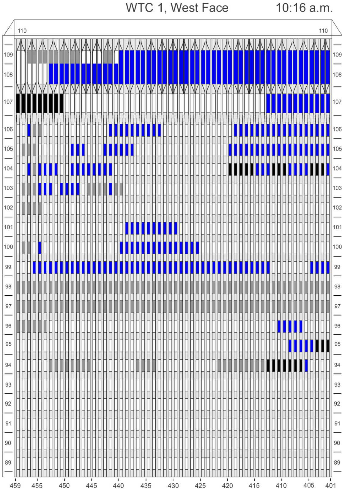
Figure F-56. Diagram of the west face of WTC 1 for floors 89 to 110 at 10:16 a.m. showing windows where smoke was observed and those that were hidden from view.
