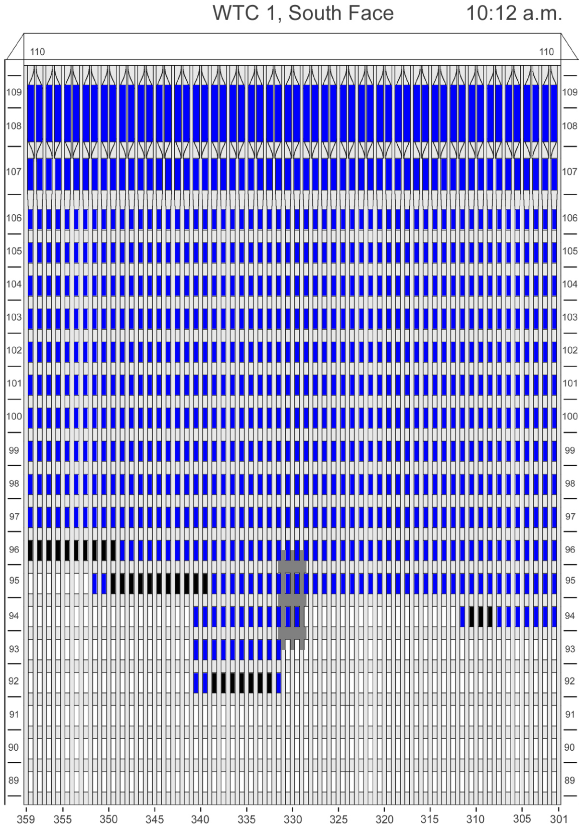
Figure E-42. Diagram of the south face of WTC 1 for floors 89 to 110 at 10:12 a.m. showing windows where smoke was observed and those that were hidden from view.
