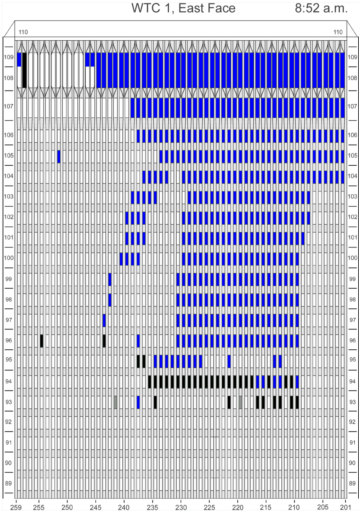
Figure D-4. Diagram of the east face of WTC 1 for floors 89 to 110 at 8:52 a.m. showing windows where smoke was observed and those that were hidden from view.
