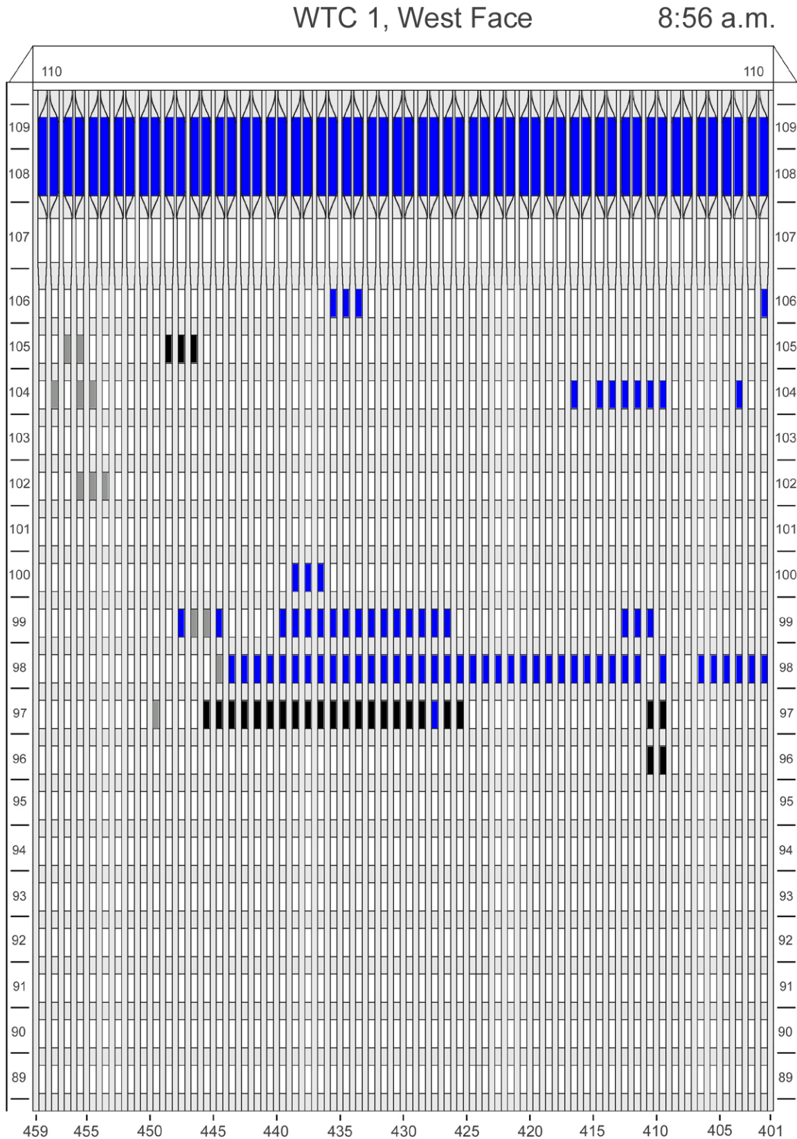
Figure F-12. Diagram of the west face of WTC 1 for floors 89 to 110 at 8:56 a.m. showing windows where smoke was observed and those that were hidden from view.
