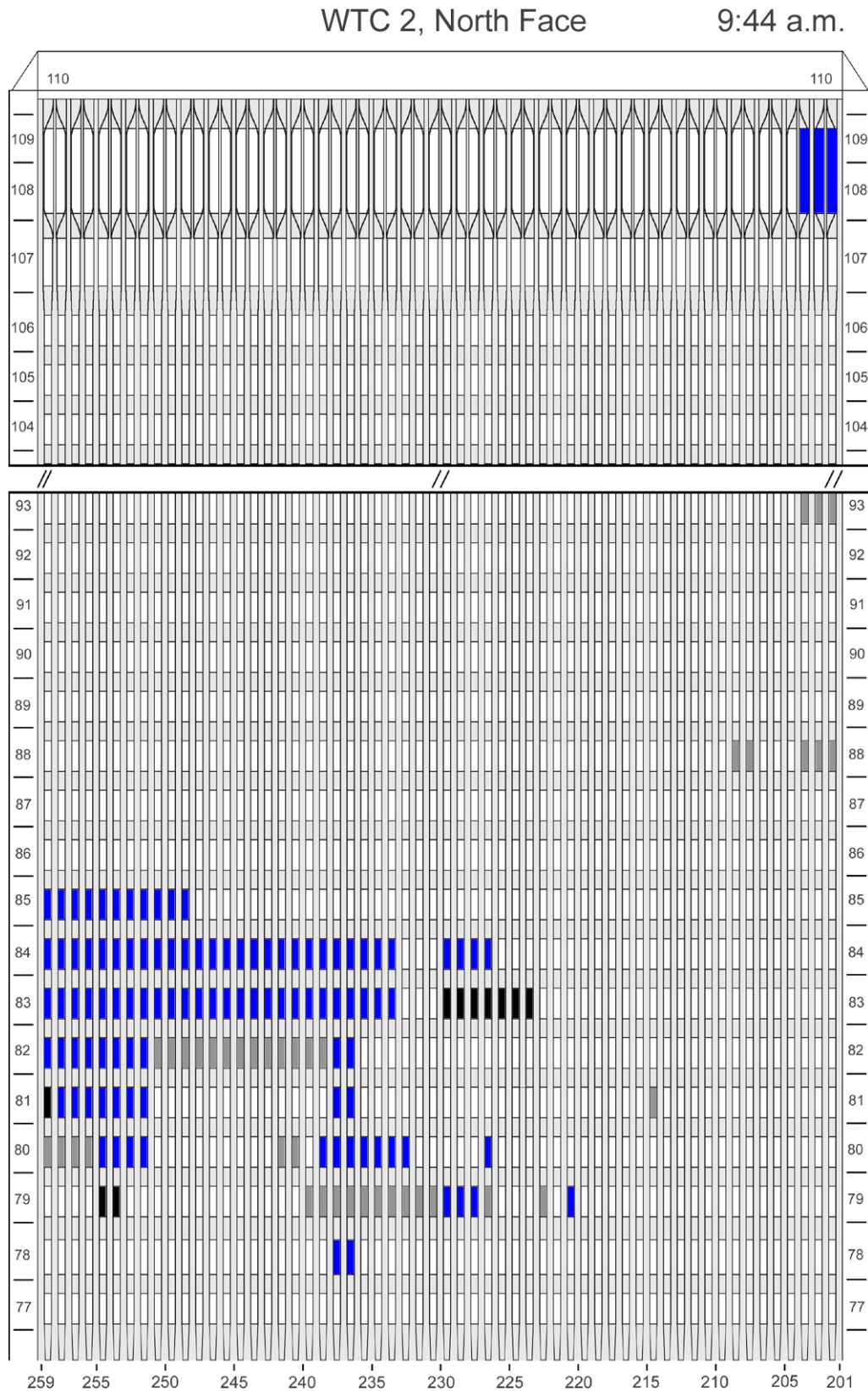
Figure G-44. Diagram of the north face of WTC 2 for floors 77 to 93 and floors 104 to 110 at 9:44 a.m. showing windows where smoke was observed and those hidden from view.
