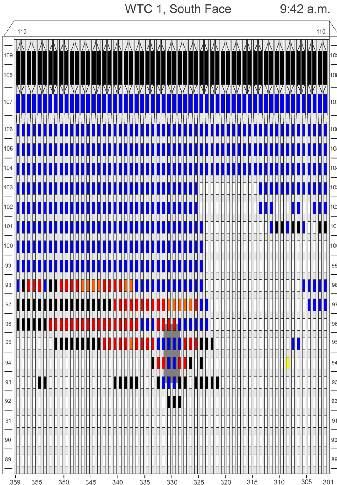
Figure E-27. Diagram of the south face of WTC 1 for floors 89 to 110 at 9:42 a.m. showing the condition of windows and locations of fires.
