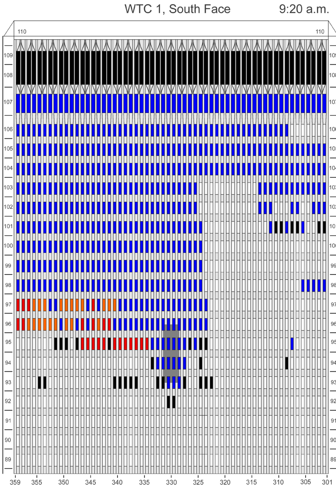
Figure E-17. Diagram of the south face of WTC 1 for floors 89 to 110 at 9:20 a.m. showing the condition of windows and locations of fires.
