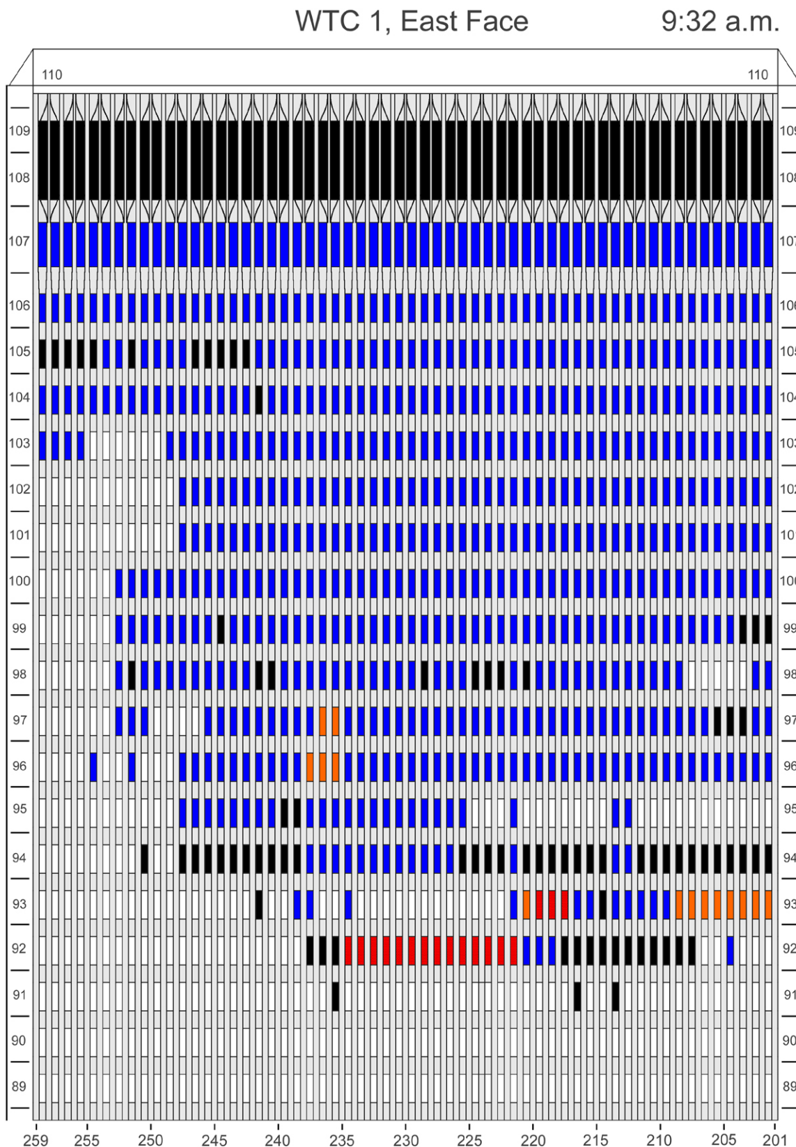
Figure D-23. Diagram of the east face of WTC 1 for floors 89 to 110 at 9:32 a.m. showing the condition of windows and locations of fires.
