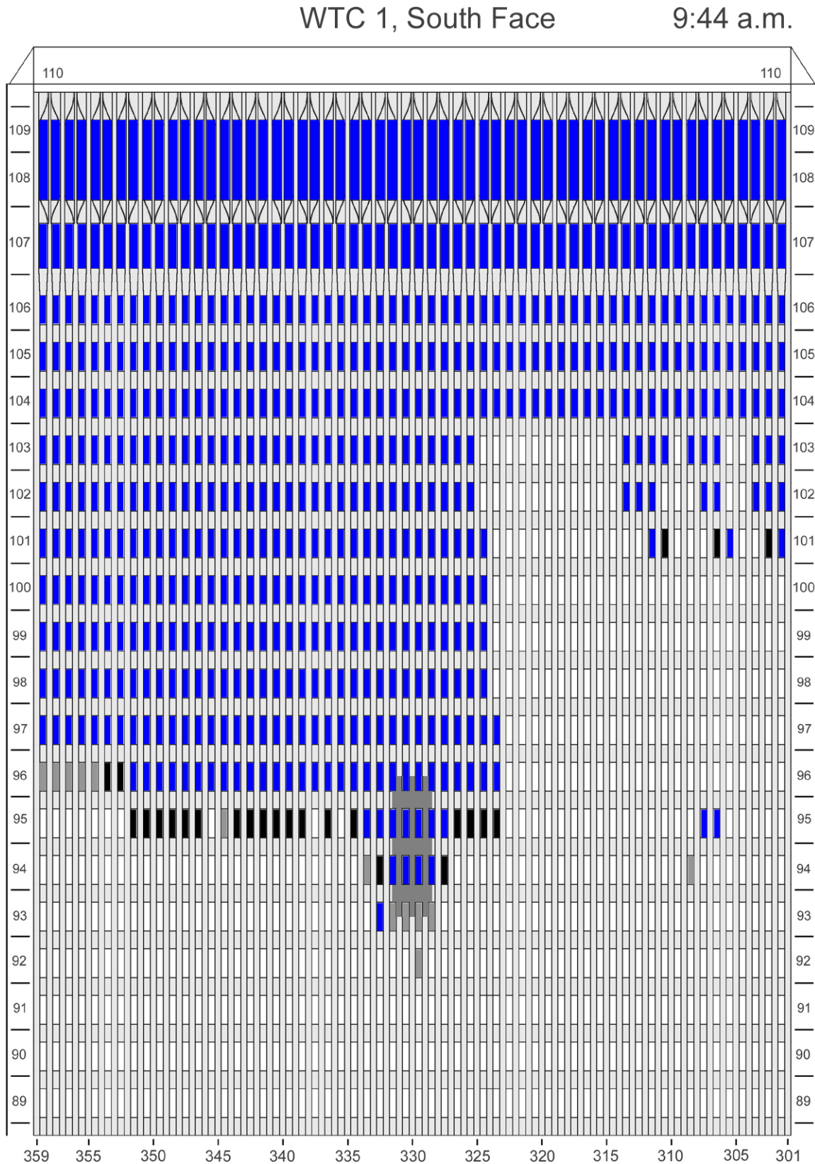
Figure E-30. Diagram of the south face of WTC 1 for floors 89 to 110 at 9:44 a.m. showing windows where smoke was observed and those that were hidden from view.
