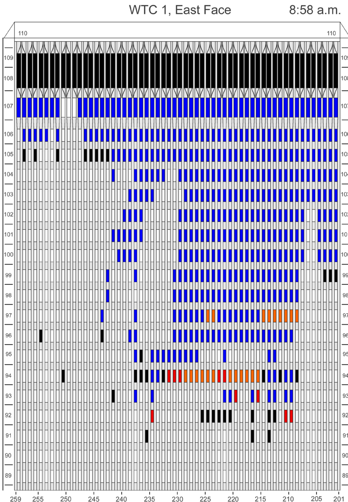
Figure D-7. Diagram of the east face of WTC 1 for floors 89 to 110 at 8:58 a.m. showing the condition of windows and locations of fires.
