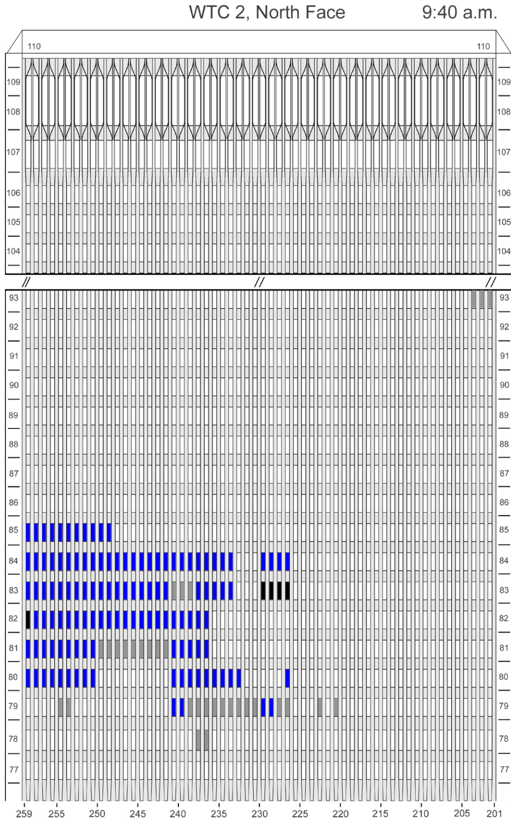
Figure G-40. Diagram of the north face of WTC 2 for floors 77 to 93 and floors 104 to 110 at 9:40 a.m. showing windows where smoke was observed and those hidden from view.
