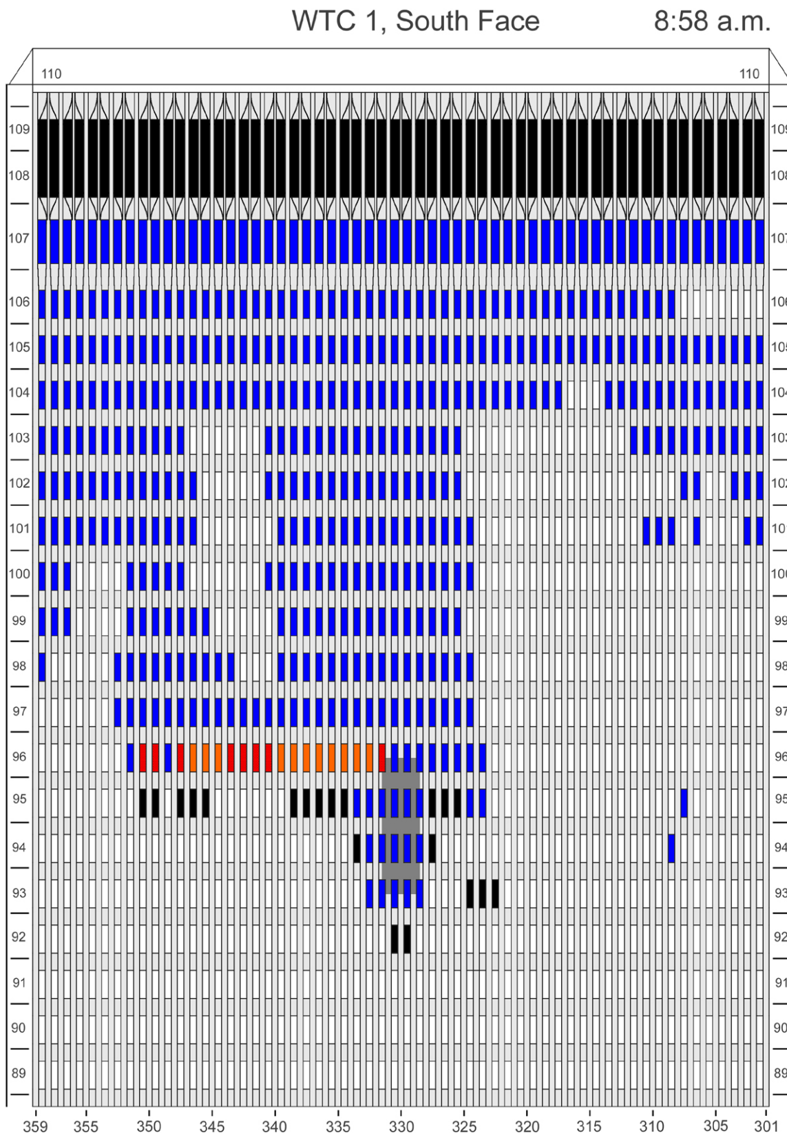
Figure E-7. Diagram of the south face of WTC 1 for floors 89 to 110 at 8:58 a.m. showing the condition of windows and locations of fires.
