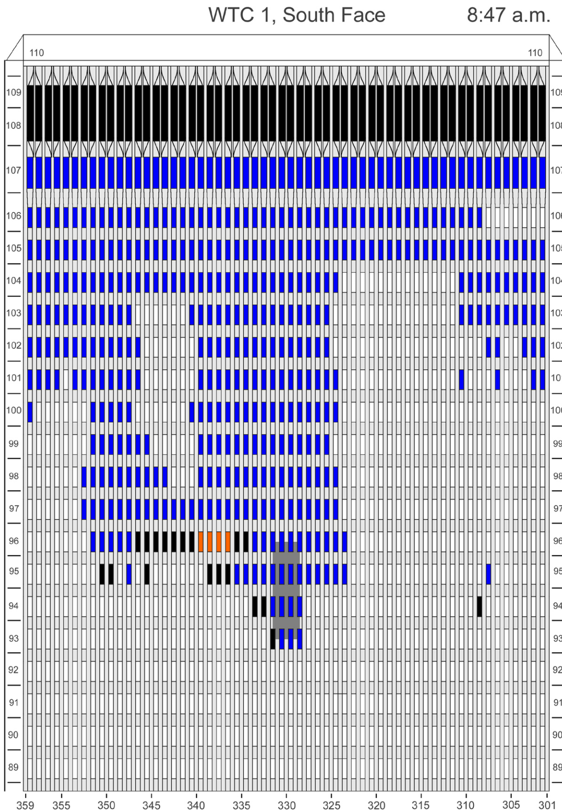
Figure E-1. Diagram of the south face of WTC 1 for floors 89 to 110 at 8:47 a.m. showing the condition of windows and locations of fires.
