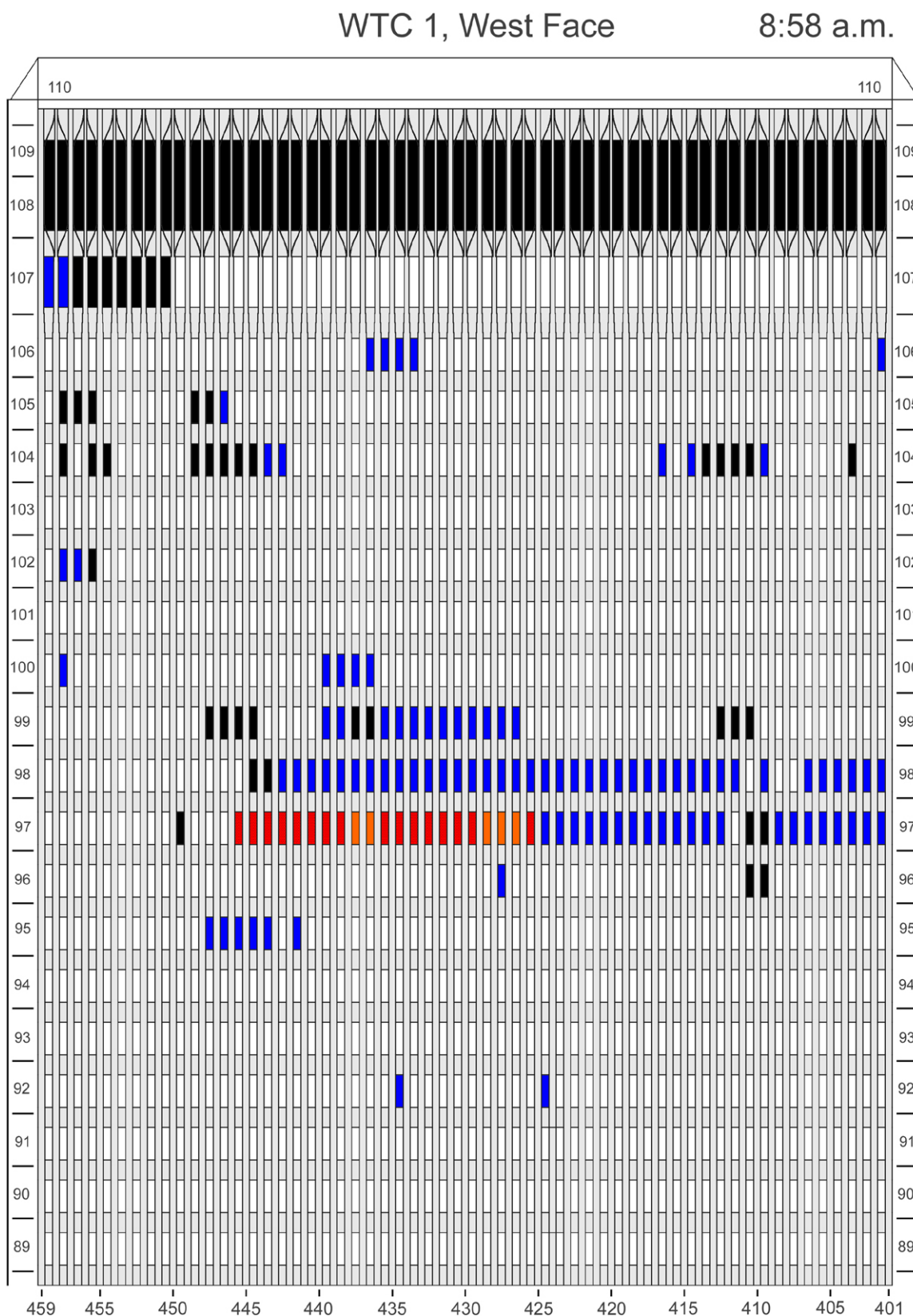
Figure F-13. Diagram of the west face of WTC 1 showing the condition of windows and locations of fires for floors 89 to 110 at 8:58 a.m.
