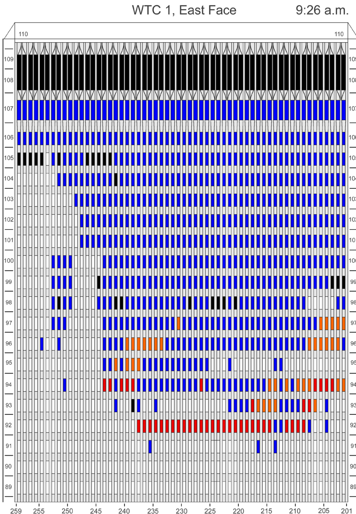
Figure D-21. Diagram of the east face of WTC 1 for floors 89 to 110 at 9:26 a.m. showing the condition of windows and locations of fires.
