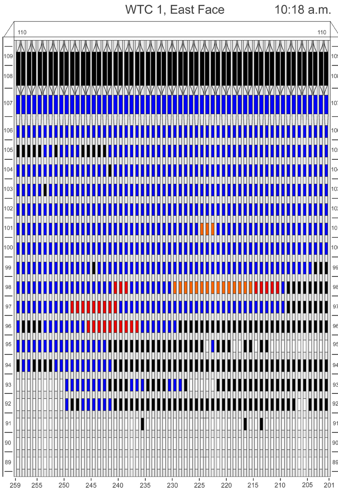
Figure D-45. Diagram of the east face of WTC 1 for floors 89 to 110 at 10:18 a.m. showing the condition of windows and locations of fires.
