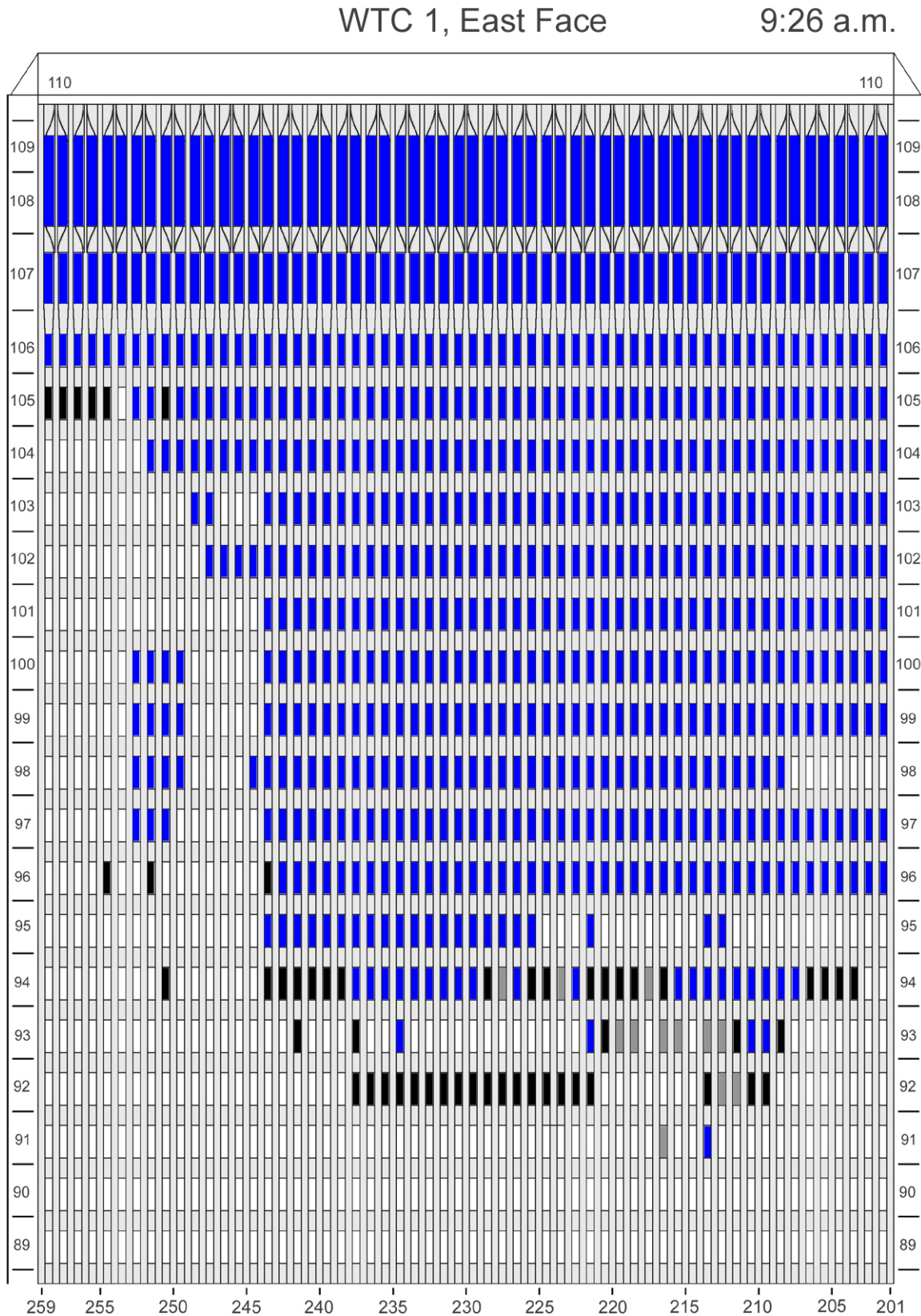
Figure D-22. Diagram of the east face of WTC 1 for floors 89 to 110 at 9:26 a.m. showing windows where smoke was observed and those that were hidden from view.
