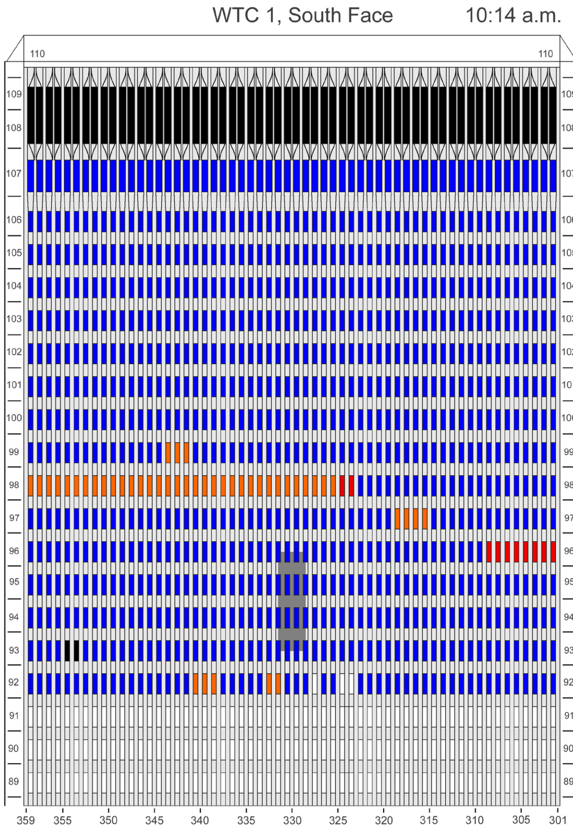
Figure E-43. Diagram of the south face of WTC 1 for floors 89 to 110 at 10:14 a.m. showing the condition of windows and locations of fires.
