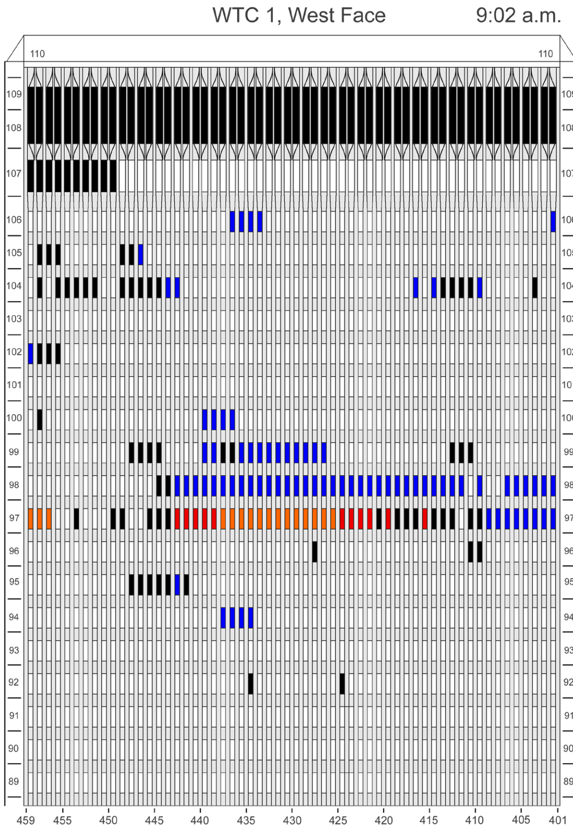
Figure F-17. Diagram of the west face of WTC 1 for floors 89 to 110 at 9:02 a.m. showing the condition of windows and locations of fires.
