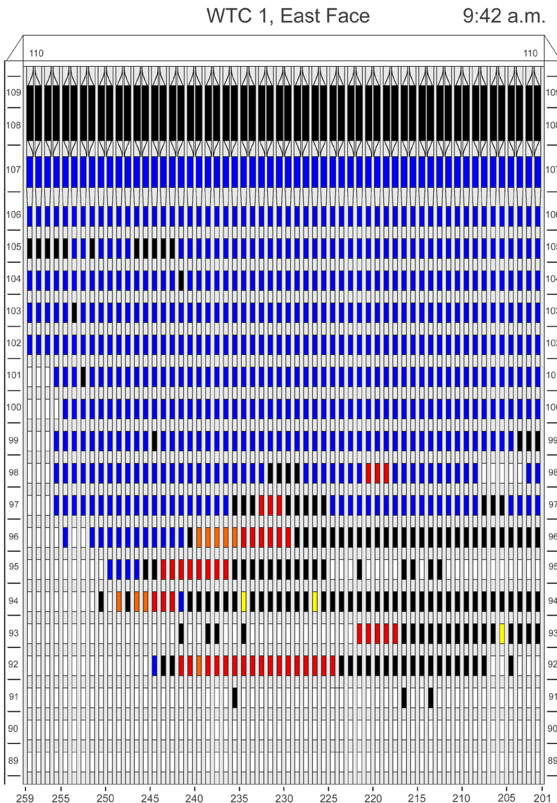
Figure D-27. Diagram of the east face of WTC 1 for floors 89 to 110 at 9:42 a.m. showing the condition of windows and locations of fires.
