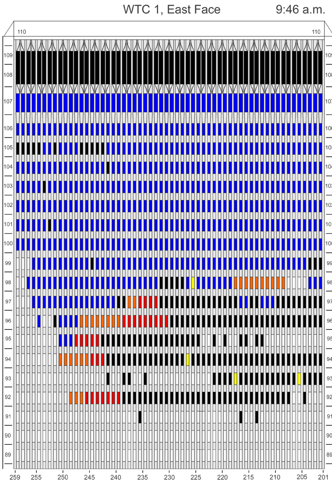
Figure D-29. Diagram of the east face of WTC 1 for floors 89 to 110 at 9:46 a.m. showing the condition of windows and locations of fires.
