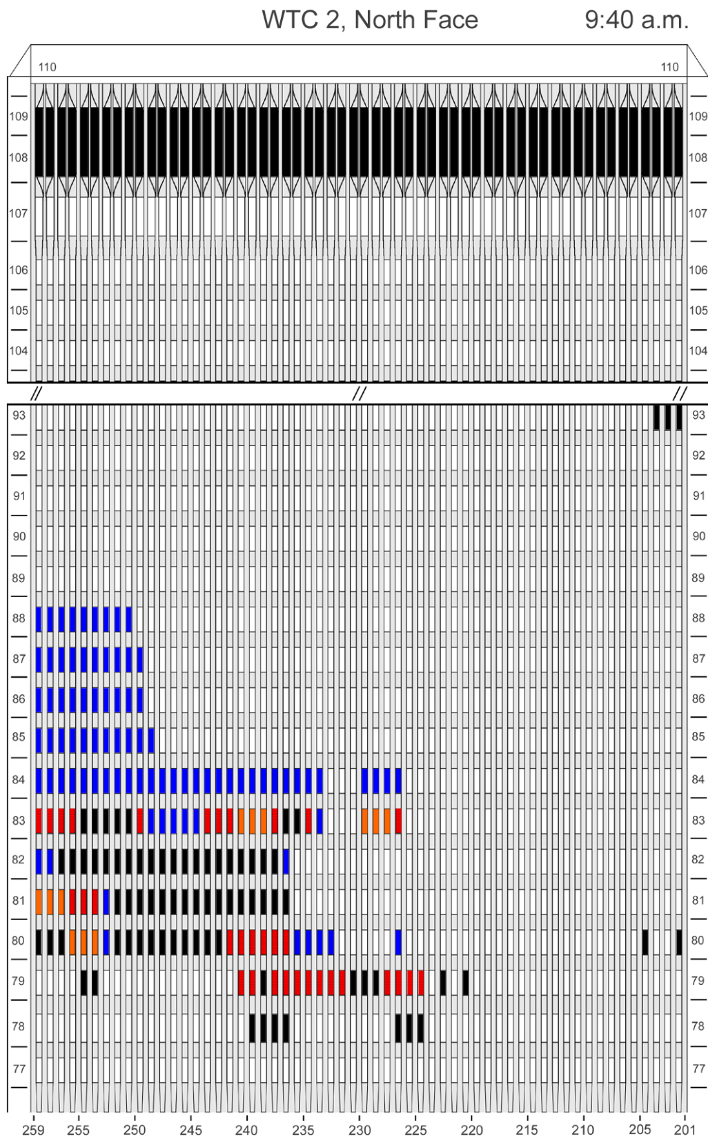
Figure G-39. Diagram of the north face of WTC 2 for floors 77 to 93 and floors 104 to 110 at 9:40 a.m. showing the condition of windows and locations of fires.
