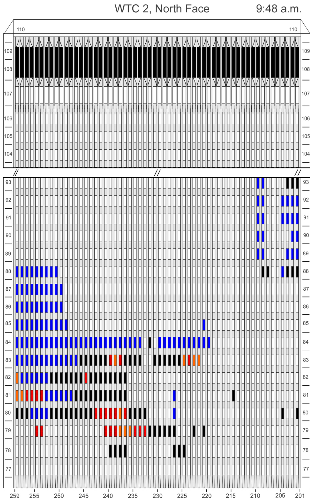
Figure G-47. Diagram of the north face of WTC 2 for floors 77 to 93 and floors 104 to 110 at 9:48 a.m. showing the condition of windows and locations of fires.
