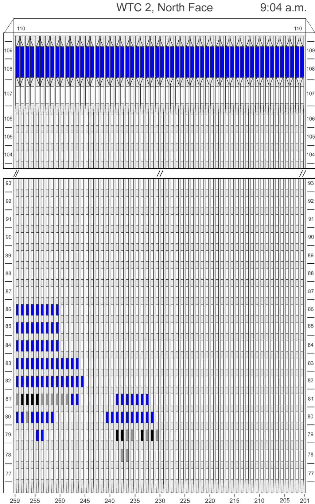
Figure G-4. Diagram of the north face of WTC 2 for floors 77 to 93 and floors 104 to 110 at 9:04 a.m. showing windows where smoke was observed and those hidden from view.
