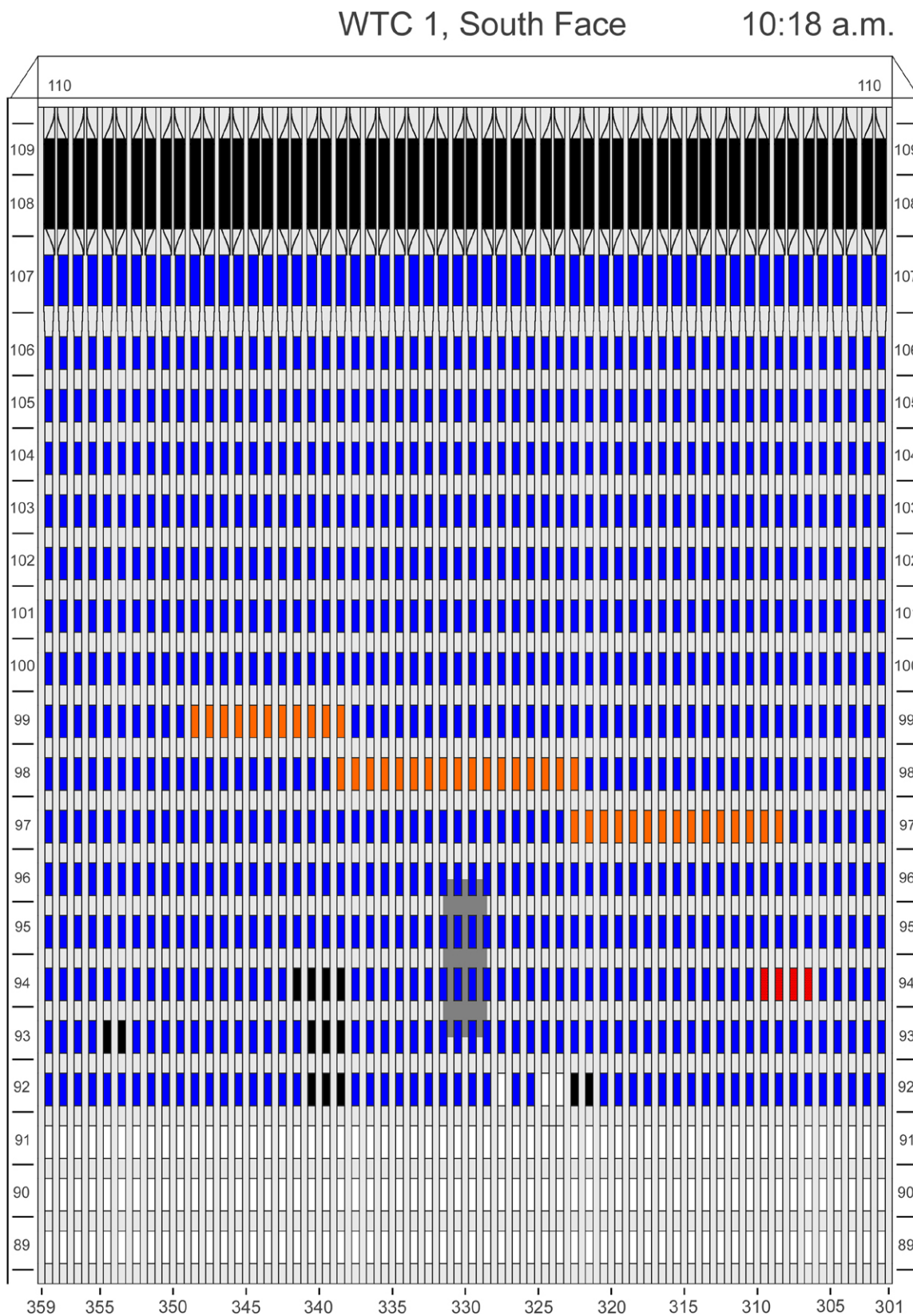
Figure E-45. Diagram of the south face of WTC 1 for floors 89 to 110 at 10:18 a.m. showing the condition of windows and locations of fires.
