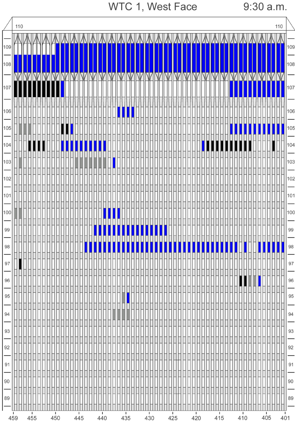
Figure F-34. Diagram of the west face of WTC 1 for floors 89 to 110 at 9:30 a.m. showing windows where smoke was observed and those that were hidden from view.
