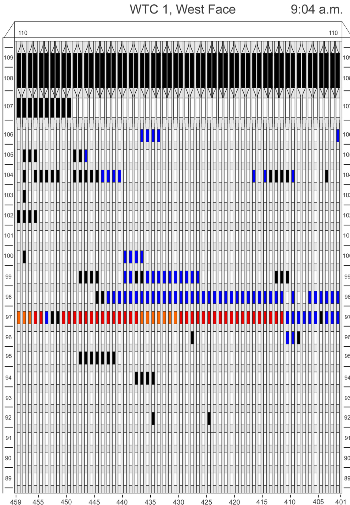
Figure F-19. Diagram of the west face of WTC 1 for floors 89 to 110 at 9:04 a.m. showing the condition of windows and locations of fires.
