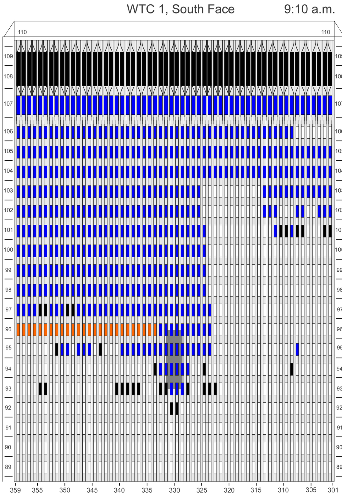
Figure E-13. Diagram of the south face of WTC 1 for floors 89 to 110 at 9:10 a.m. showing the condition of windows and locations of fires.
