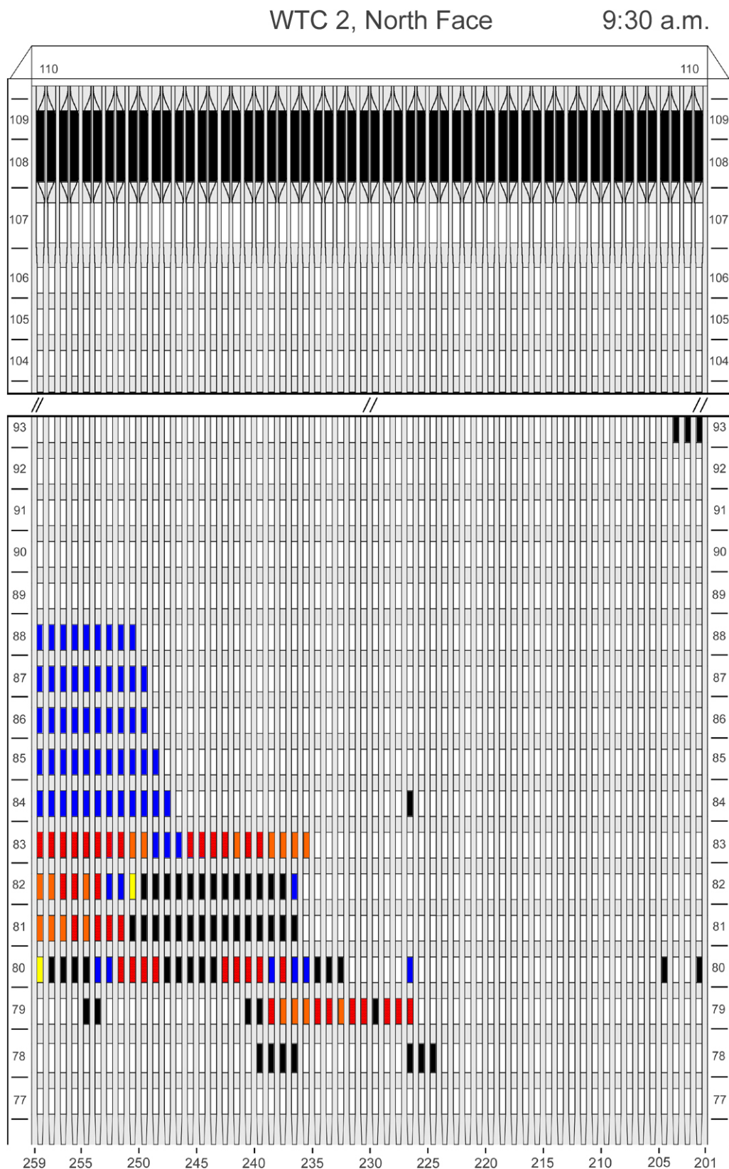
Figure G-29. Diagram of the north face of WTC 2 for floors 77 to 93 and floors 104 to 110 at 9:30 a.m. showing the condition of windows and locations of fires.
