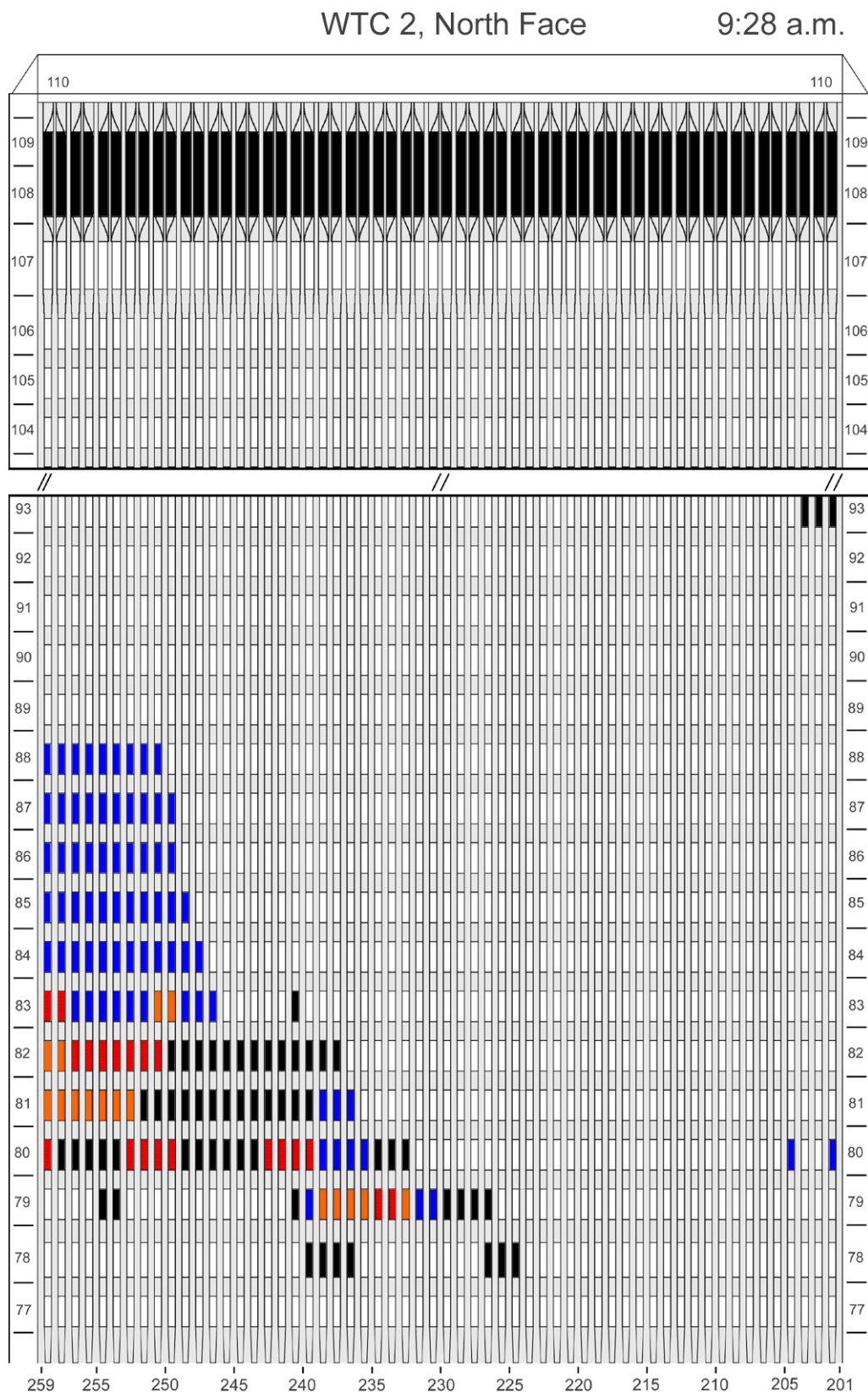
Figure G-27. Diagram of the north face of WTC 2 for floors 77 to 93 and floors 104 to 110 at 9:28 a.m. showing the condition of windows and locations of fires.
