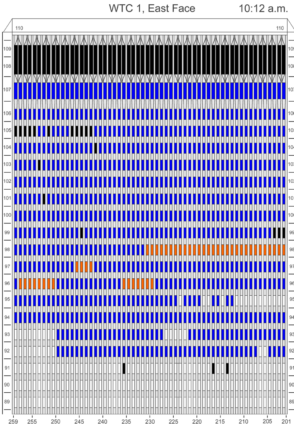
Figure D-43. Diagram of the east face of WTC 1 for floors 89 to 110 at 10:12 a.m. showing the condition of windows and locations of fires.
