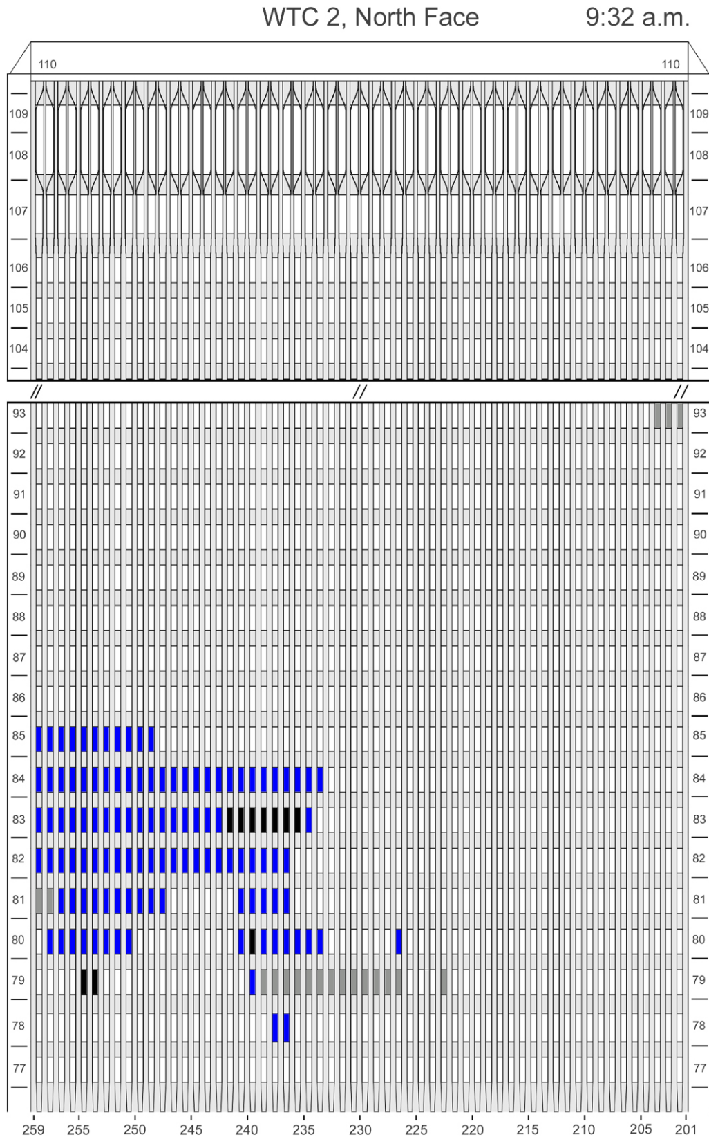
Figure G-32. Diagram of the north face of WTC 2 for floors 77 to 93 and floors 104 to 110 at 9:32 a.m. showing windows where smoke was observed and those hidden from view.
