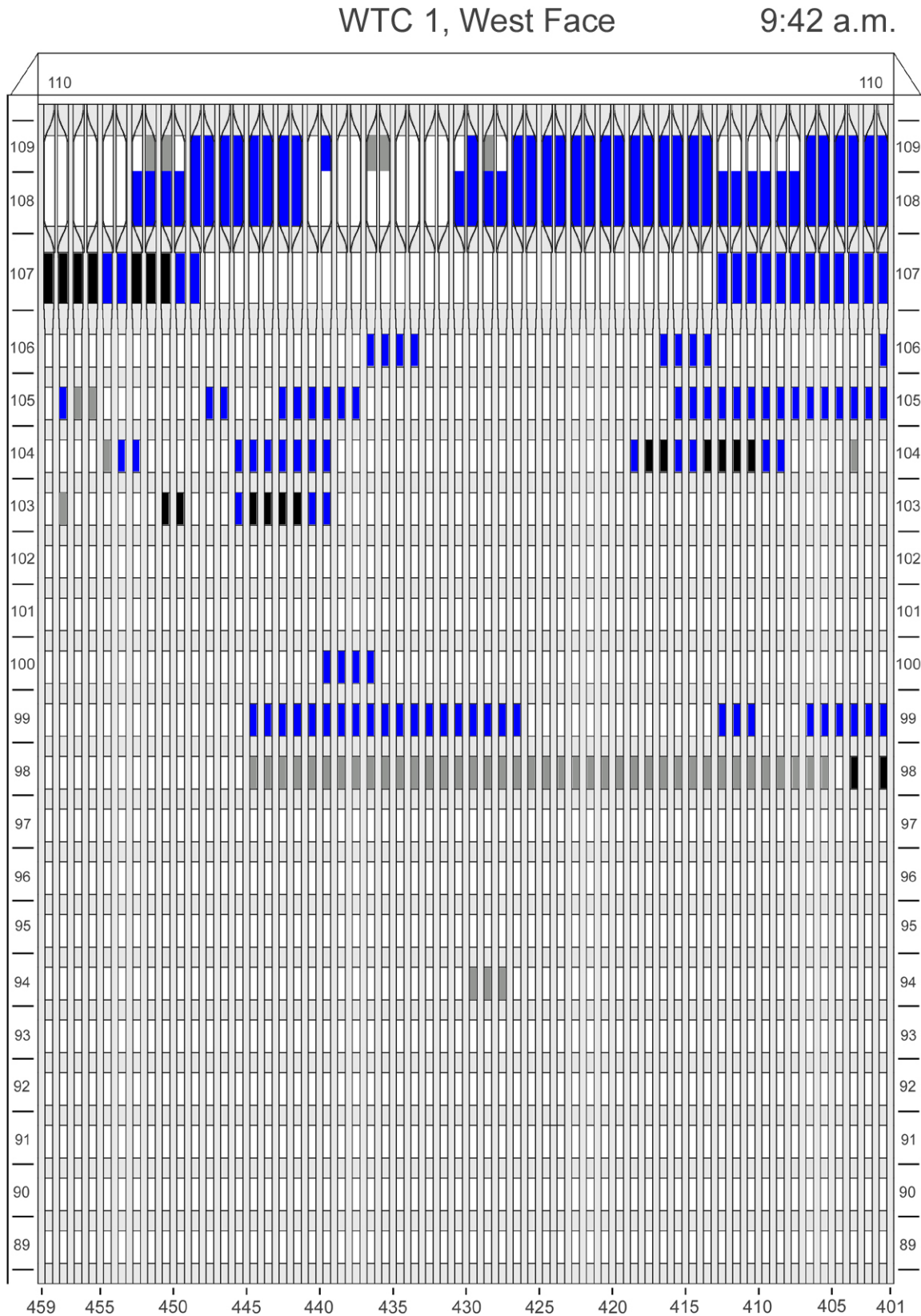
Figure F-40. Diagram of the west face of WTC 1 for floors 89 to 110 at 9:42 a.m. showing windows where smoke was observed and those that were hidden from view.
