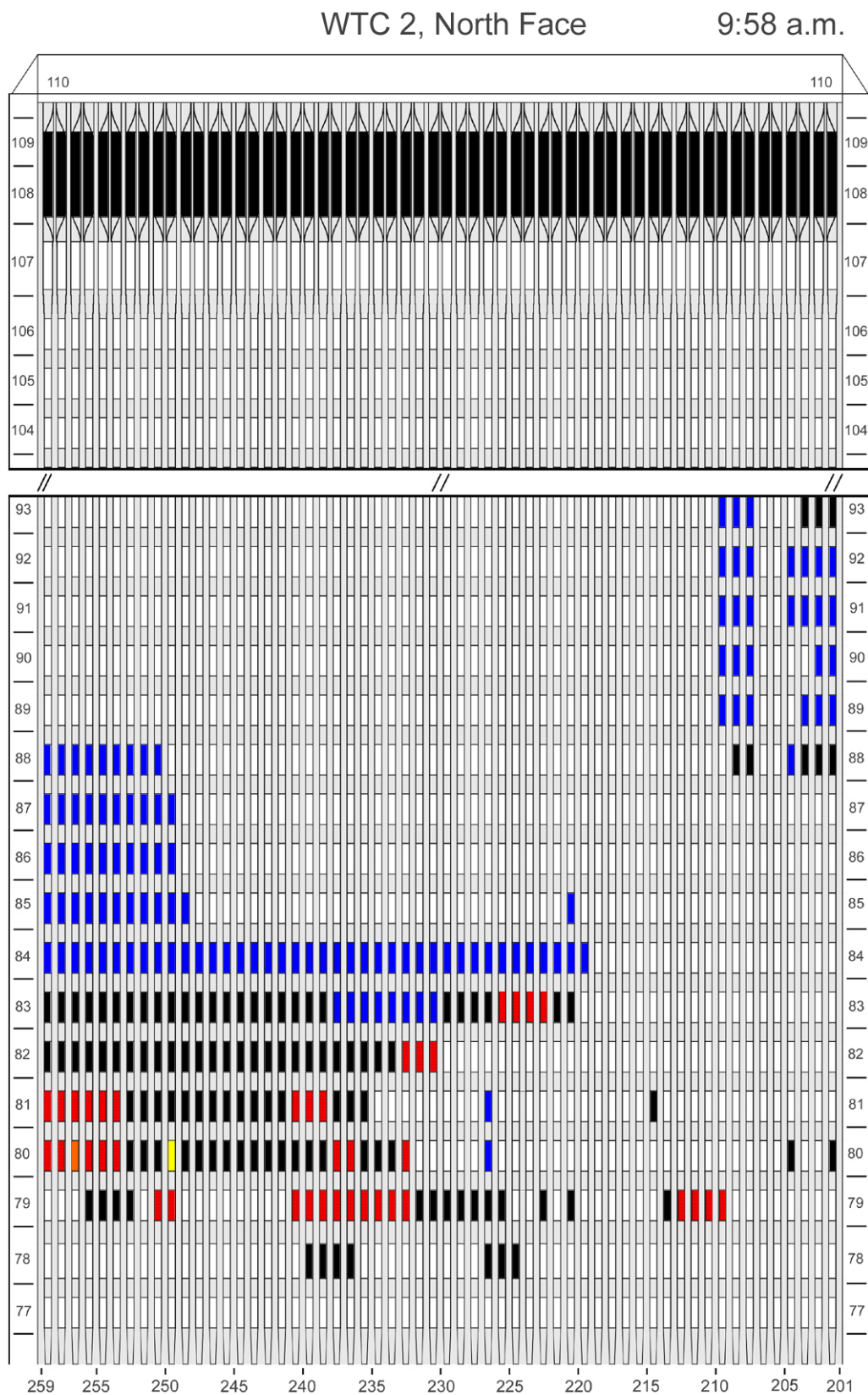
Figure G-57. Diagram of the north face of WTC 2 for floors 77 to 93 and floors 104 to 110 at 9:58 a.m. showing the condition of windows and locations of fires.
