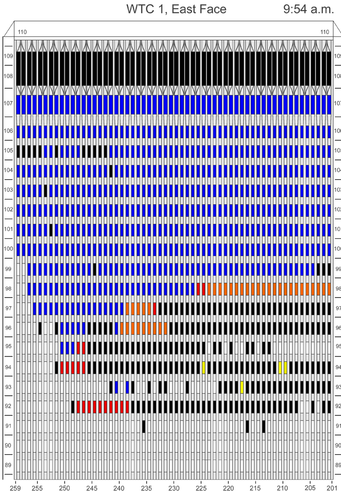
Figure D-33. Diagram of the east face of WTC 1 for floors 89 to 110 at 9:54 a.m. showing the condition of windows and locations of fires.
