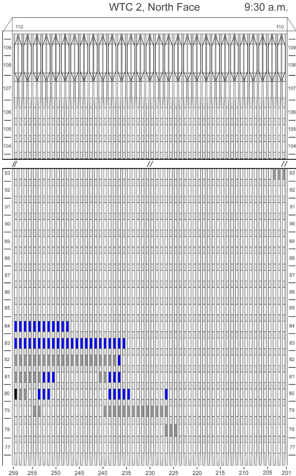
Figure G-30. Diagram of the north face of WTC 2 for floors 77 to 93 and floors 104 to 110 at 9:30 a.m. showing windows where smoke was observed and those hidden from view.
