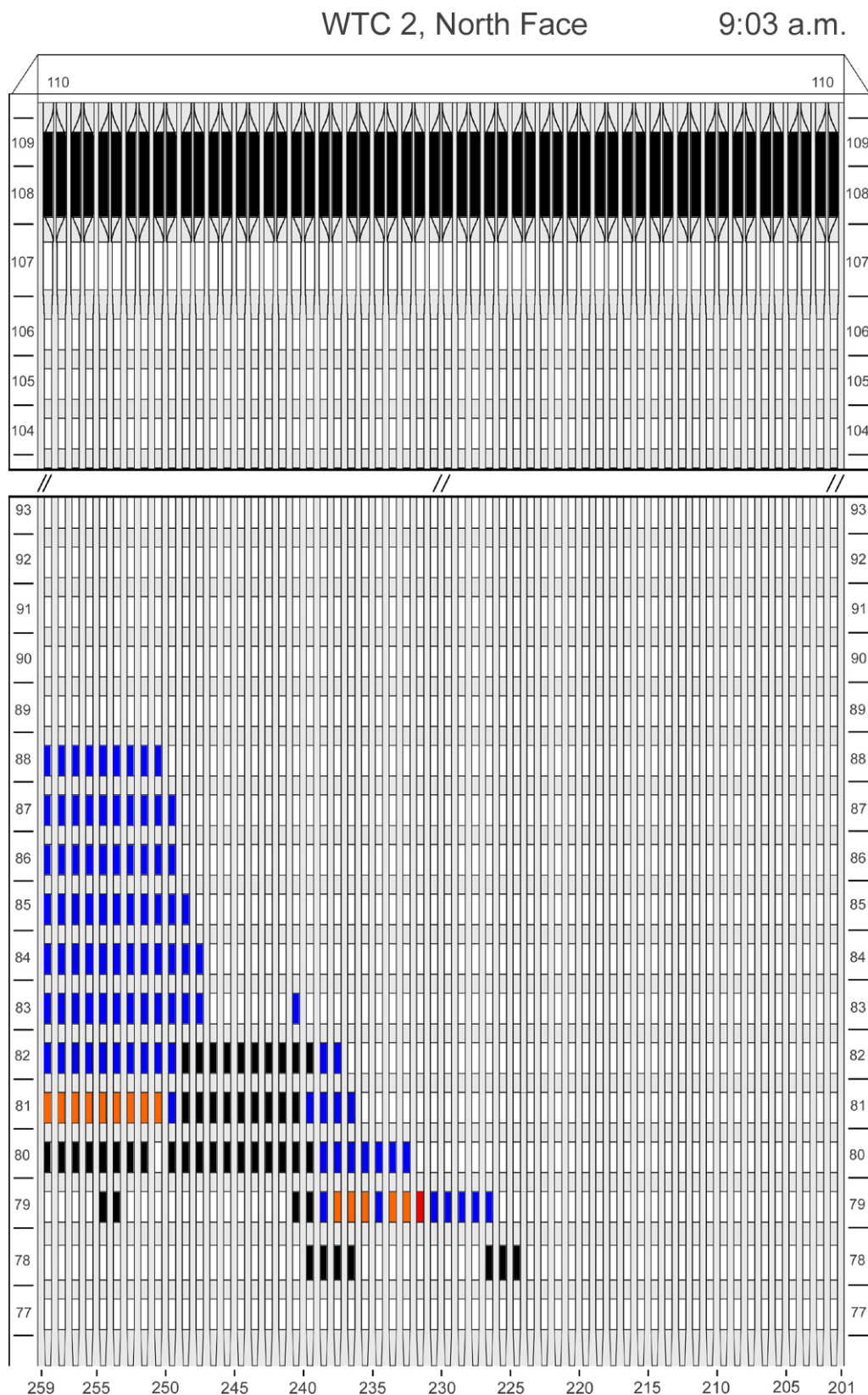
Figure G-1. Diagram of the north face of WTC 2 for floors 77 to 93 and floors 104 to 110 at 9:03 a.m. showing the condition of windows and locations of fires.
