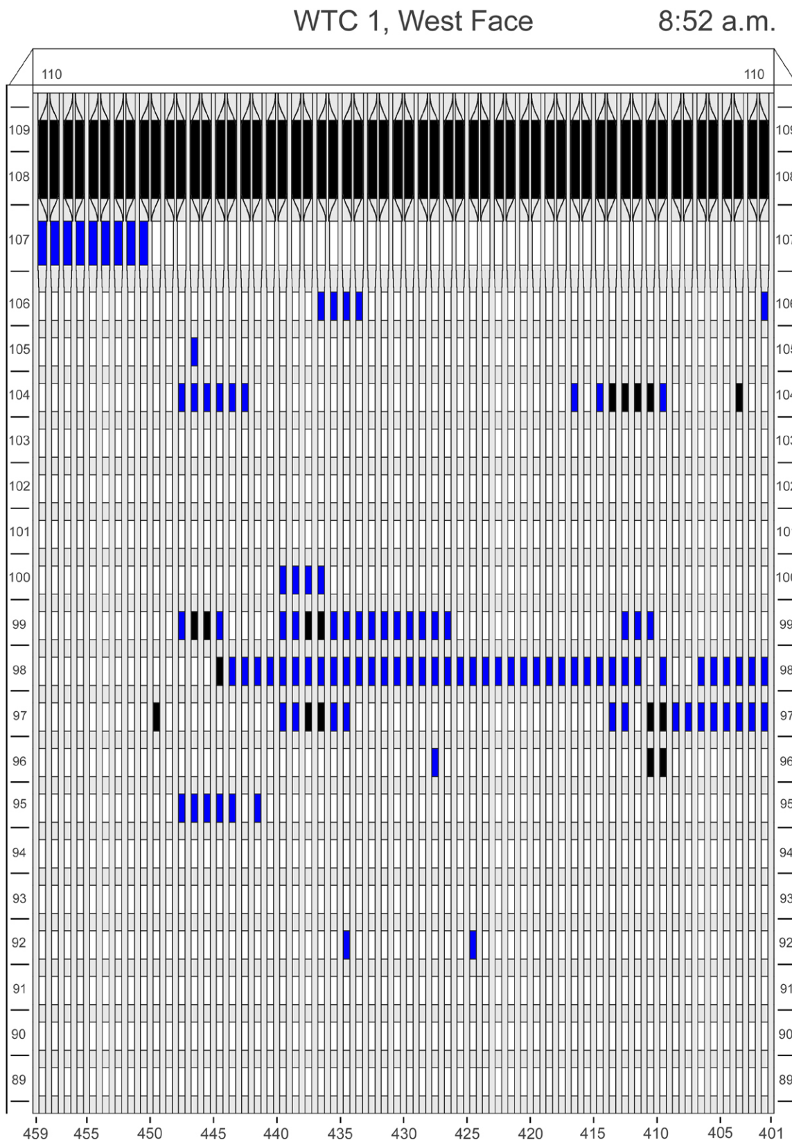
Figure F-7. Diagram of the west face of WTC 1 for floors 89 to 110 at 8:52 a.m. showing the condition of windows and locations of fires.
