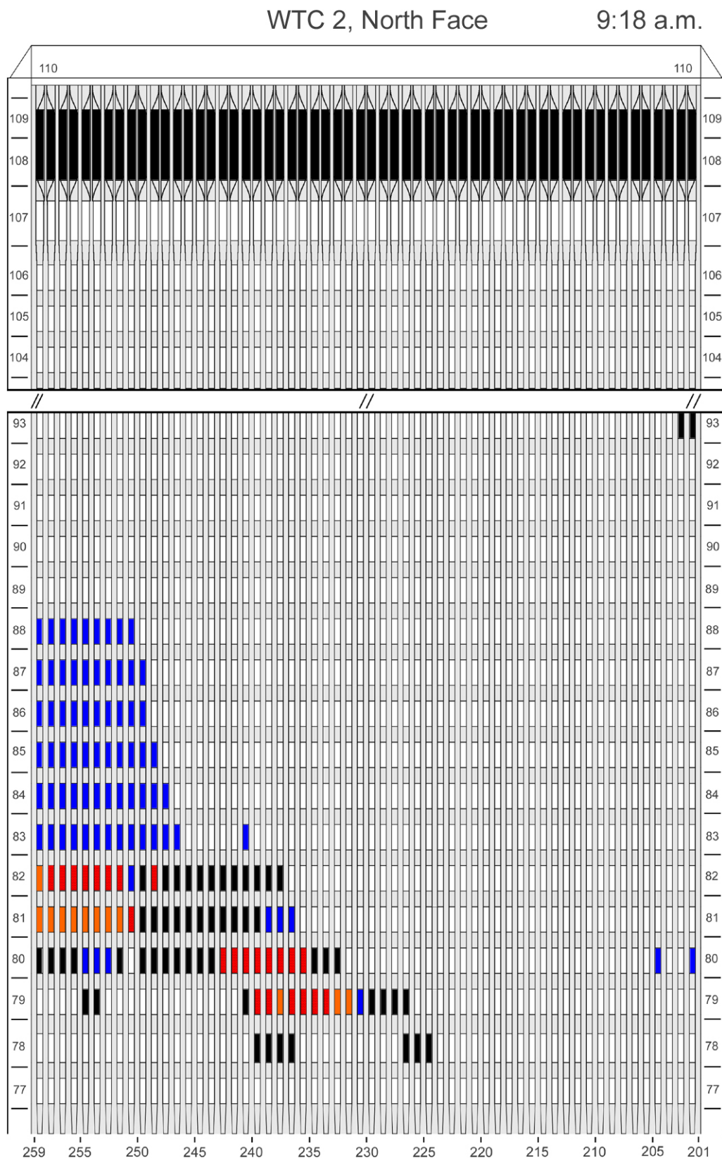
Figure G-17. Diagram of the north face of WTC 2 for floors 77 to 93 and floors 104 to 110 at 9:18 a.m. showing the condition of windows and locations of fires.
