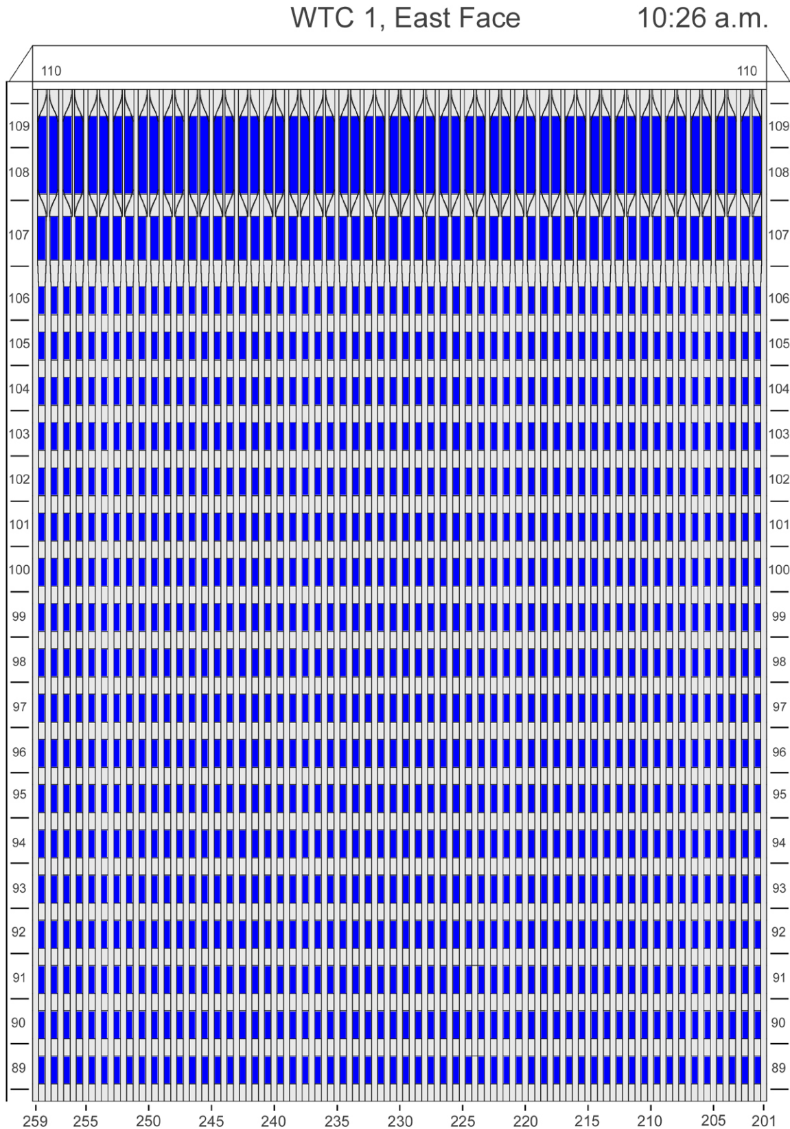
Figure D-50. Diagram of the east face of WTC 1 for floors 89 to 110 at 10:26 a.m. showing windows where smoke was observed and those that were hidden from view.
