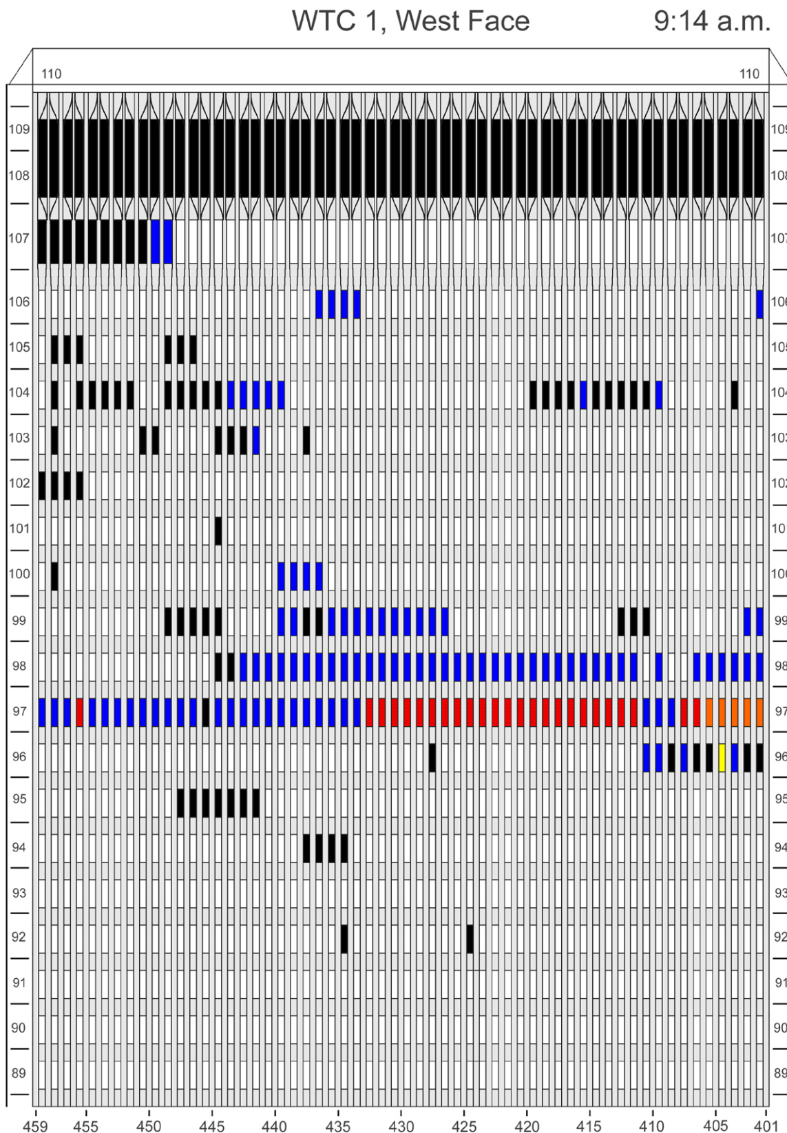
Figure F-27. Diagram of the west face of WTC 1 for floors 89 to 110 at 9:14 a.m. showing the condition of windows and locations of fires.
