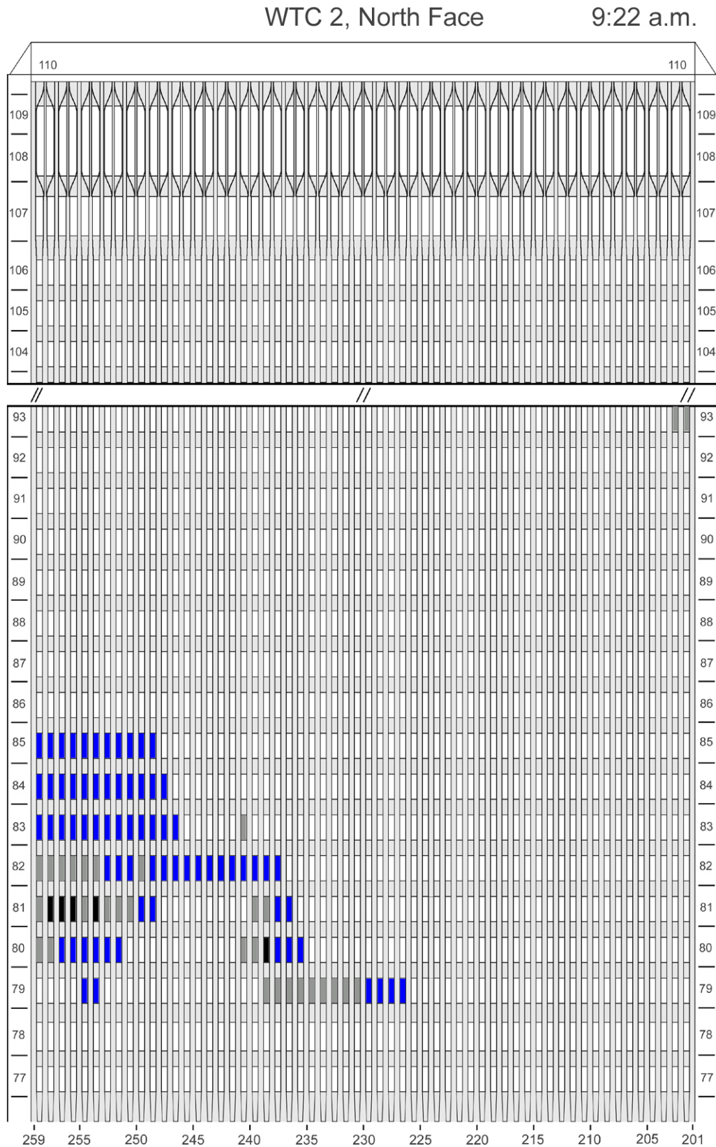
Figure G-22. Diagram of the north face of WTC 2 for floors 77 to 93 and floors 104 to 110 at 9:22 a.m. showing windows where smoke was observed and those hidden from view.
