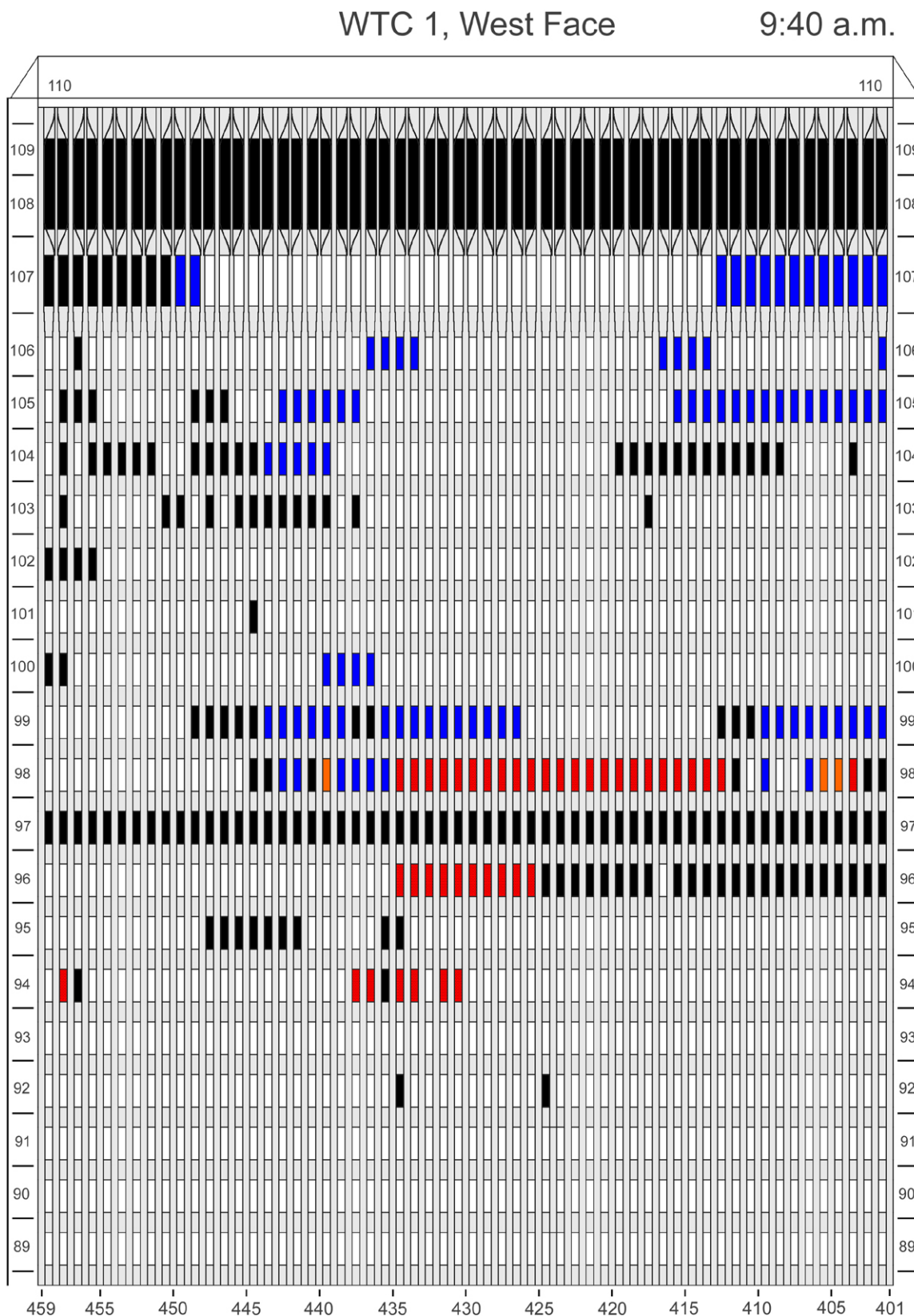
Figure F-37. Diagram of the west face of WTC 1 for floors 89 to 110 at 9:40 a.m. showing the condition of windows and locations of fires.
