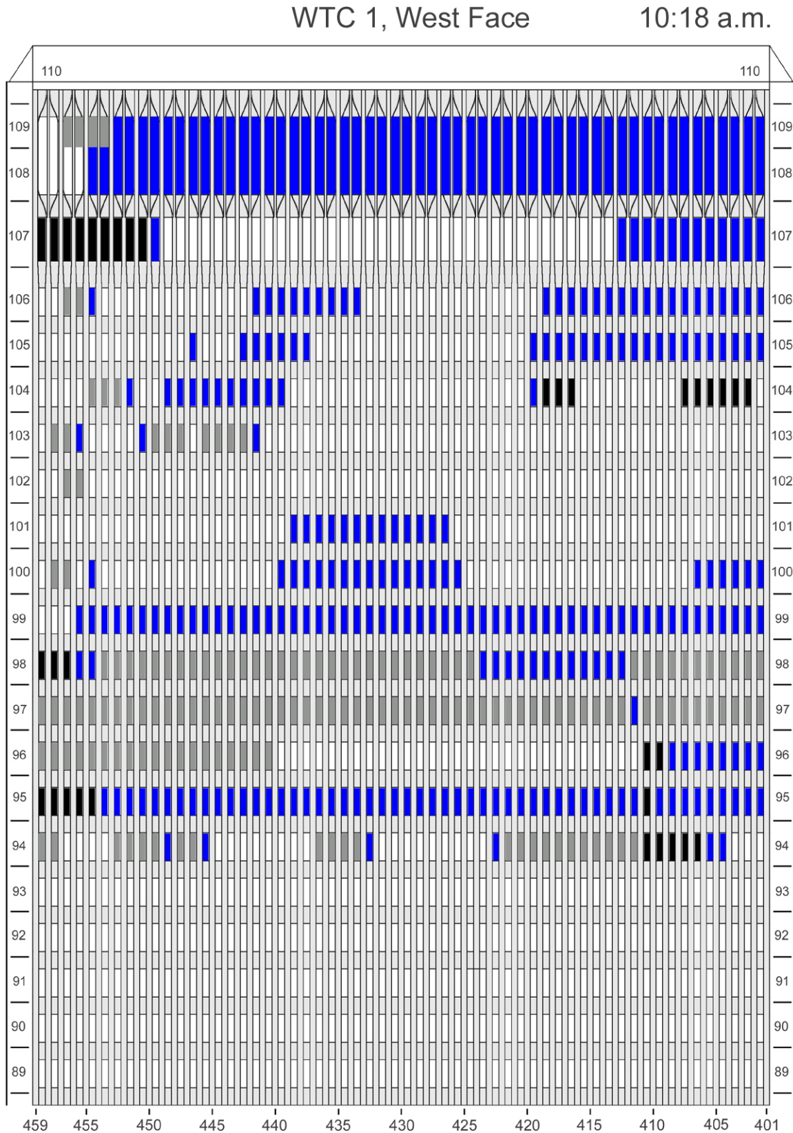
Figure F-58. Diagram of the west face of WTC 1 for floors 89 to 110 at 10:18 a.m. showing windows where smoke was observed and those that were hidden from view.
