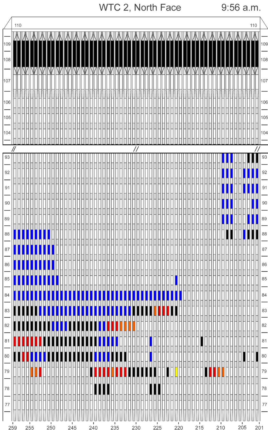
Figure G-55. Diagram of the north face of WTC 2 for floors 77 to 93 and floors 104 to 110 at 9:56 a.m. showing the condition of windows and locations of fires.
