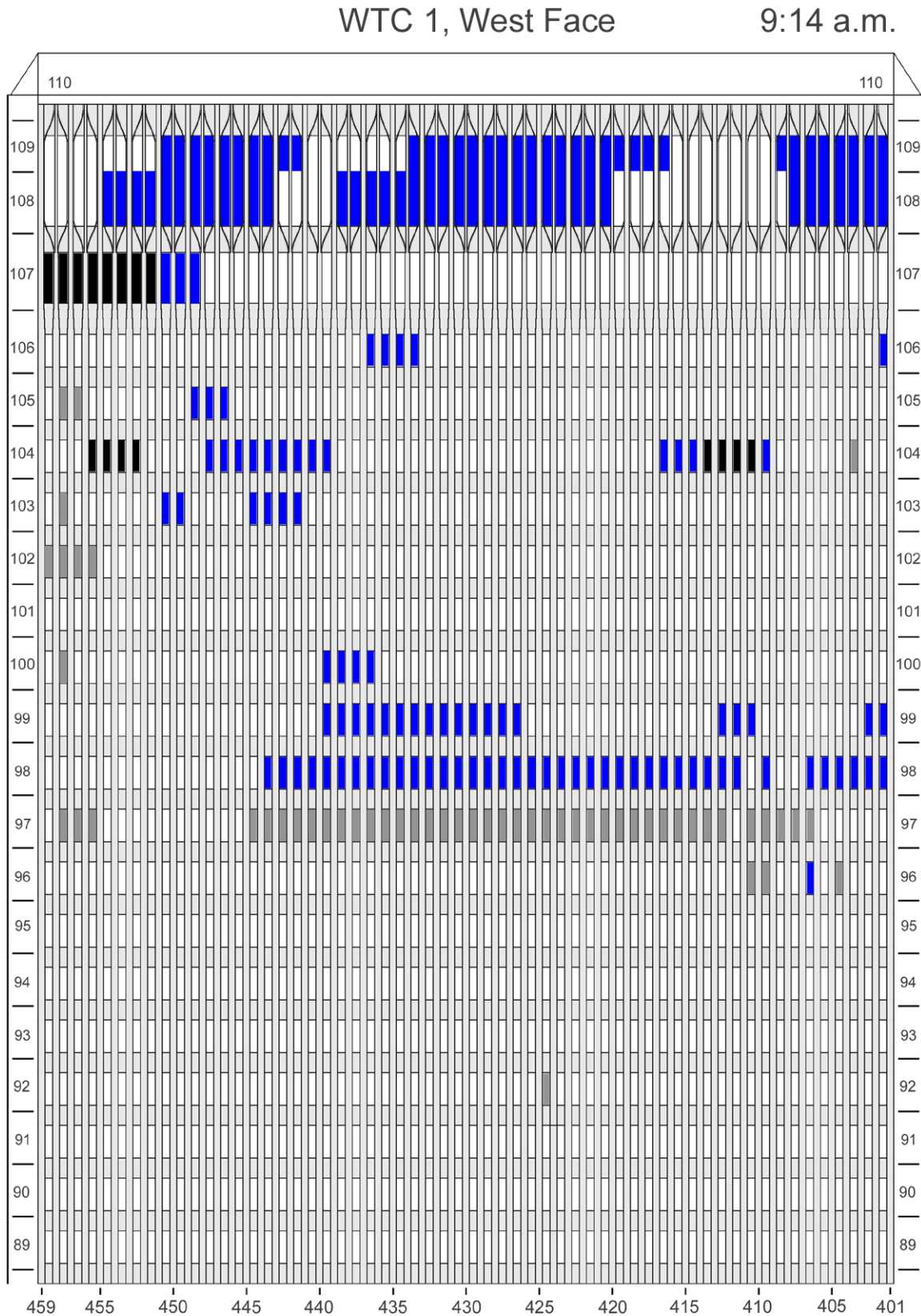
Figure F-28. Diagram of the west face of WTC 1 for floors 89 to 110 at 9:14 a.m. showing windows where smoke was observed and those that were hidden from view.
