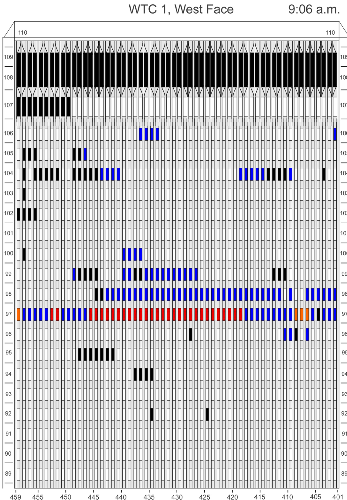
Figure F-21. Diagram of the west face of WTC 1 for floors 89 to 110 at 9:06 a.m. showing the condition of windows and locations of fires.
