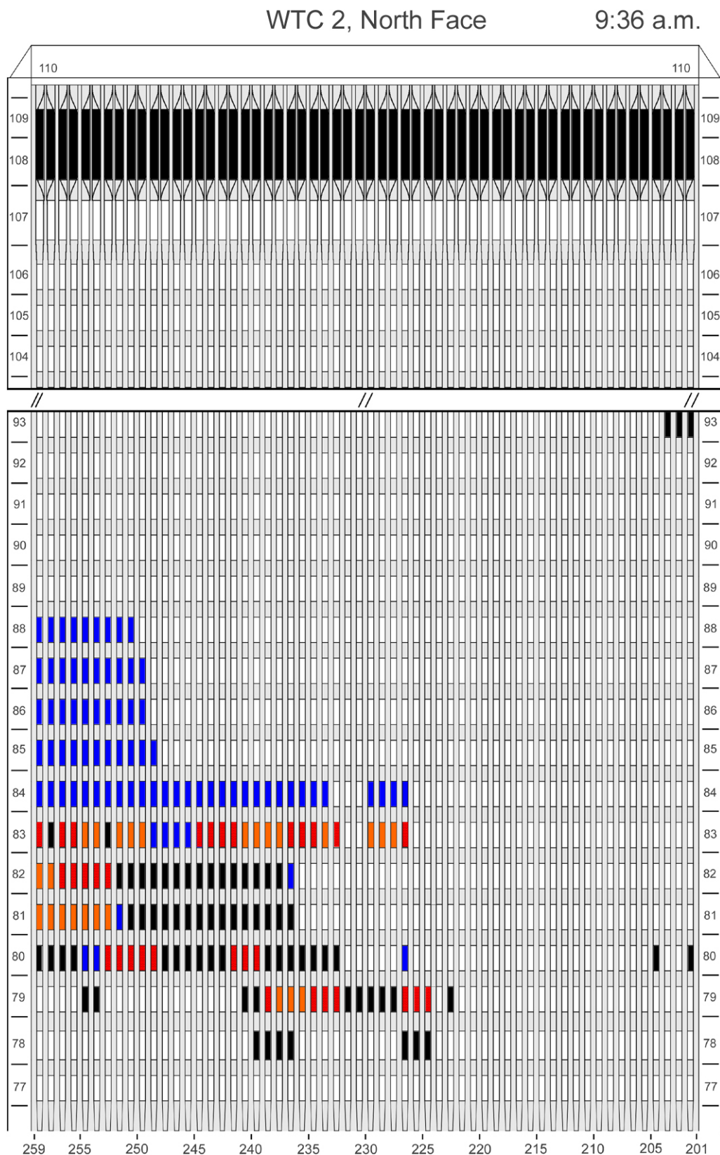
Figure G-35. Diagram of the north face of WTC 2 for floors 77 to 93 and floors 104 to 110 at 9:36 a.m. showing the condition of windows and locations of fires.
