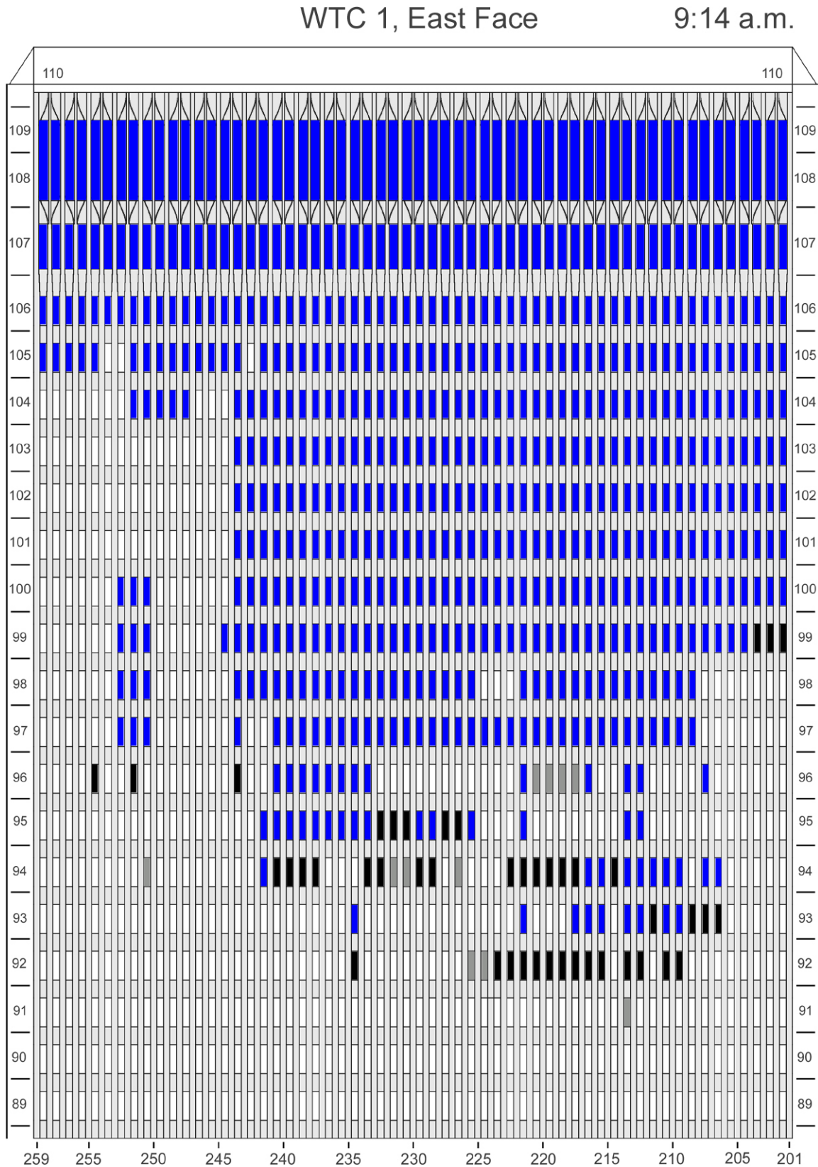
Figure D-18. Diagram of the east face of WTC 1 for floors 89 to 110 at 9:14 a.m. showing windows where smoke was observed and those that were hidden from view.
