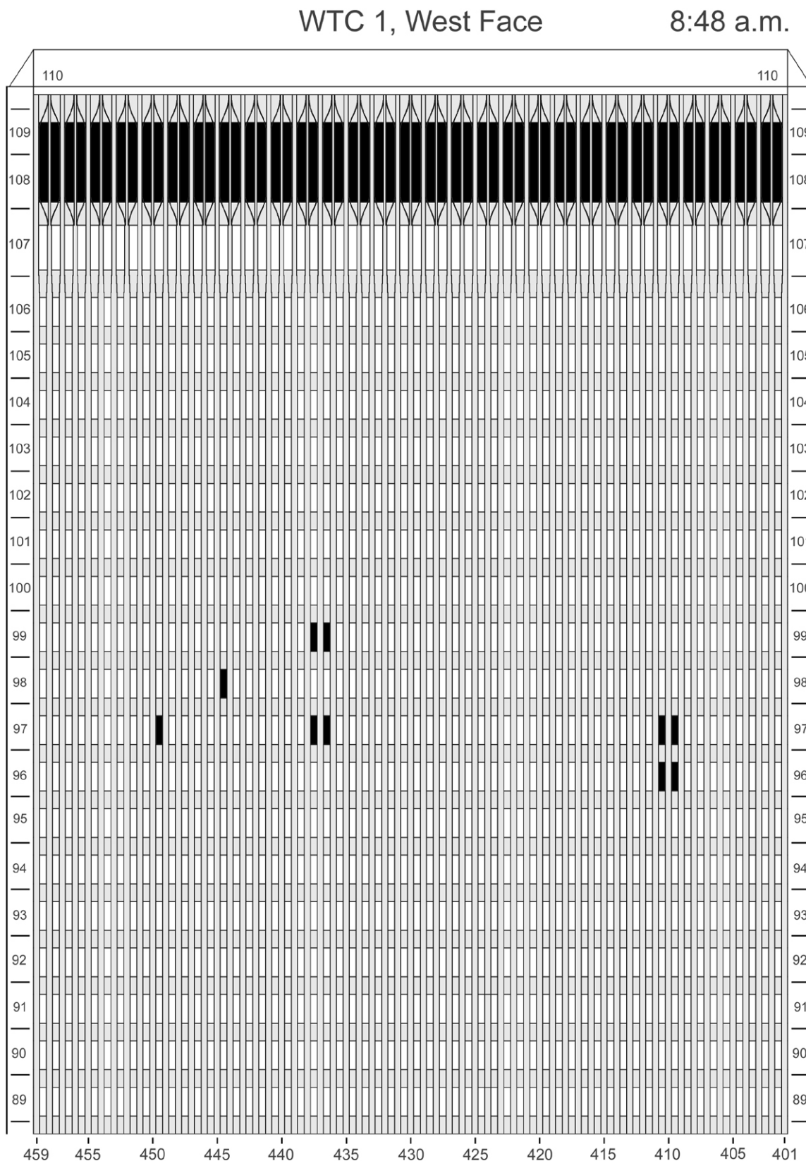
Figure F-3. Diagram of the west face of WTC 1 for floors 89 to 110 at 8:48 a.m. showing the condition of windows and locations of fires.
