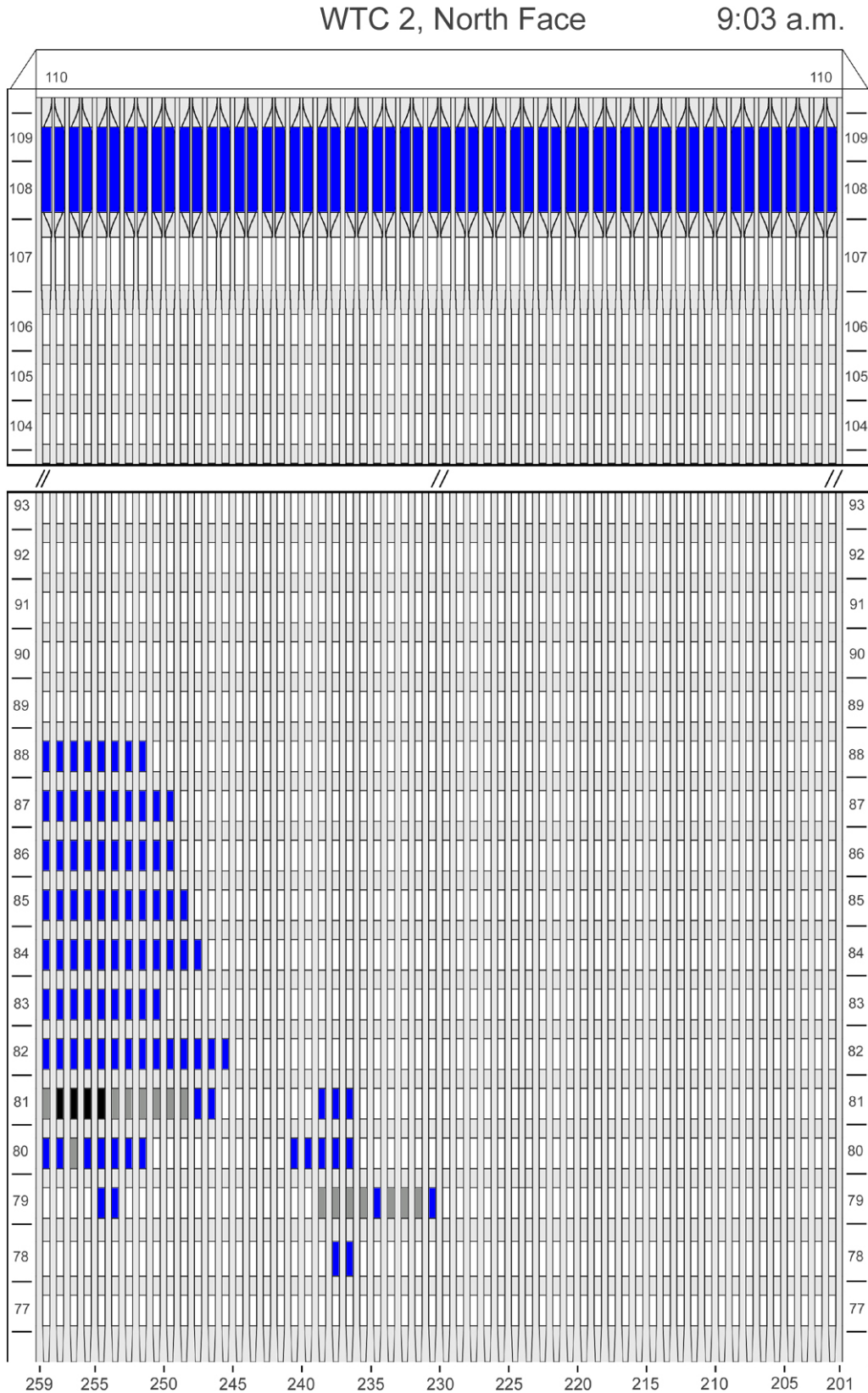
Figure G-2. Diagram of the north face of WTC 2 for floors 77 to 93 and floors 104 to 110 at 9:03 a.m. showing windows where smoke was observed and those hidden from view.
