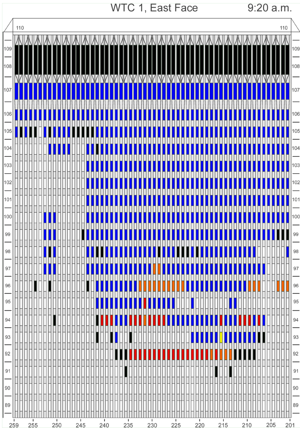
Figure D-19. Diagram of the east face of WTC 1 for floors 89 to 110 at 9:20 a.m. showing the condition of windows and locations of fires.
