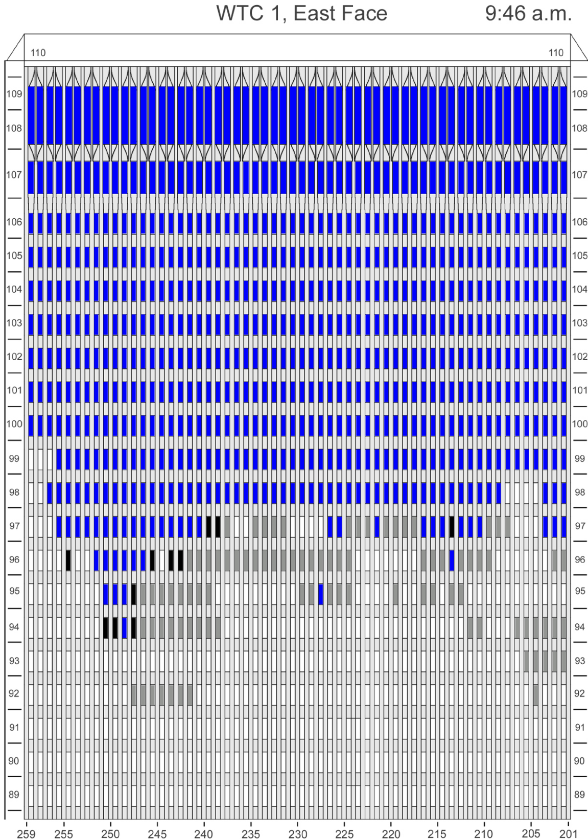
Figure D-30. Diagram of the east face of WTC 1 for floors 89 to 110 at 9:46 a.m. showing windows where smoke was observed and those that were hidden from view.
