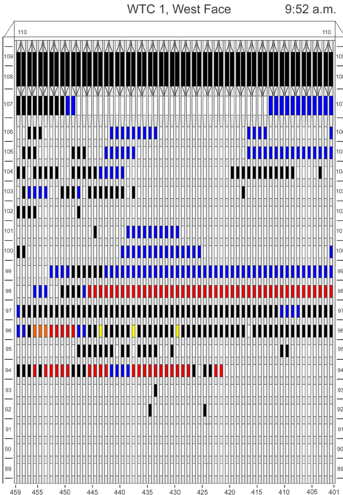
Figure F-45. Diagram of the west face of WTC 1 for floors 89 to 110 at 9:52 a.m. showing the condition of windows and locations of fires.
