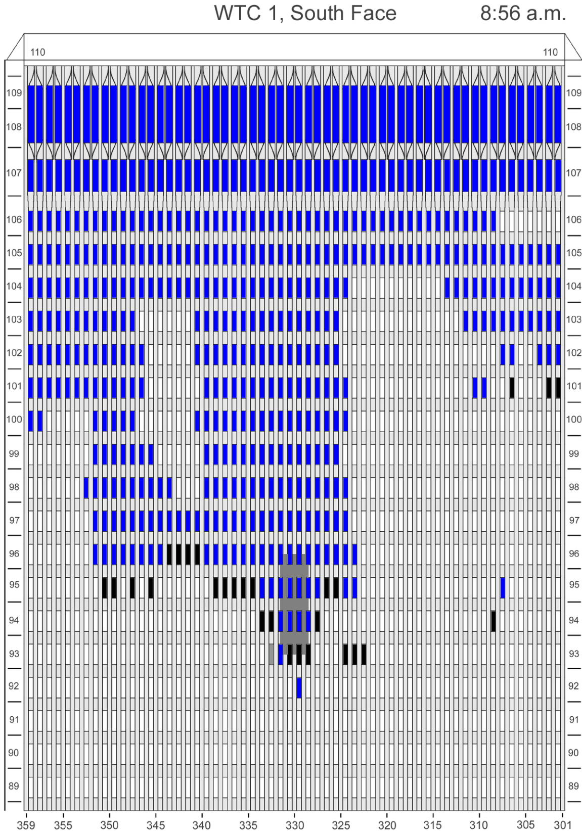
Figure E-6. Diagram of the south face of WTC 1 for floors 89 to 110 at 8:56 a.m. showing windows where smoke was observed and those that were hidden from view.
