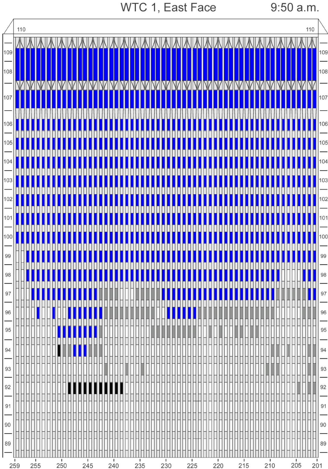
Figure D-32. Diagram of the east face of WTC 1 for floors 89 to 110 at 9:50 a.m. showing windows where smoke was observed and those that were hidden from view.
