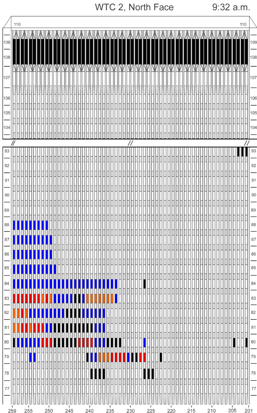
Figure G-31. Diagram of the north face of WTC 2 for floors 77 to 93 and floors 104 to 110 at 9:32 a.m. showing the condition of windows and locations of fires.
