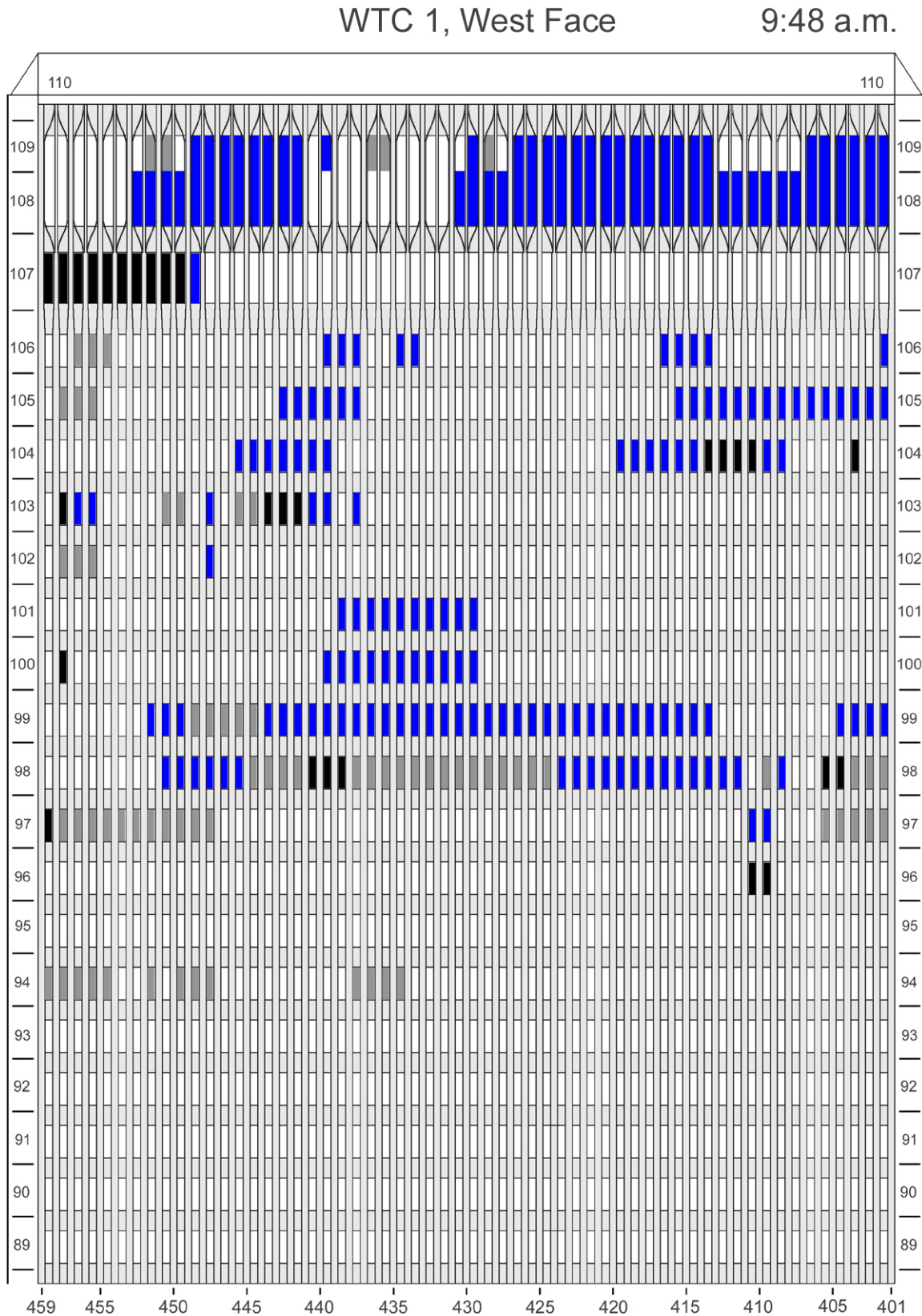
Figure F-44. Diagram of the west face of WTC 1 for floors 89 to 110 at 9:48 a.m. showing windows where smoke was observed and those that were hidden from view.
