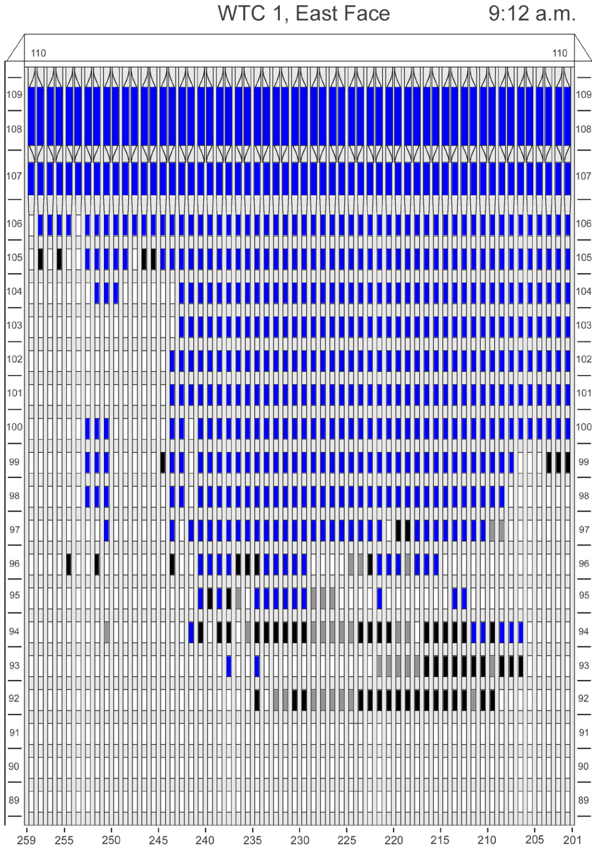
Figure D-16. Diagram of the east face of WTC 1 for floors 89 to 110 at 9:12 a.m. showing windows where smoke was observed and those that were hidden from view.
