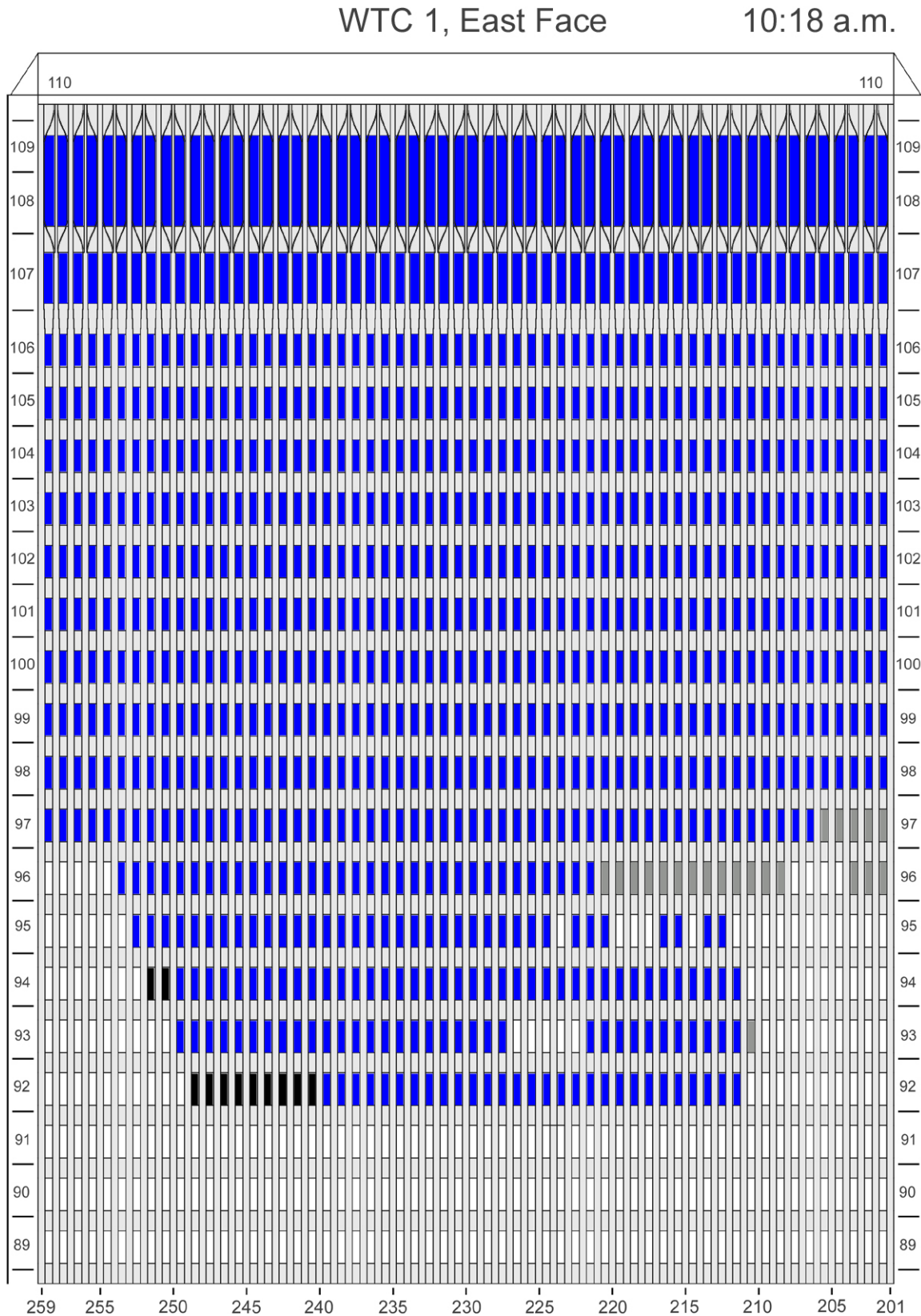
Figure D-46. Diagram of the east face of WTC 1 for floors 89 to 110 at 10:18 a.m. showing windows where smoke was observed and those that were hidden from view.
