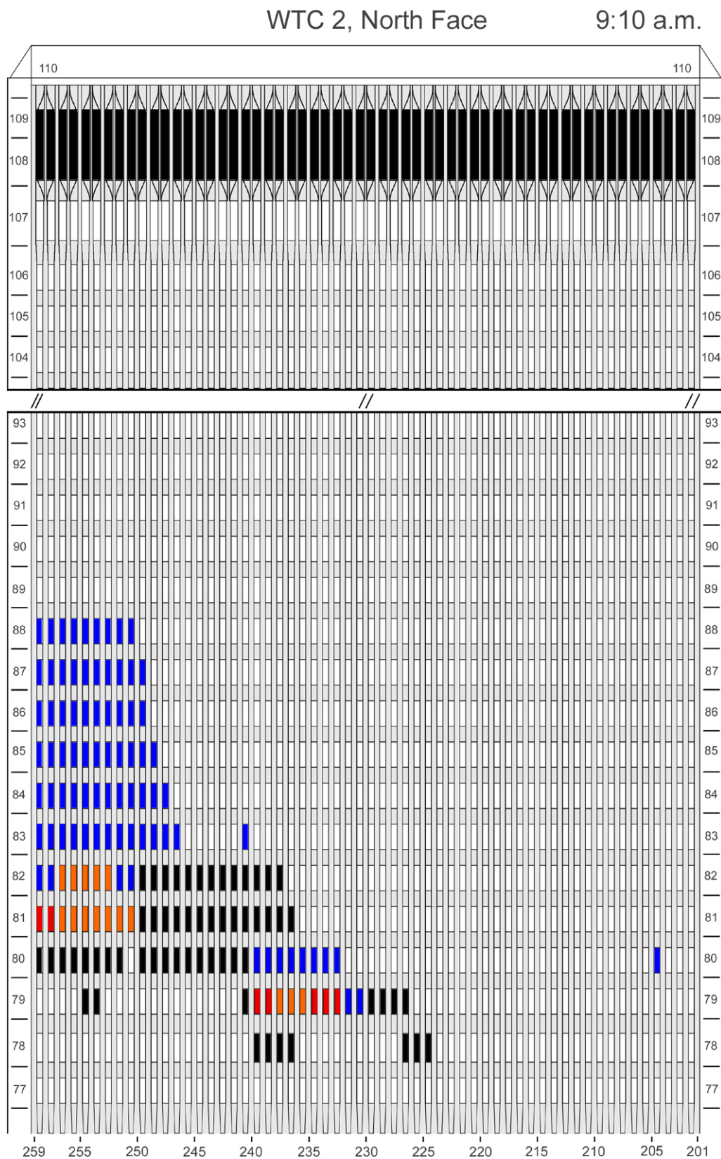
Figure G-9. Diagram of the north face of WTC 2 for floors 77 to 93 and floors 104 to 110 at 9:10 a.m. showing the condition of windows and locations of fires.
