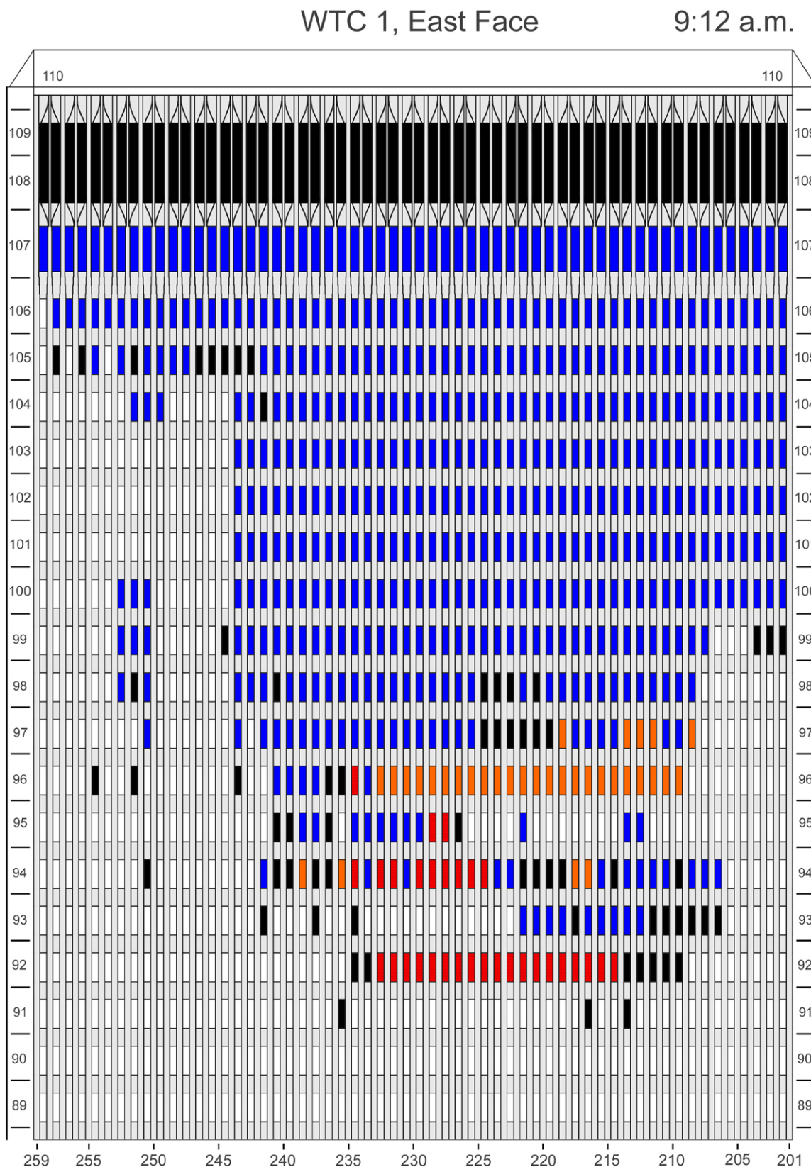
Figure D-15. Diagram of the east face of WTC 1 for floors 89 to 110 at 9:12 a.m. showing the condition of windows and locations of fires.
