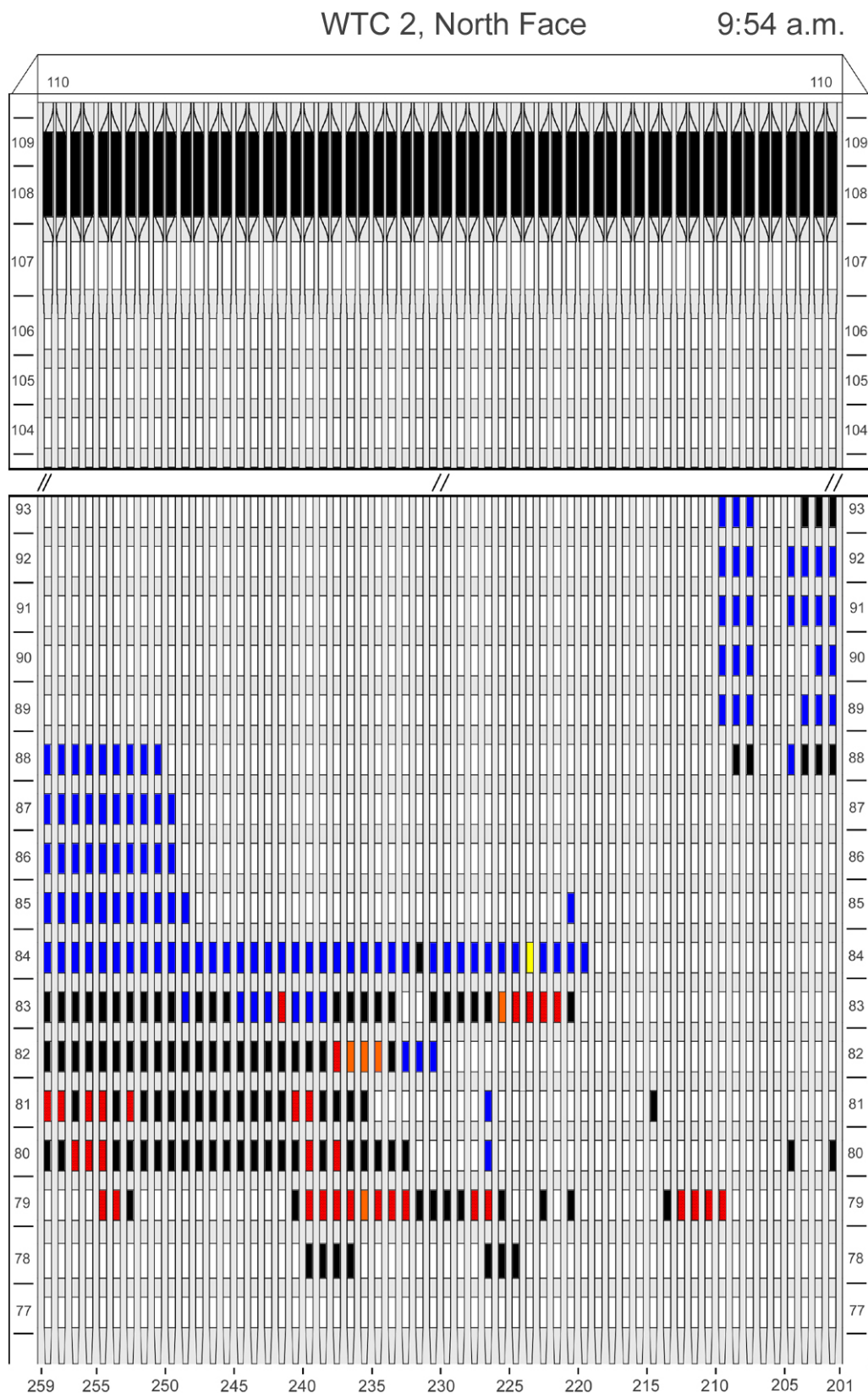
Figure G-53. Diagram of the north face of WTC 2 for floors 77 to 93 and floors 104 to 110 at 9:54 a.m. showing the condition of windows and locations of fires.
