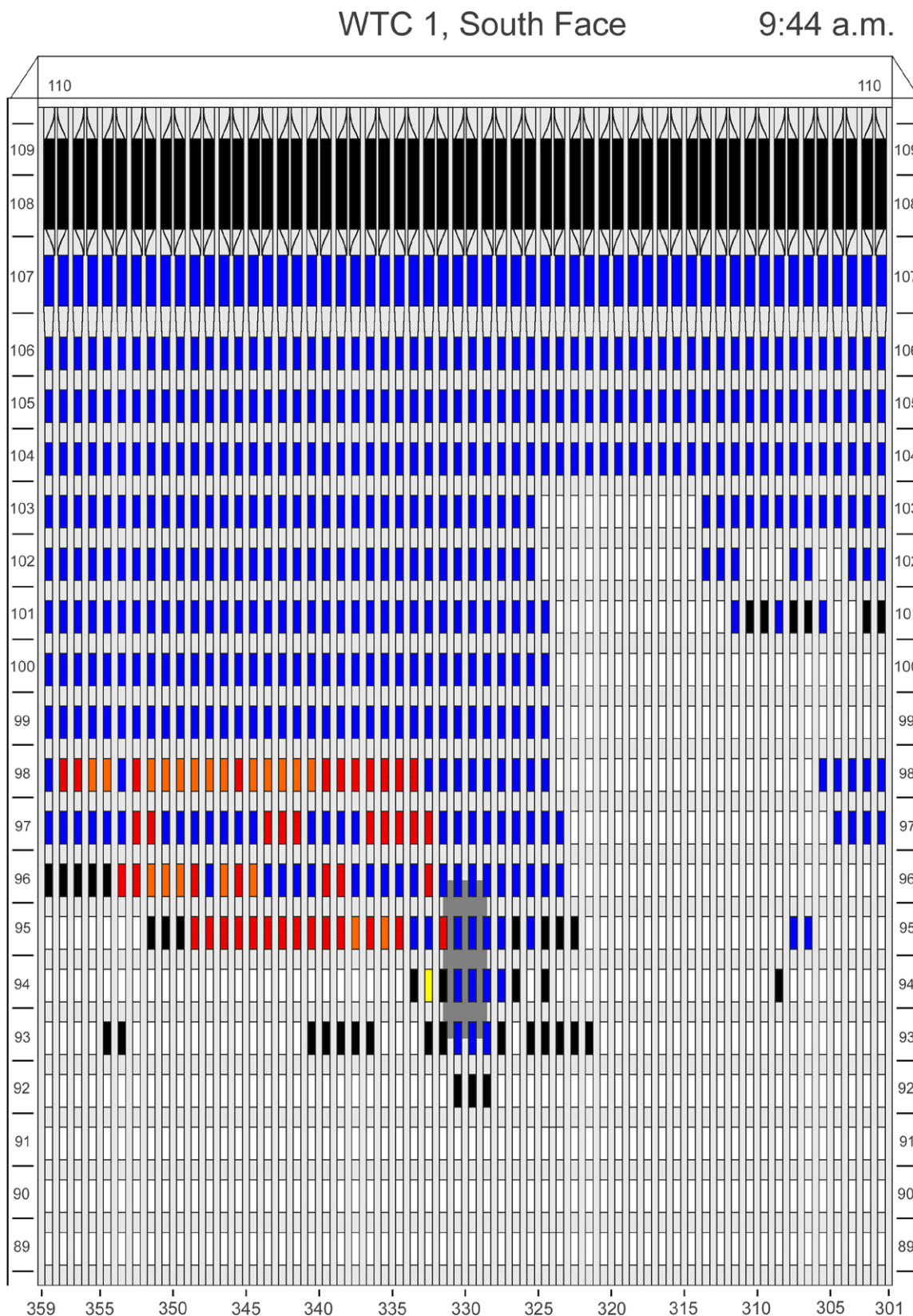
Figure E-29. Diagram of the south face of WTC 1 for floors 89 to 110 at 9:44 a.m. showing the condition of windows and locations of fires.
