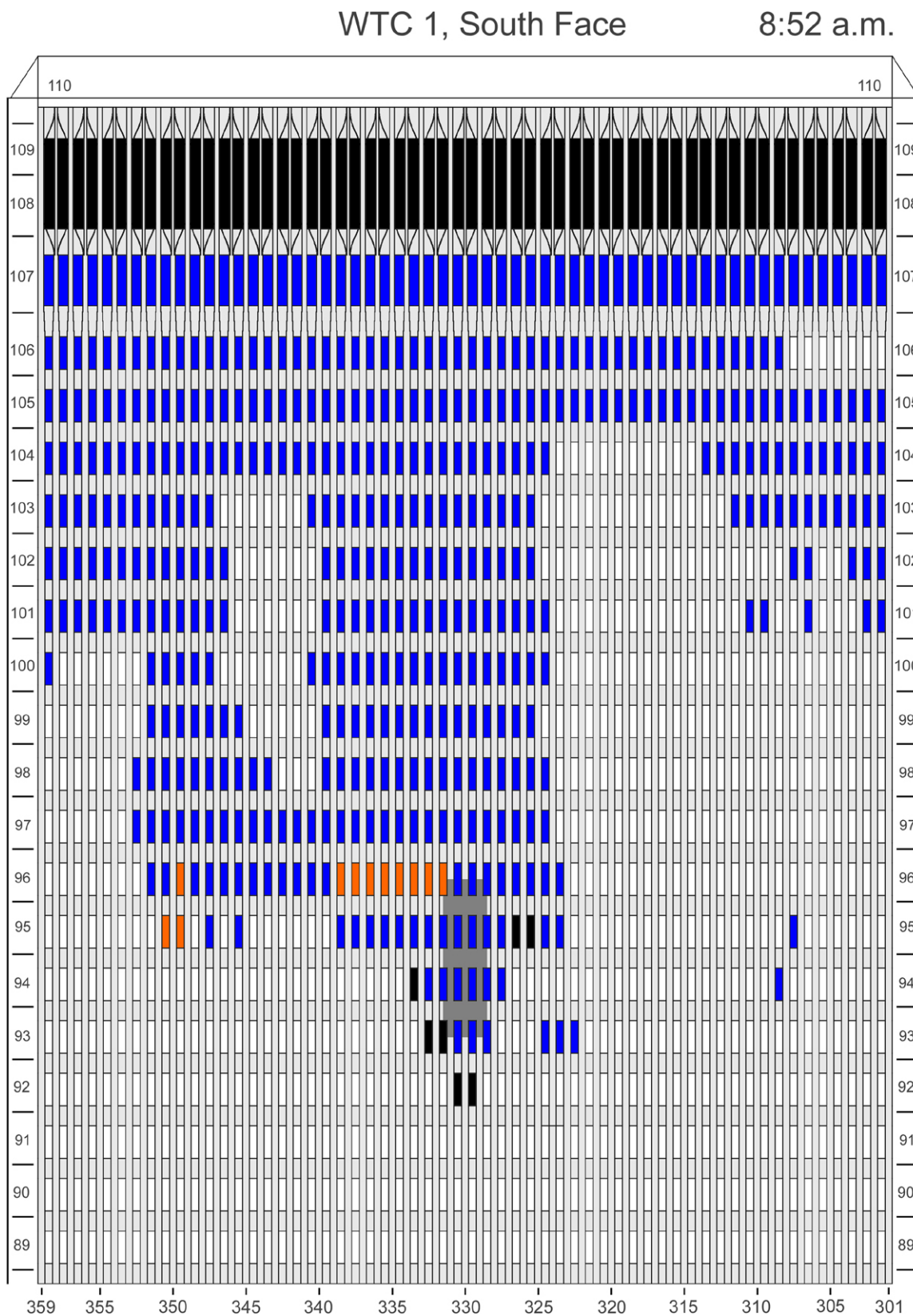
Figure E-3. Diagram of the south face of WTC 1 for floors 89 to 110 at 8:52 a.m. showing the condition of windows and locations of fires.
