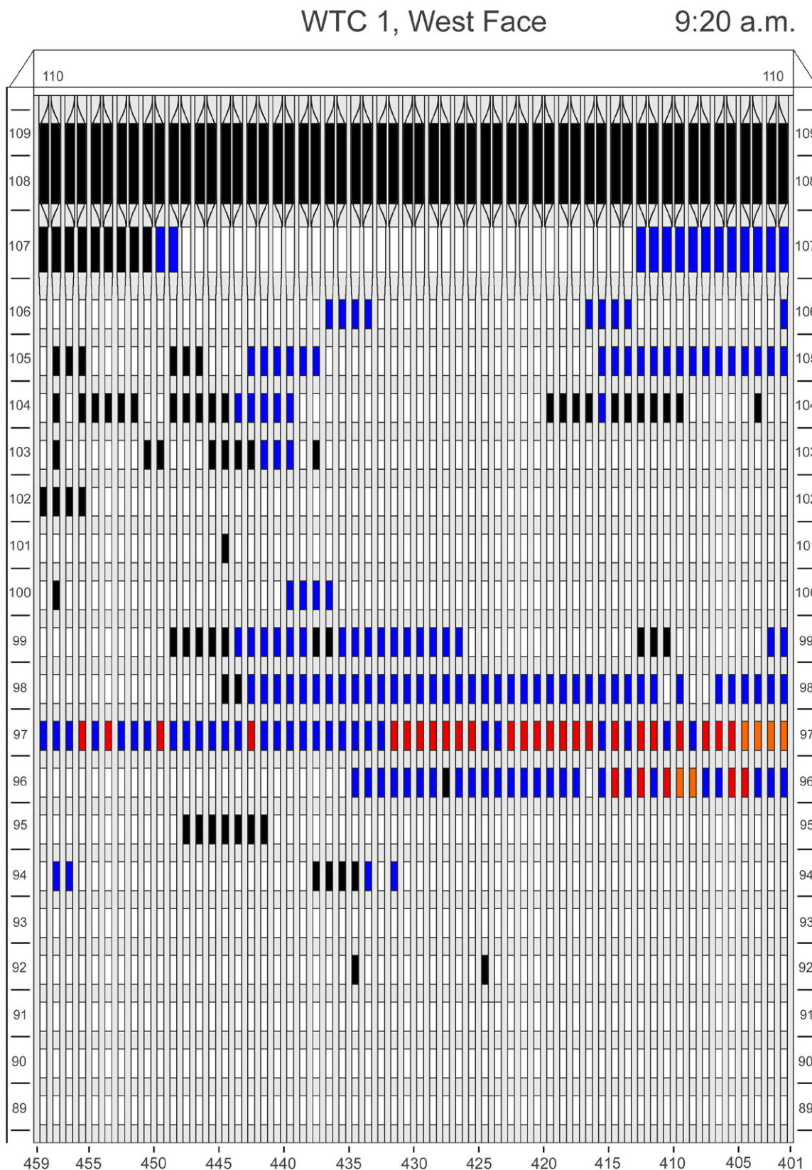
Figure F-29. Diagram of the west face of WTC 1 for floors 89 to 110 at 9:20 a.m. showing the condition of windows and locations of fires.
