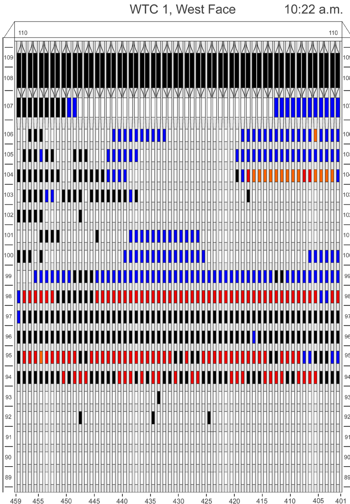
Figure F-59. Diagram of the west face of WTC 1 for floors 89 to 110 at 10:22 a.m. showing the condition of windows and locations of fires.
