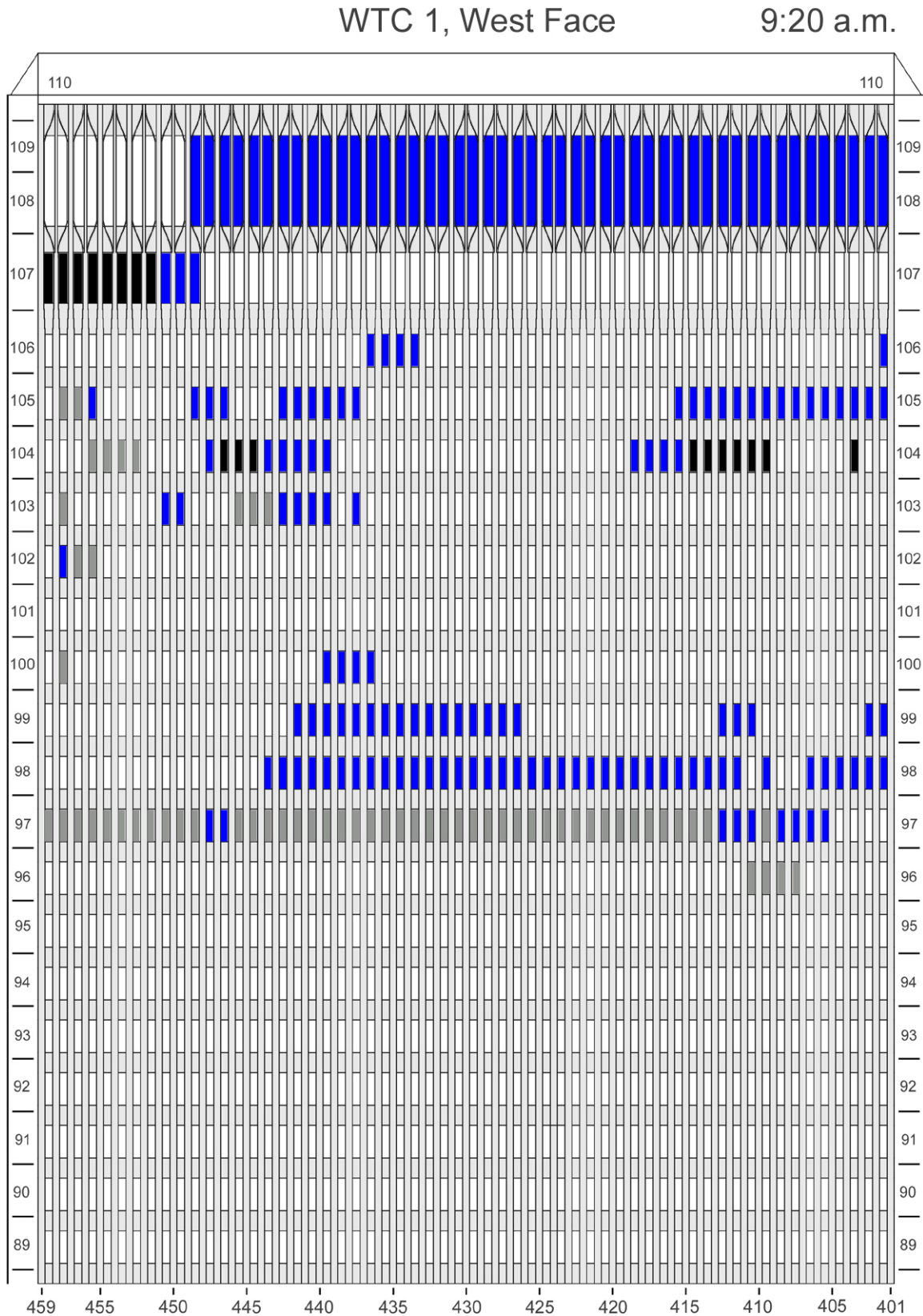
Figure F-30. Diagram of the west face of WTC 1 for floors 89 to 110 at 9:20 a.m. showing windows where smoke was observed and those that were hidden from view.
