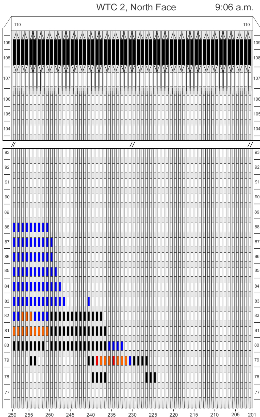
Figure G-5. Diagram of the north face of WTC 2 for floors 77 to 93 and floors 104 to 110 at 9:06 a.m. showing the condition of windows and locations of fires.
