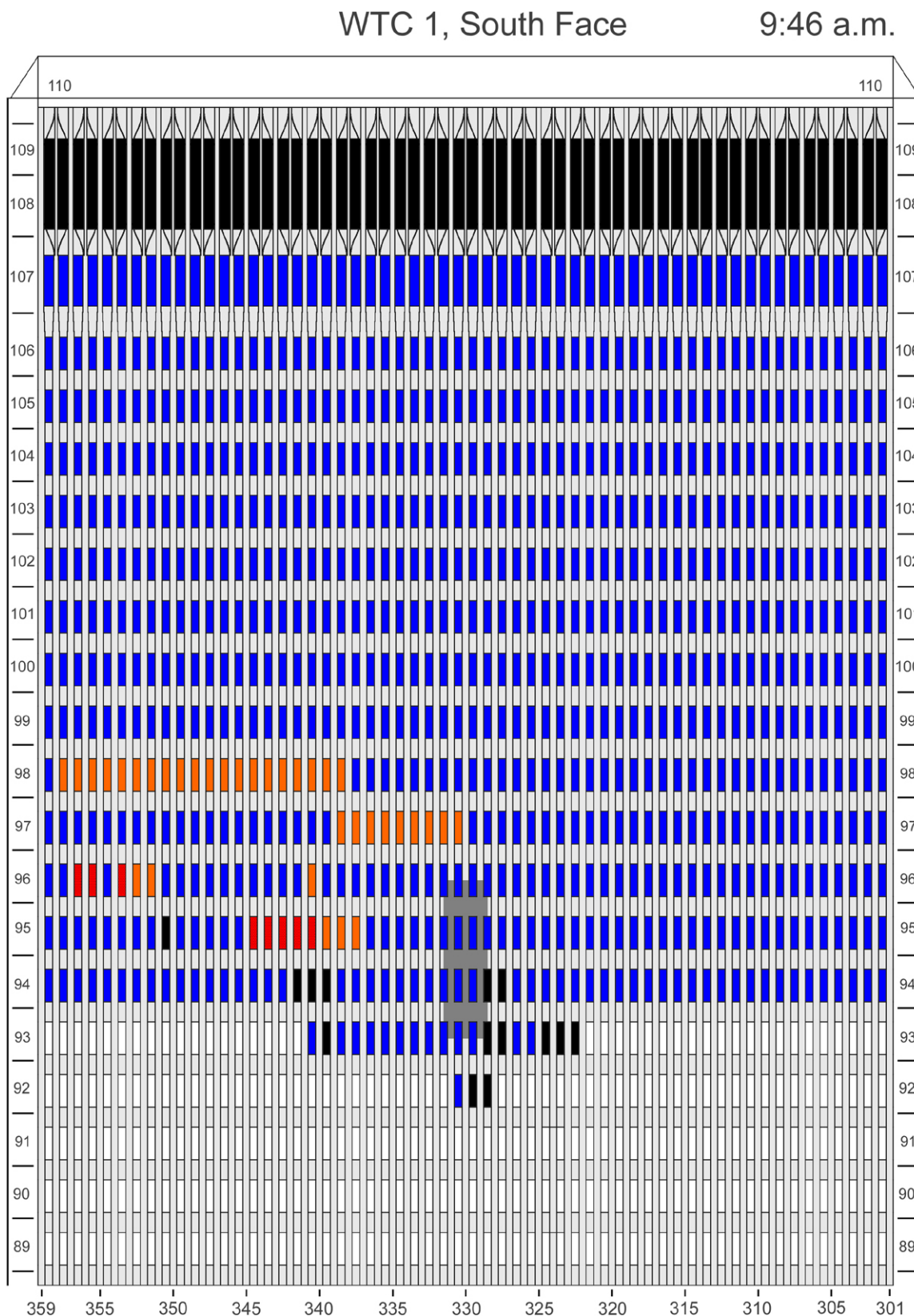
Figure E-31. Diagram of the south face of WTC 1 for floors 89 to 110 at 9:46 a.m. showing the condition of windows and locations of fires.
