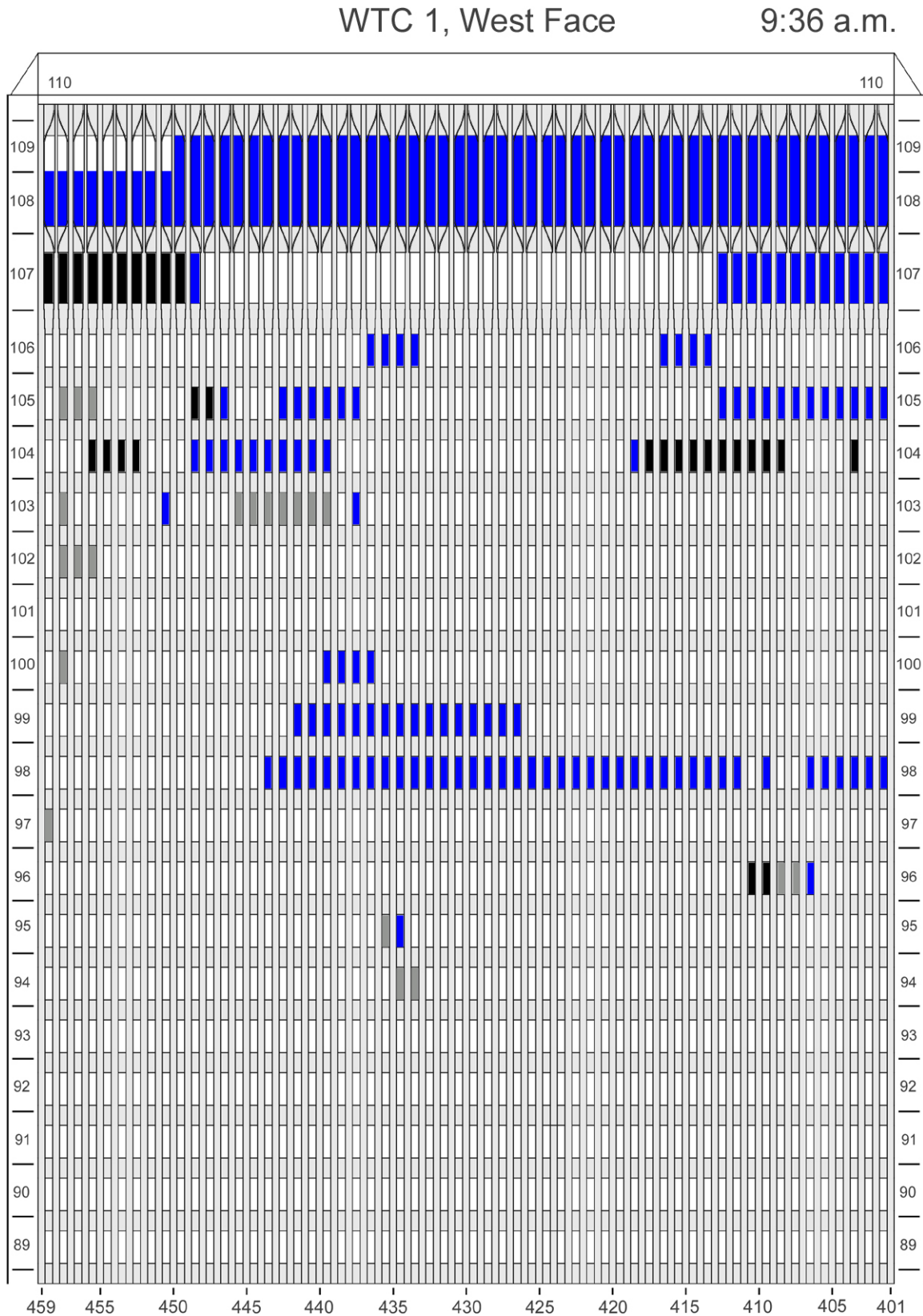
Figure F-36. Diagram of the west face of WTC 1 for floors 89 to 110 at 9:36 a.m. showing windows where smoke was observed and those that were hidden from view.
