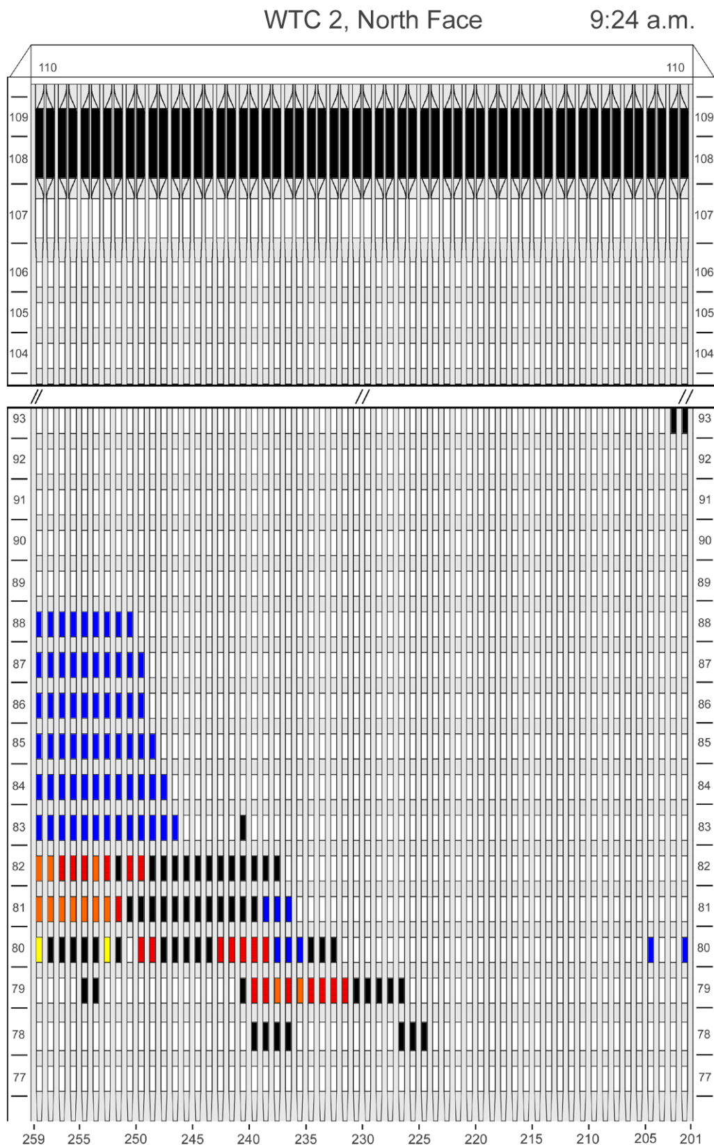
Figure G-23. Diagram of the north face of WTC 2 for floors 77 to 93 and floors 104 to 110 at 9:24 a.m. showing the condition of windows and locations of fires.
