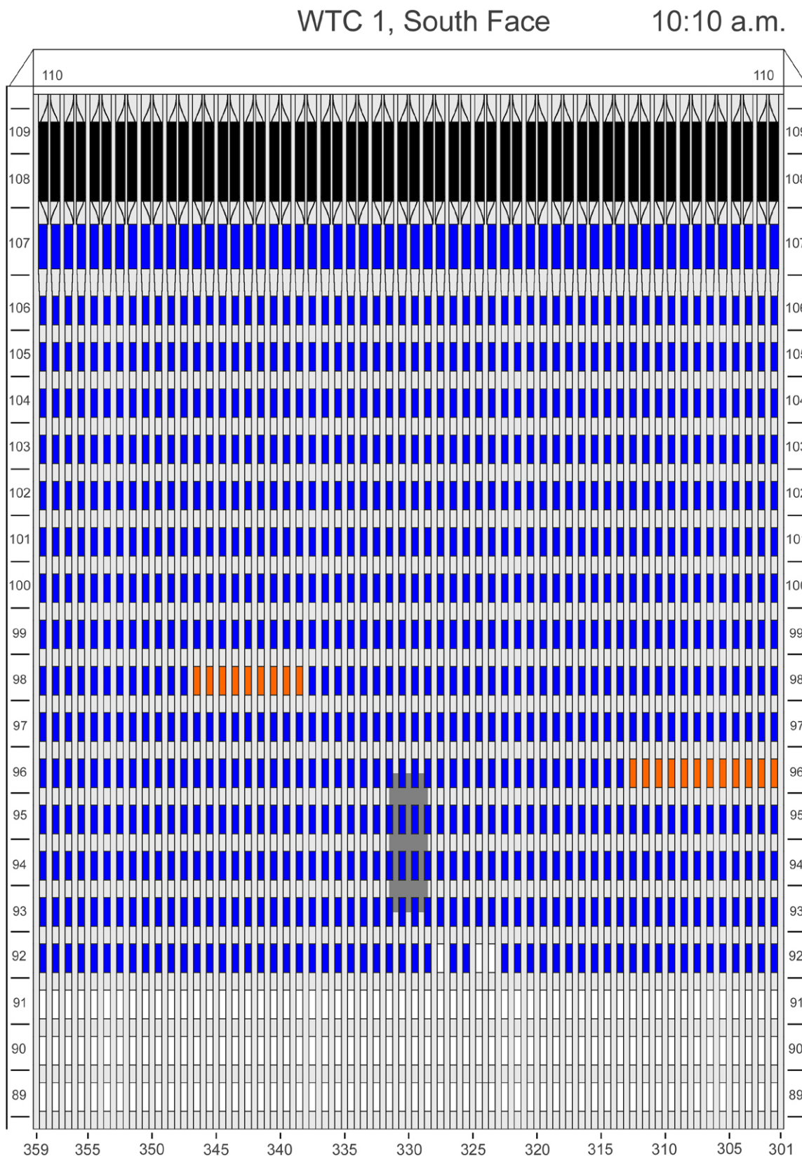
Figure E-39. Diagram of the south face of WTC 1 for floors 89 to 110 at 10:10 a.m. showing the condition of windows and locations of fires.
