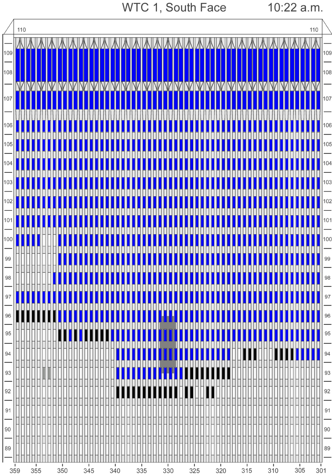
Figure E- 48. Diagram of the south face of WTC 1 for floors 89 to 110 at 10:22 a.m. showing windows where smoke was observed and those that were hidden from view.
