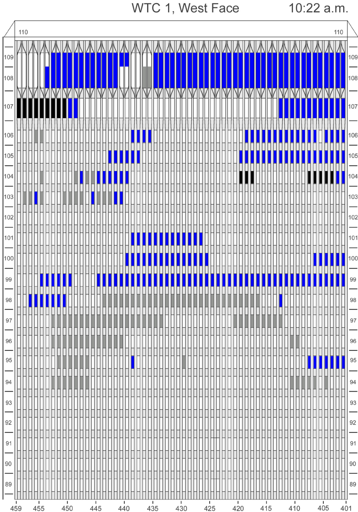
Figure F-60. Diagram of the west face of WTC 1 for floors 89 to 110 at 10:22 a.m. showing windows where smoke was observed and those that were hidden from view.
