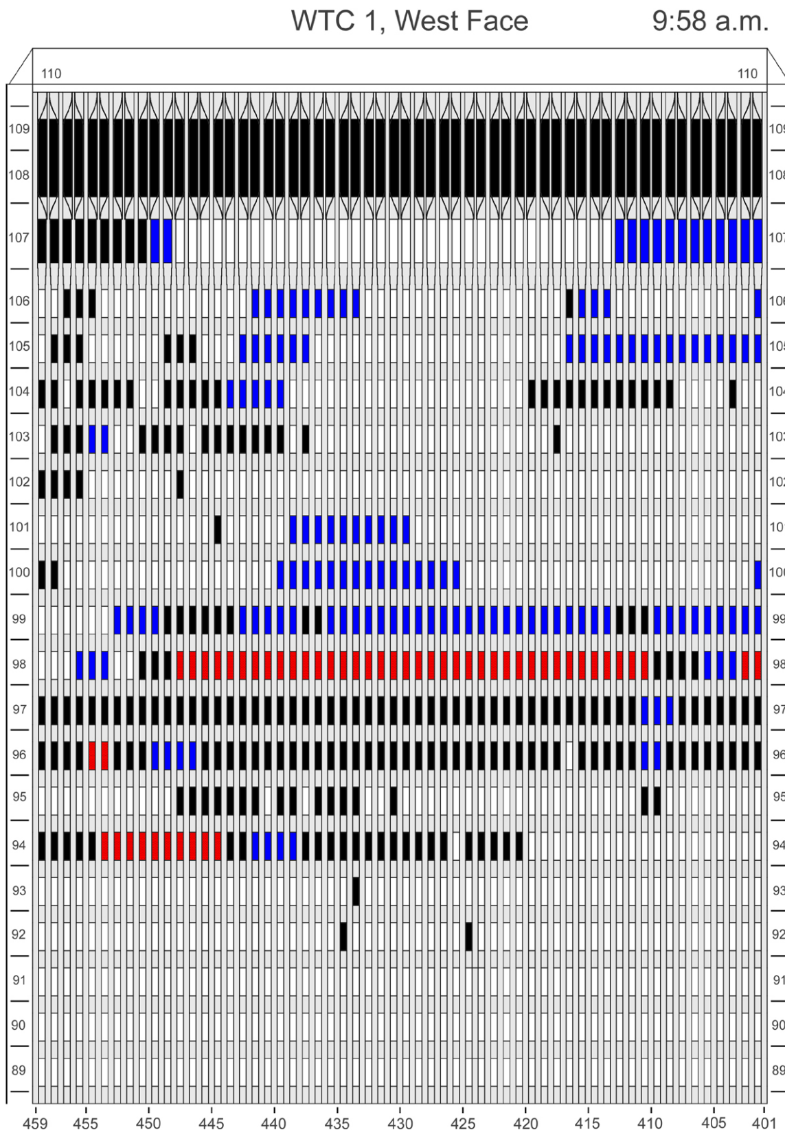
Figure F-49. Diagram of the west face of WTC 1 for floors 89 to 110 at 9:58 a.m. showing the condition of windows and locations of fires.
