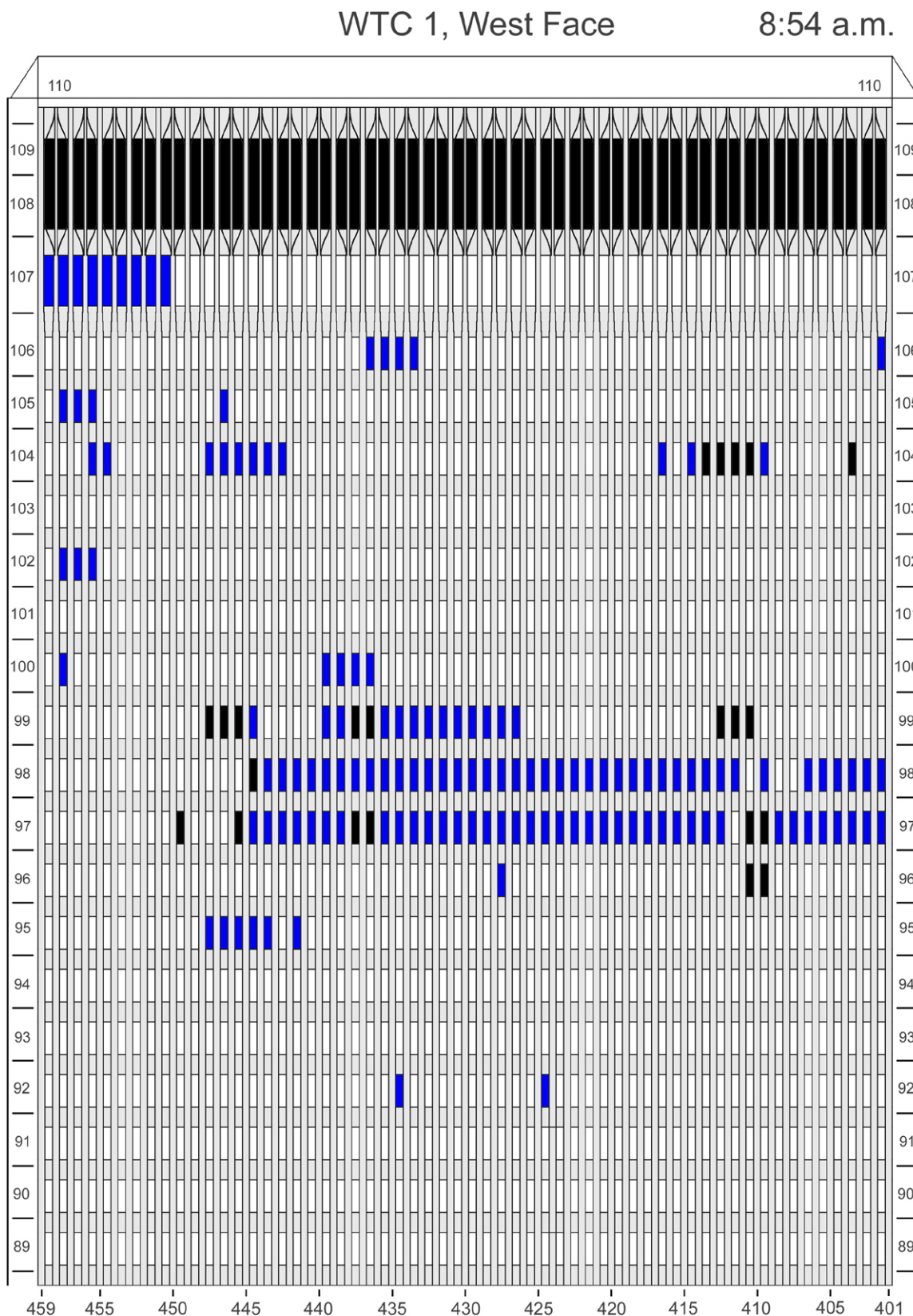
Figure F-9. Diagram of the west face of WTC 1 for floors 89 to 110 at 8:54 a.m. showing the condition of windows and locations of fires.
