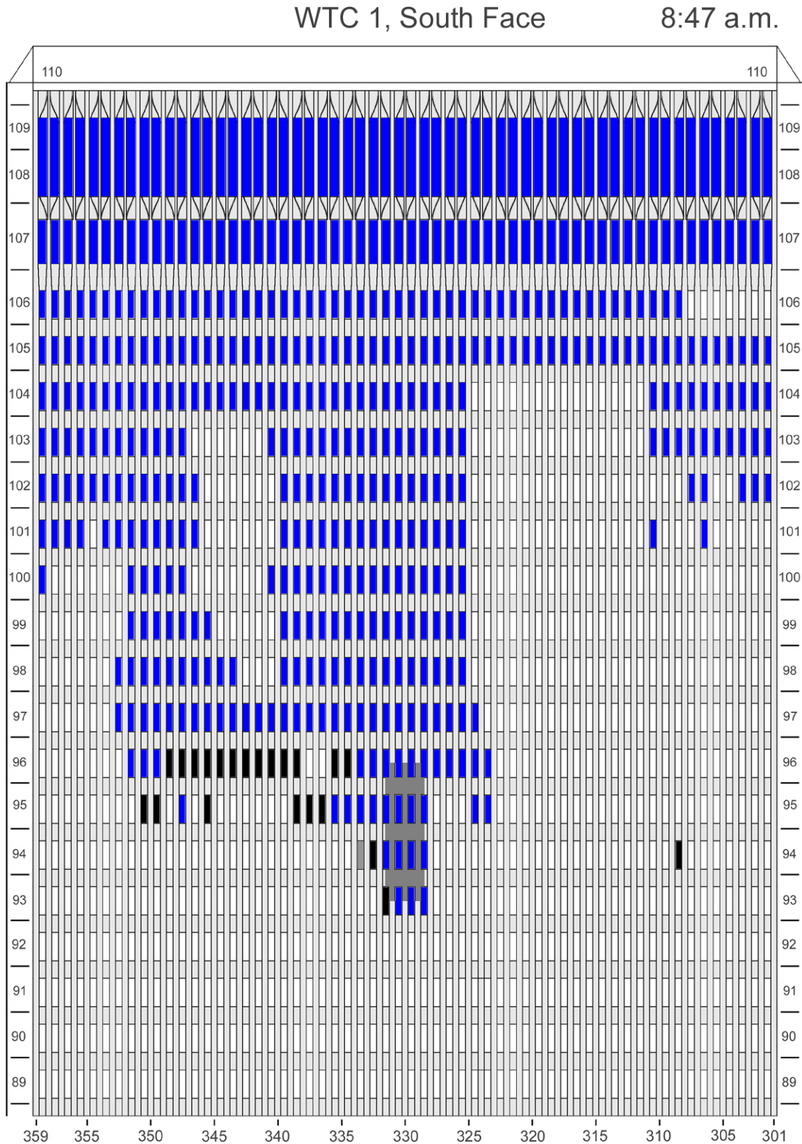
Figure E-2. Diagram of the south face of WTC 1 for floors 89 to 110 at 8:47 a.m. showing windows where smoke was observed and those that were hidden from view.
