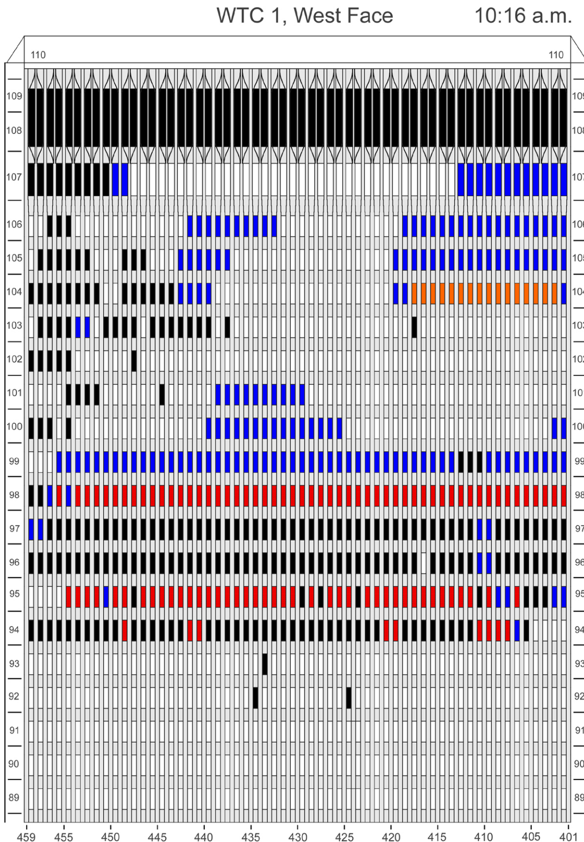
Figure F-55. Diagram of the west face of WTC 1 for floors 89 to 110 at 10:16 a.m. showing the condition of windows and locations of fires.
