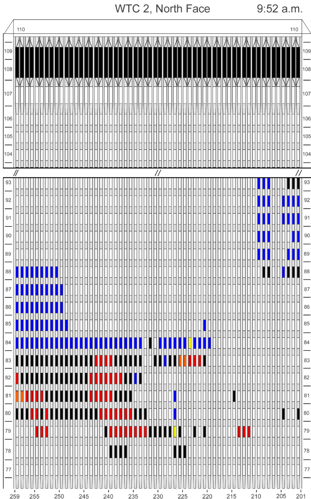
Figure G-51. Diagram of the north face of WTC 2 for floors 77 to 93 and floors 104 to 110 at 9:52 a.m. showing the condition of windows and locations of fires.
