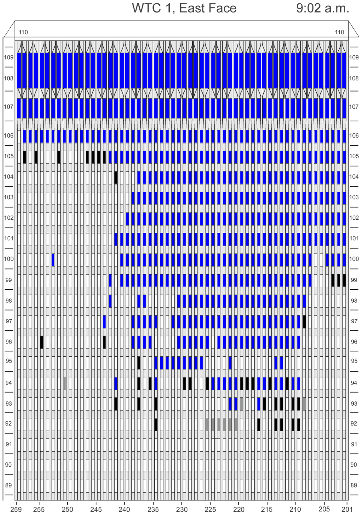
Figure D-12. Diagram of the east face of WTC 1 for floors 89 to 110 at 9:02 a.m. showing windows where smoke was observed and those that were hidden from view.
