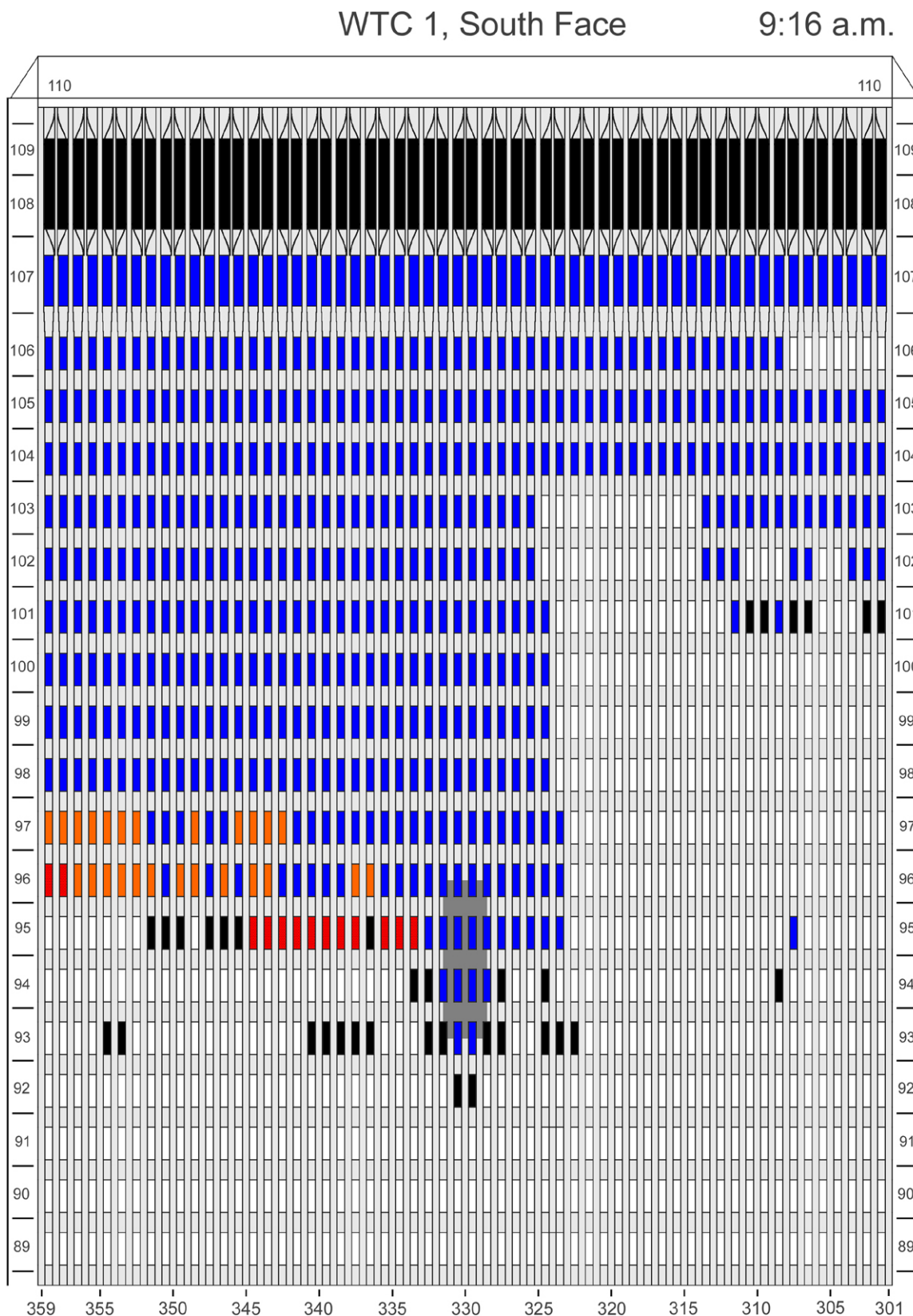
Figure E-15. Diagram of the south face of WTC 1 for floors 89 to 110 at 9:16 a.m. showing the condition of windows and locations of fires.
