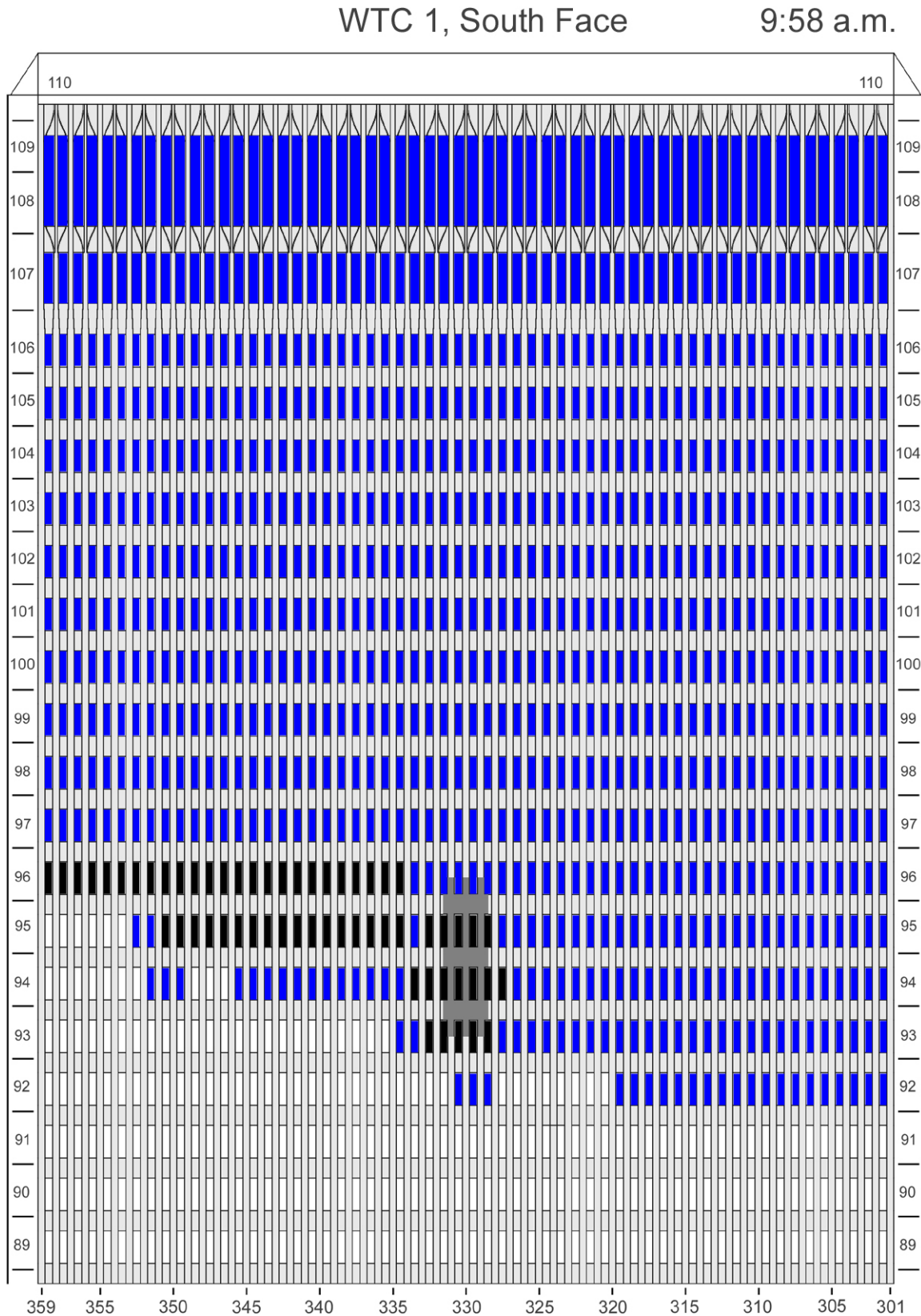
Figure E-36. Diagram of the south face of WTC 1 for floors 89 to 110 at 9:58 a.m. showing windows where smoke was observed and those that were hidden from view.
