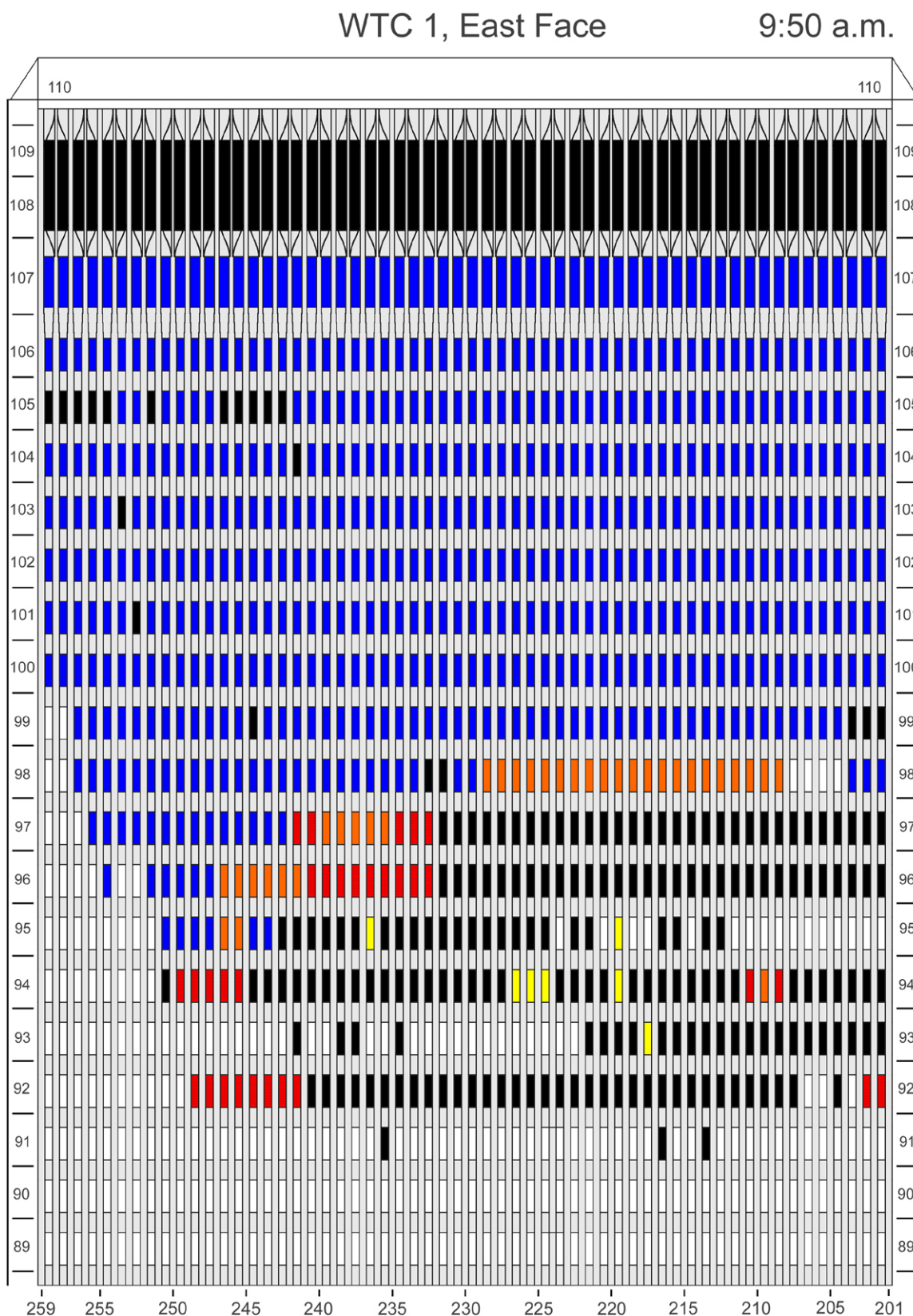
Figure D-31. Diagram of the east face of WTC 1 for floors 89 to 110 at 9:50 a.m. showing the condition of windows and locations of fires.
