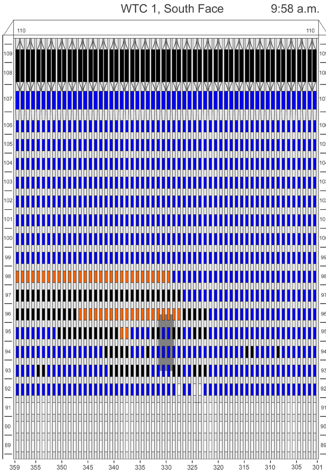
Figure E-35. Diagram of the south face of WTC 1 for floors 89 to 110 at 9:58 a.m. showing the condition of windows and locations of fires.
