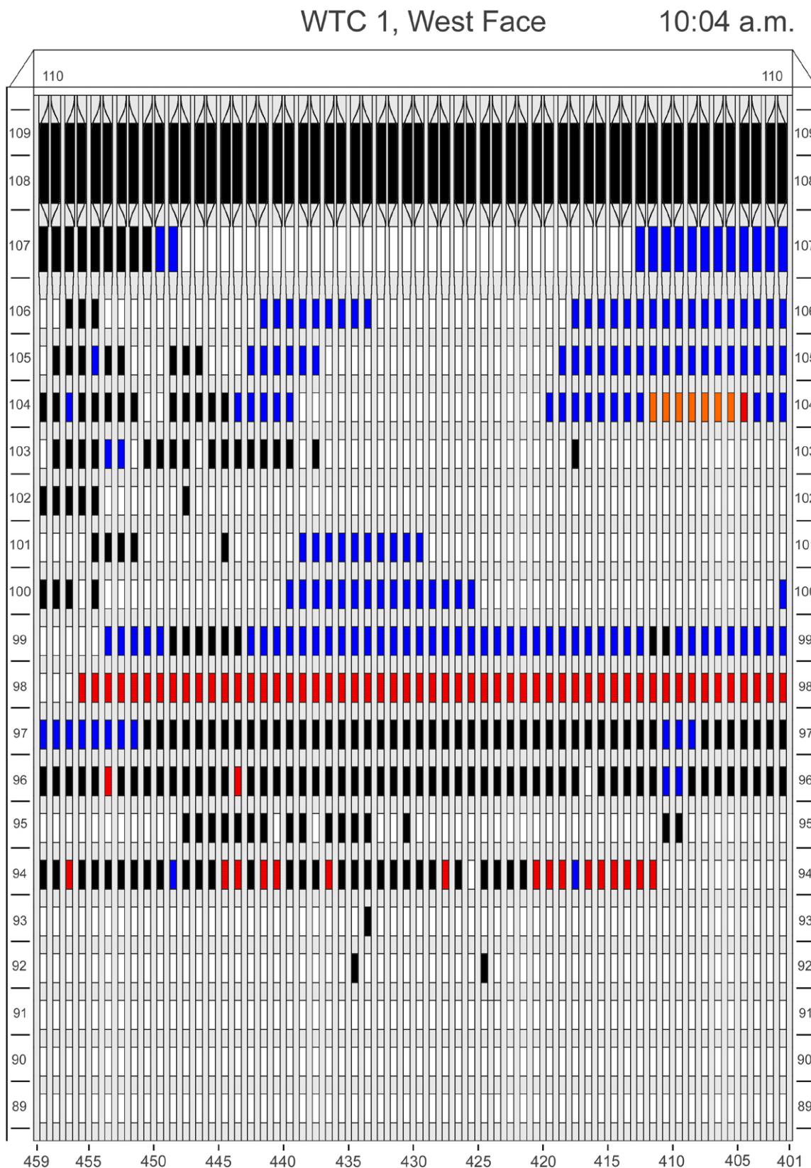
Figure F-51. Diagram of the west face of WTC 1 for floors 89 to 110 at 10:04 a.m. showing the condition of windows and locations of fires.
