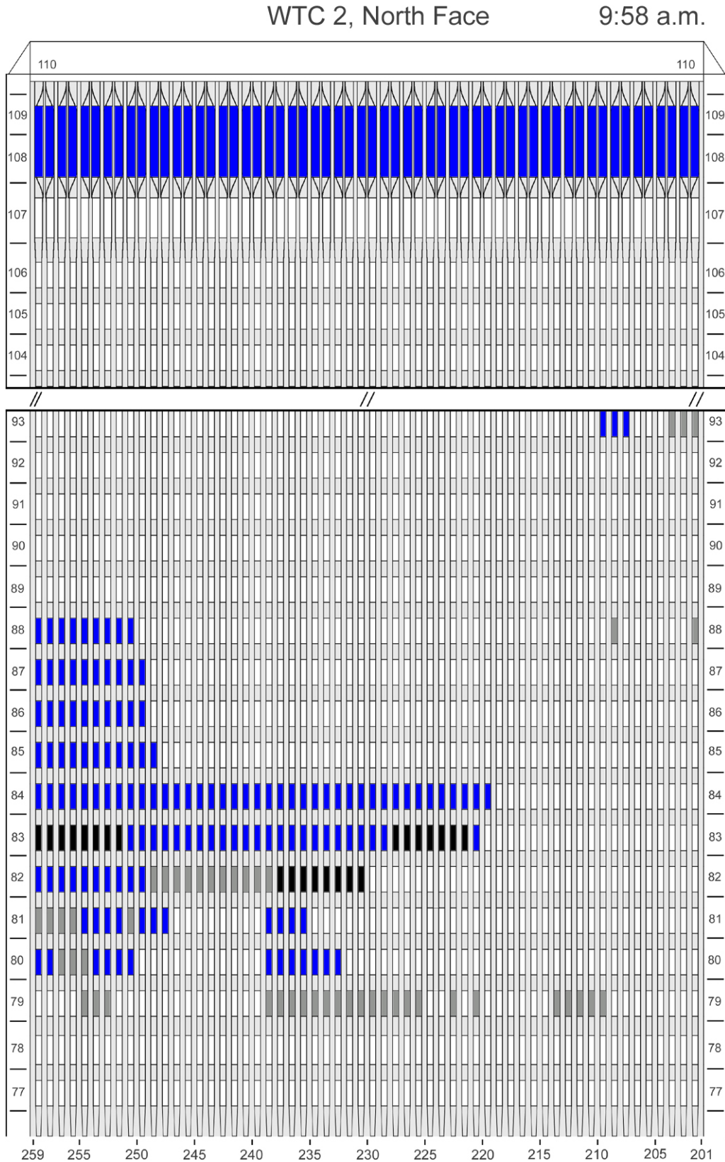
Figure G-58. Diagram of the north face of WTC 2 for floors 77 to 93 and floors 104 to 110 at 9:58 a.m. showing windows where smoke was observed and those hidden from view.
