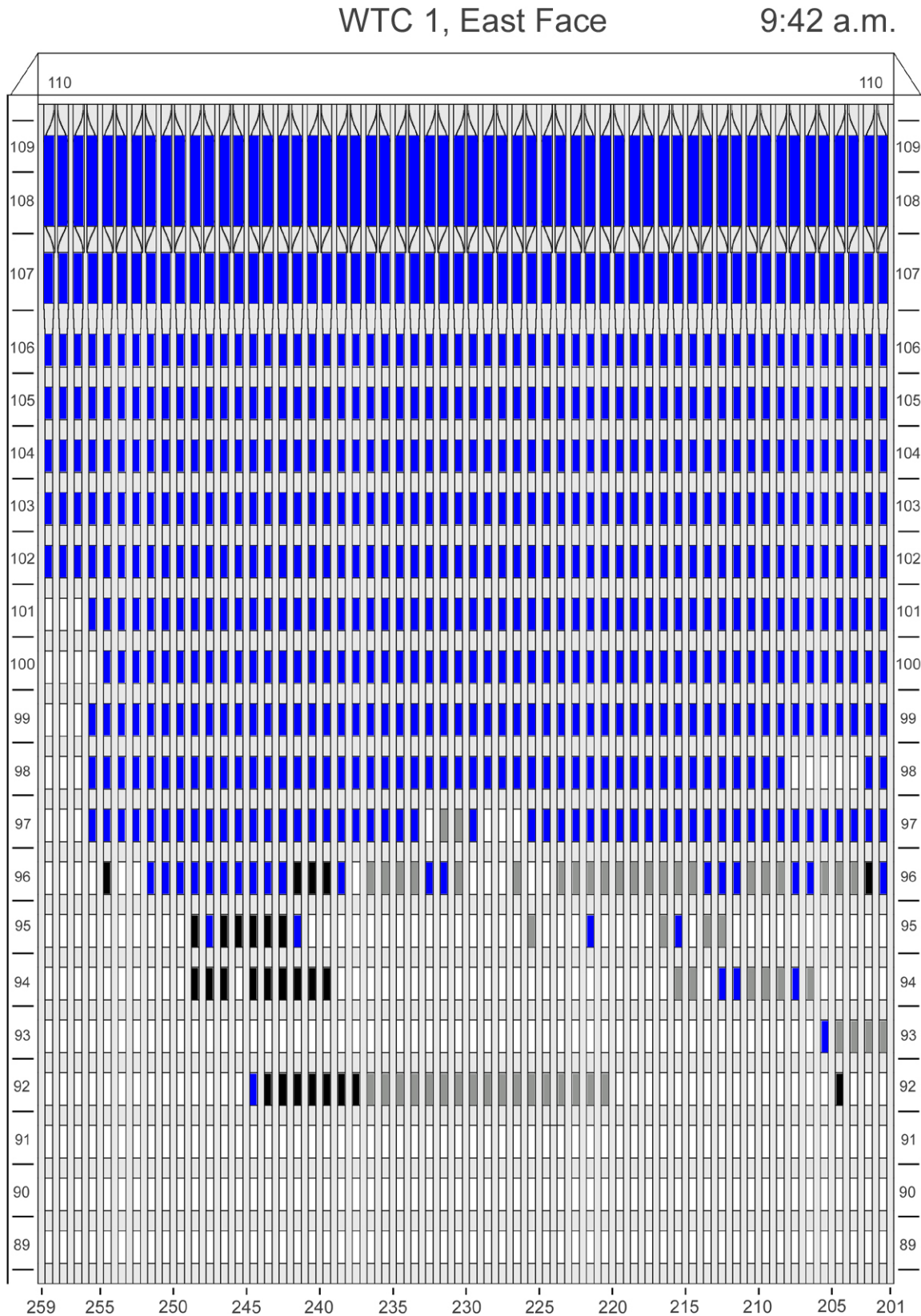
Figure D-28. Diagram of the east face of WTC 1 for floors 89 to 110 at 9:42 a.m. showing windows where smoke was observed and those that were hidden from view.
