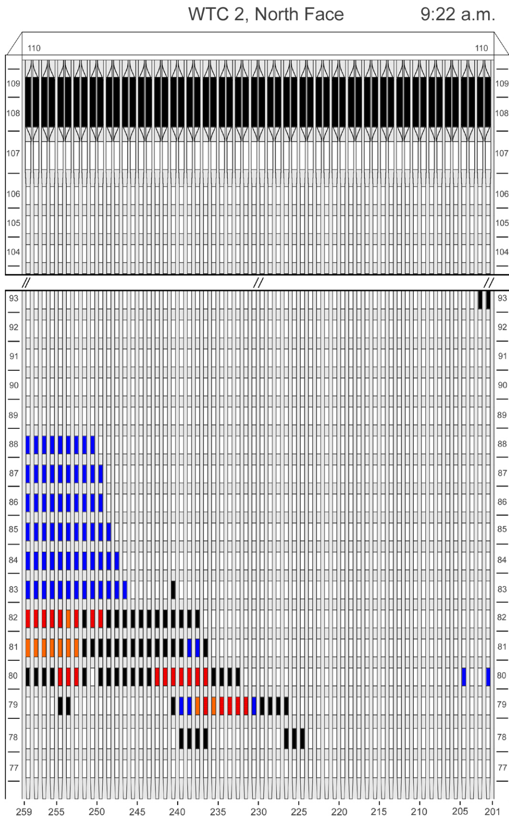
Figure G-21. Diagram of the north face of WTC 2 for floors 77 to 93 and floors 104 to 110 at 9:22 a.m. showing the condition of windows and locations of fires.
