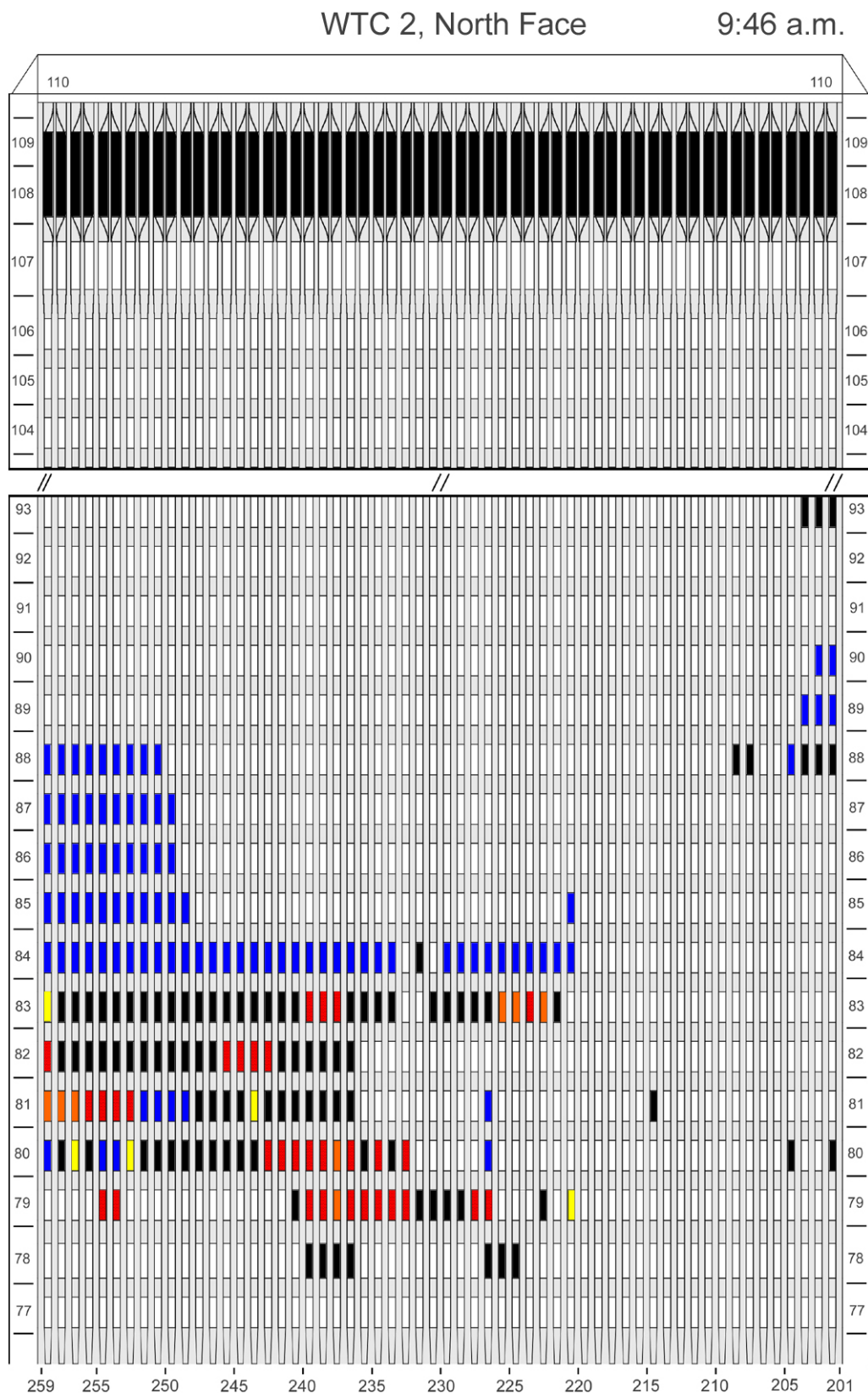
Figure G-45. Diagram of the north face of WTC 2 for floors 77 to 93 and floors 104 to 110 at 9:46 a.m. showing the condition of windows and locations of fires.
