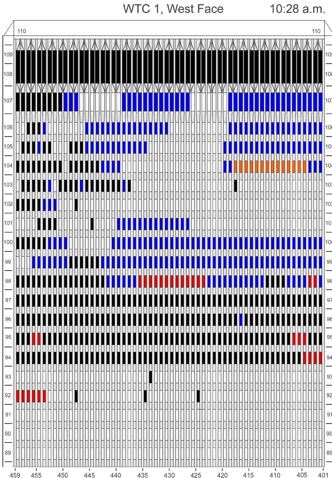
Figure F-61. Diagram of the west face of WTC 1 for floors 89 to 110 at 10:28 a.m. showing the condition of windows and locations of fires.
