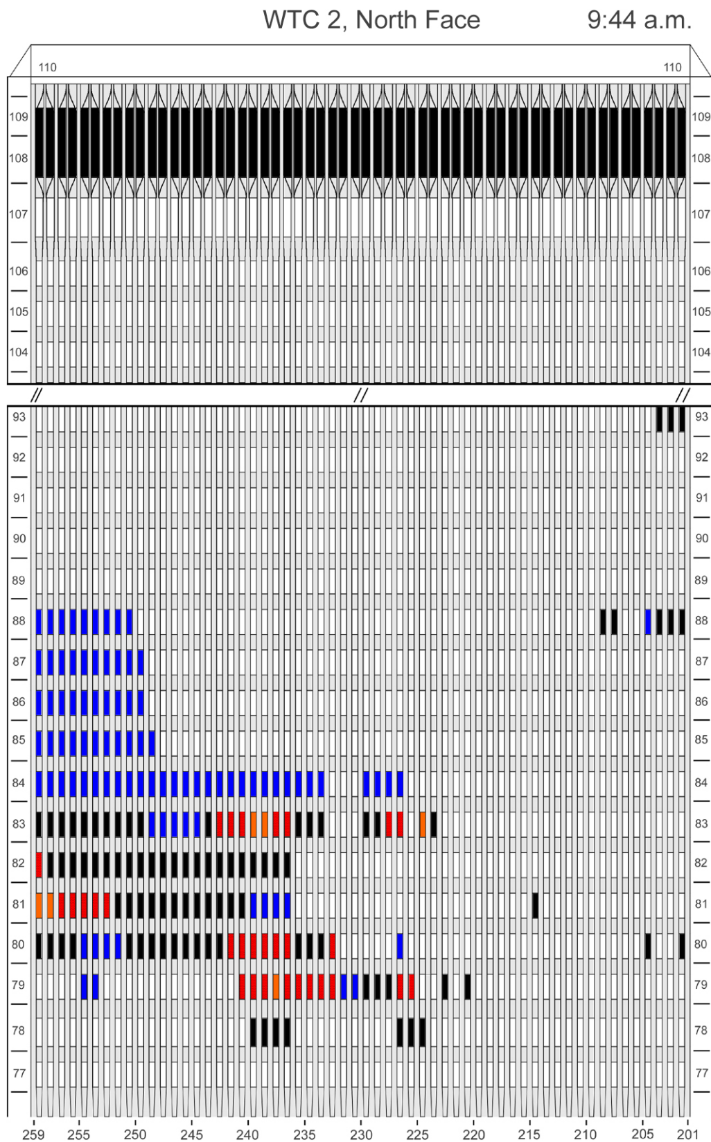
Figure G-43. Diagram of the north face of WTC 2 for floors 77 to 93 and floors 104 to 110 at 9:44 a.m. showing the condition of windows and locations of fires.
