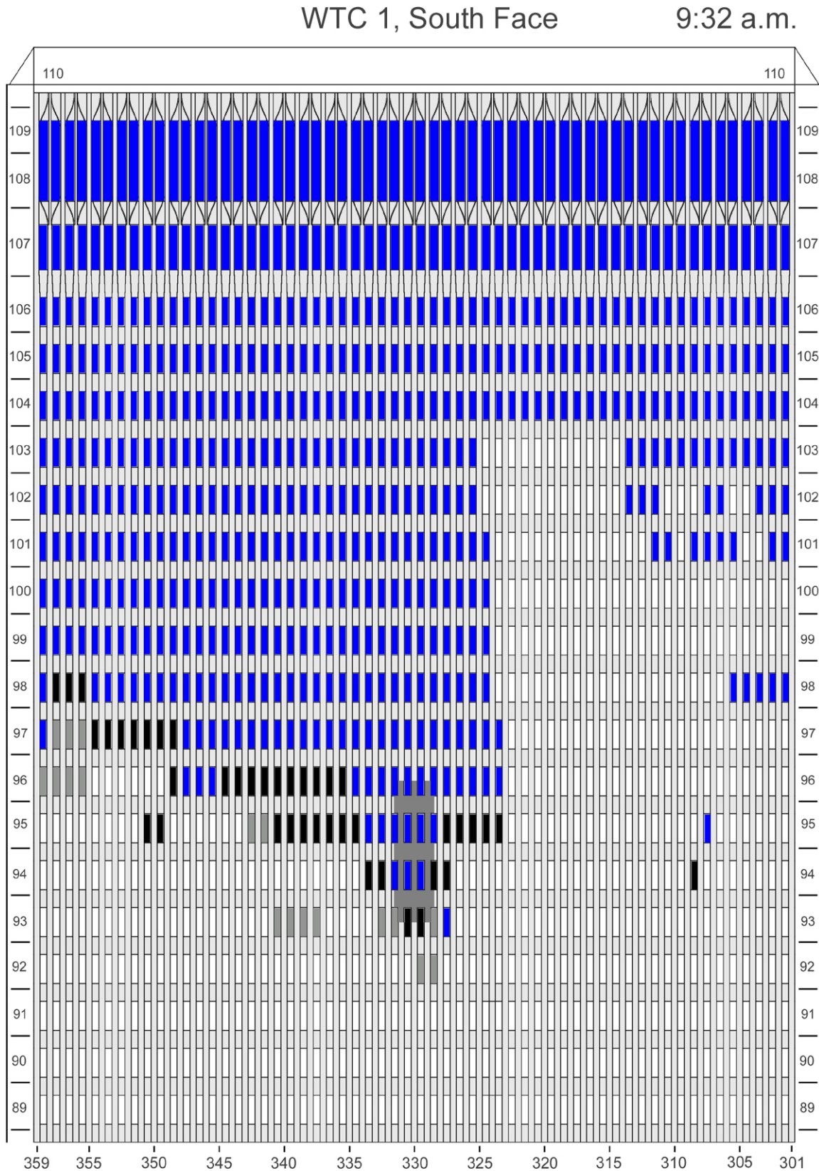
Figure E-22. Diagram of the south face of WTC 1 for floors 89 to 110 at 9:32 a.m. showing windows where smoke was observed and those that were hidden from view.
