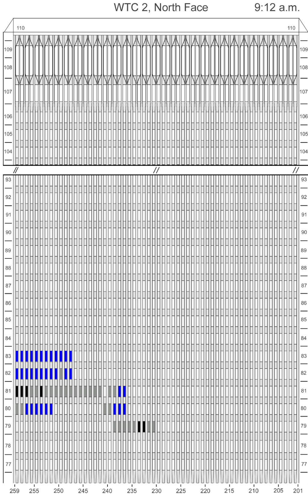
Figure G-12. Diagram of the north face of WTC 2 for floors 77 to 93 and floors 104 to 110 at 9:12 a.m. showing windows where smoke was observed and those hidden from view.
