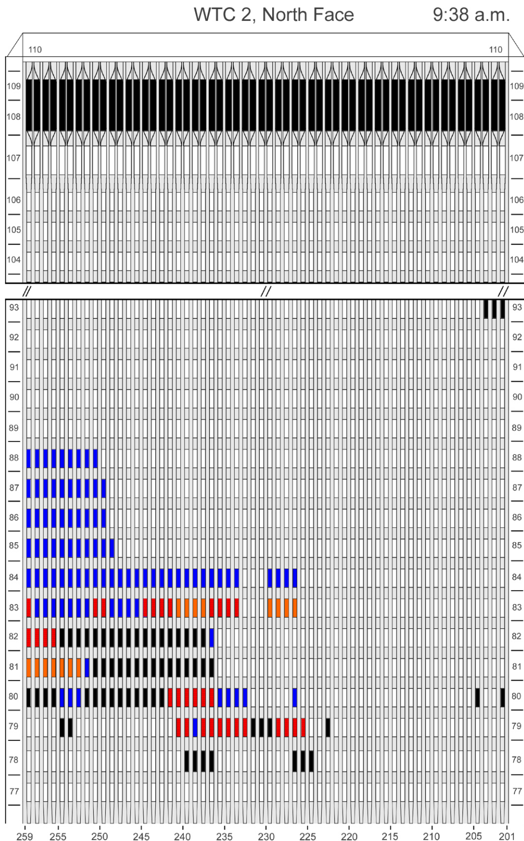
Figure G-37. Diagram of the north face of WTC 2 for floors 77 to 93 and floors 104 to 110 at 9:38 a.m. showing the condition of windows and locations of fires.
