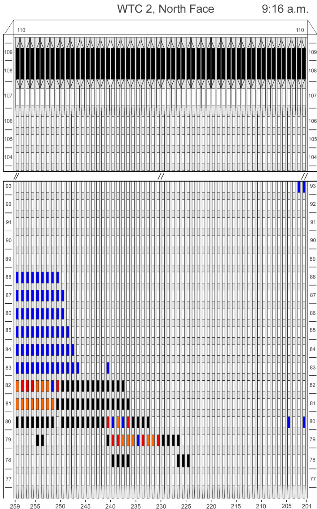
Figure G-15. Diagram of the north face of WTC 2 for floors 77 to 93 and floors 104 to 110 at 9:16 a.m. showing the condition of windows and locations of fires.
