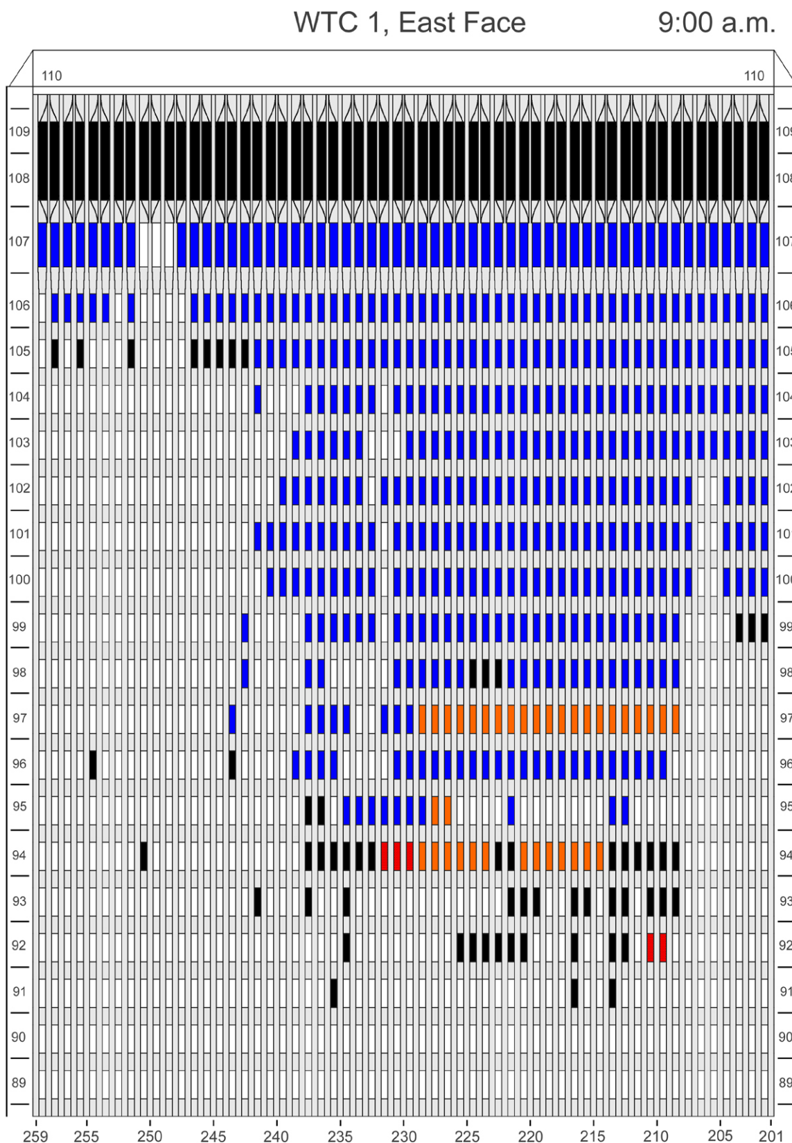
Figure D-9. Diagram of the east face of WTC 1 for floors 89 to 110 at 9:00 a.m. showing the condition of windows and locations of fires.
