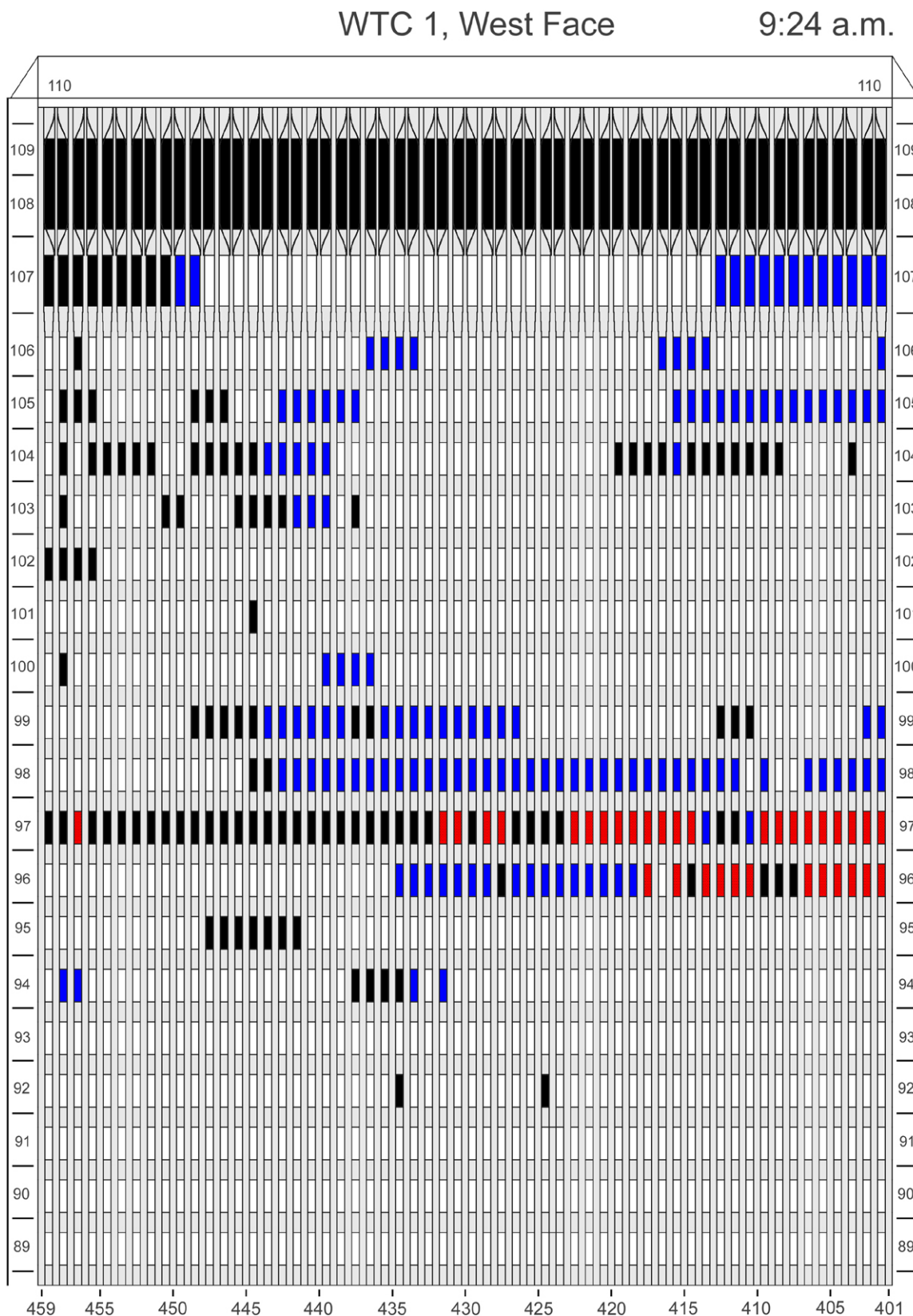
Figure F-31. Diagram of the west face of WTC 1 for floors 89 to 110 at 9:24 a.m. showing the condition of windows and locations of fires.
