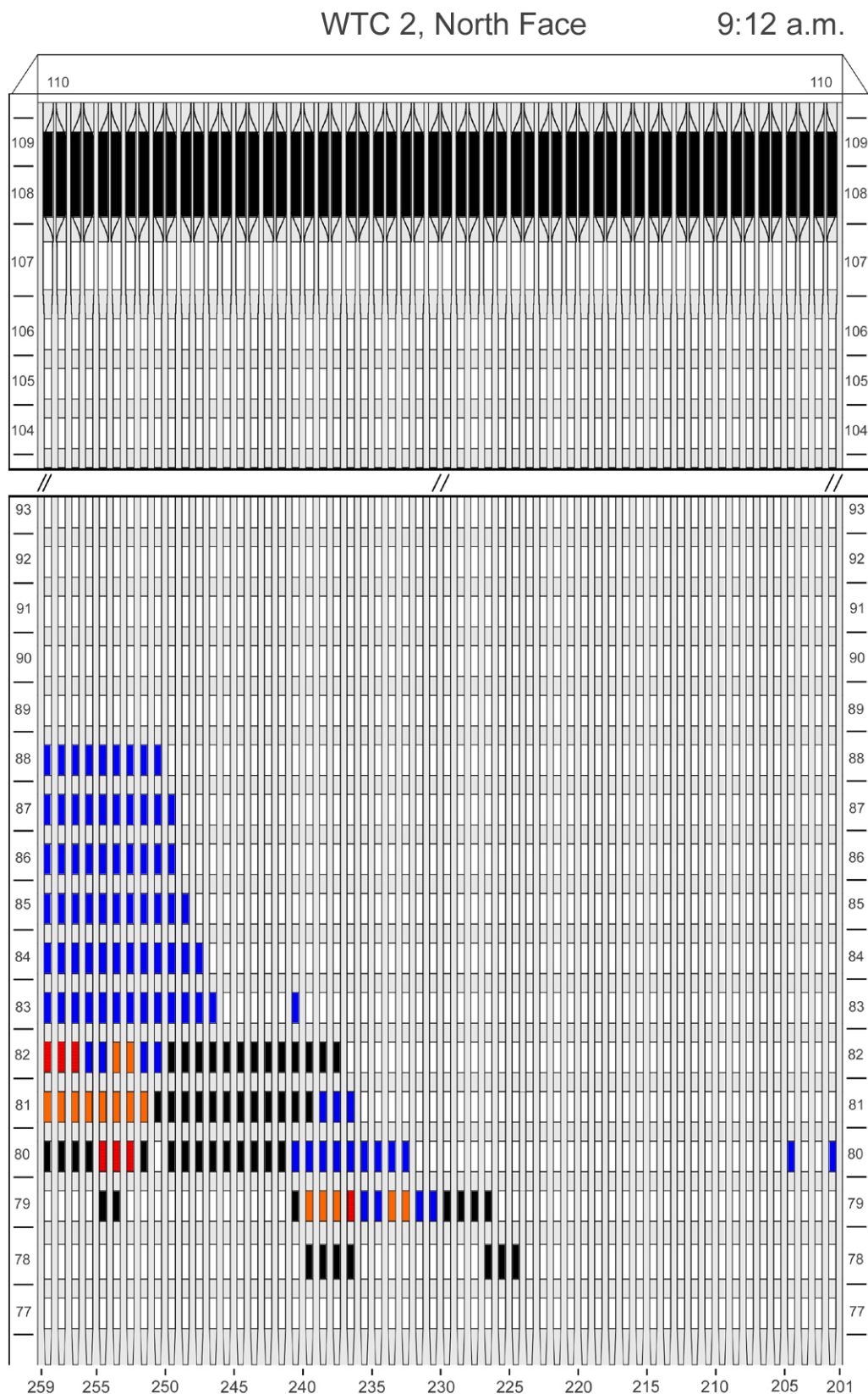
Figure G-11. Diagram of the north face of WTC 2 for floors 77 to 93 and floors 104 to 110 at 9:12 a.m. showing the condition of windows and locations of fires.
