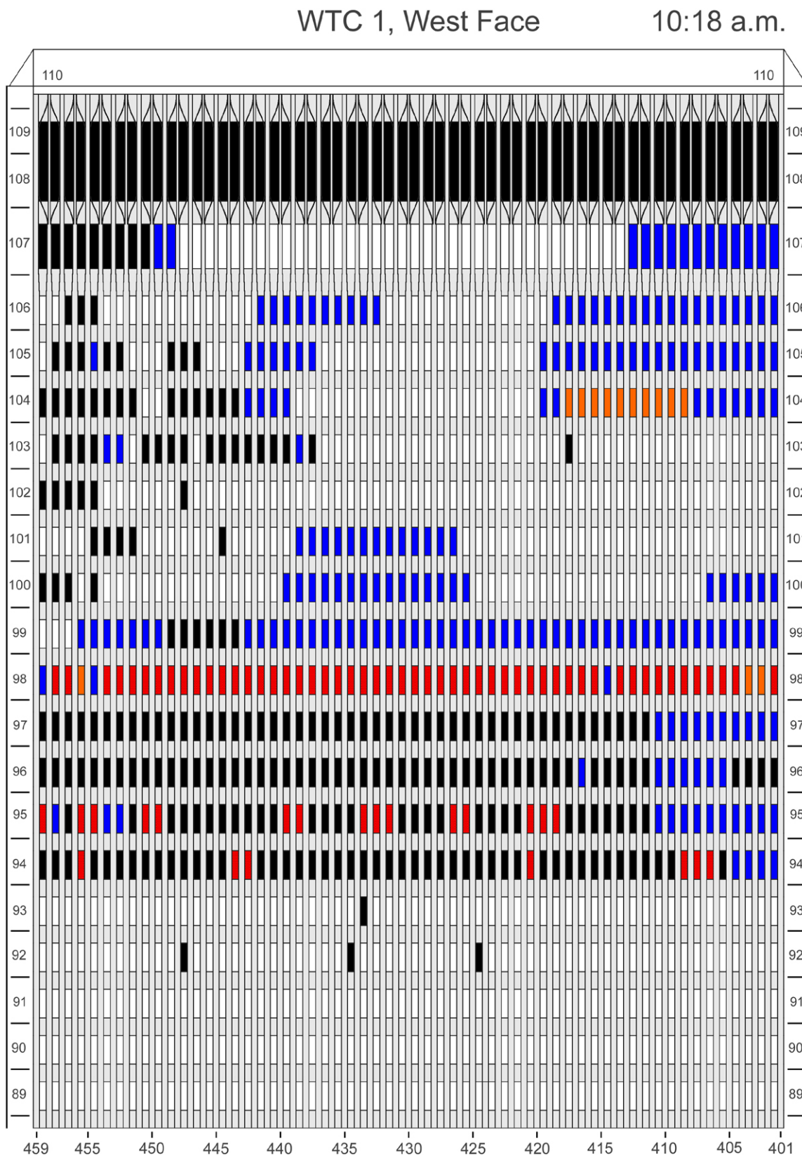
Figure F-57. Diagram of the west face of WTC 1 for floors 89 to 110 at 10:18 a.m. showing the condition of windows and locations of fires.
