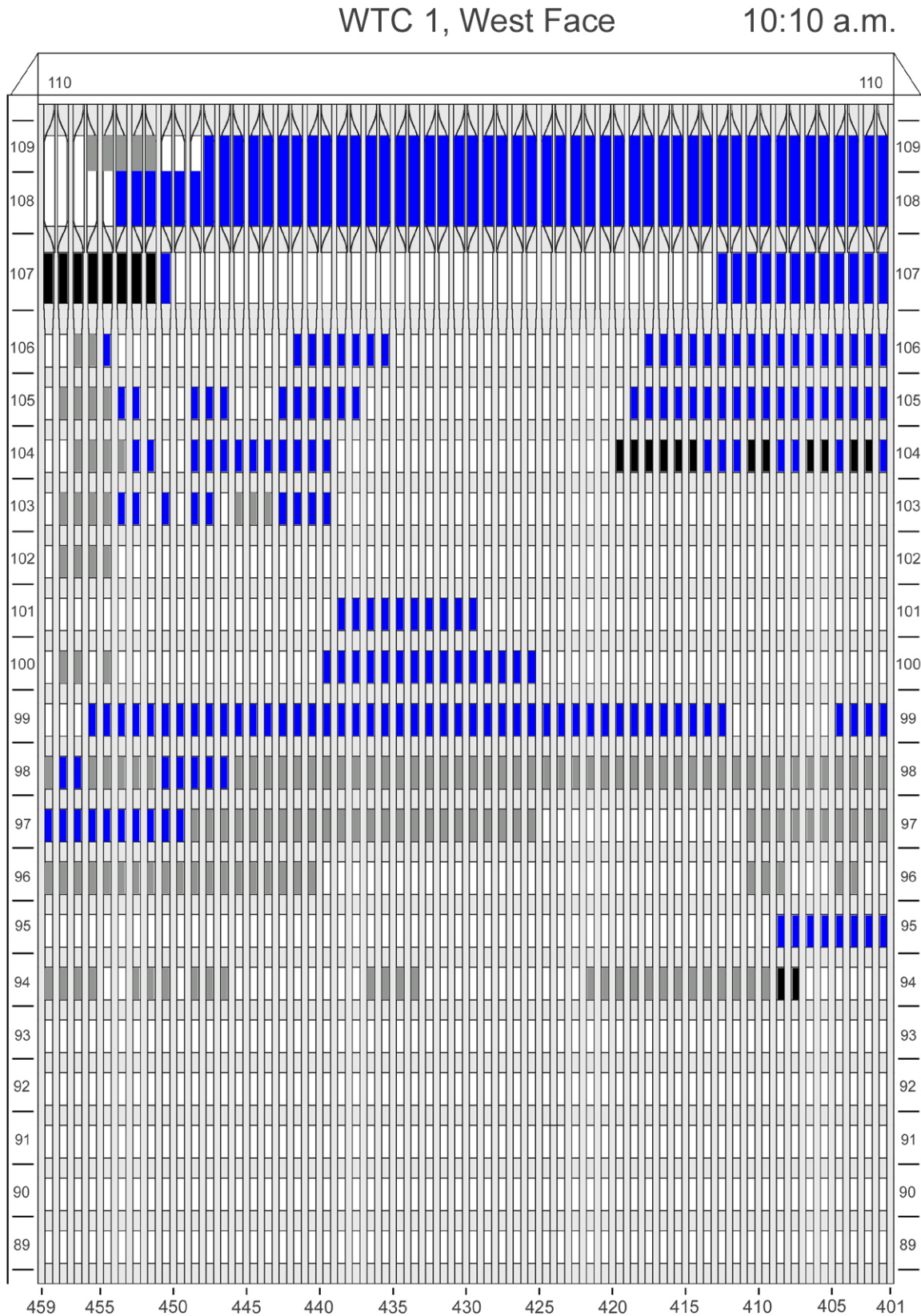
Figure F-54. Diagram of the west face of WTC 1 for floors 89 to 110 at 10:10 a.m. showing windows where smoke was observed and those that were hidden from view.
