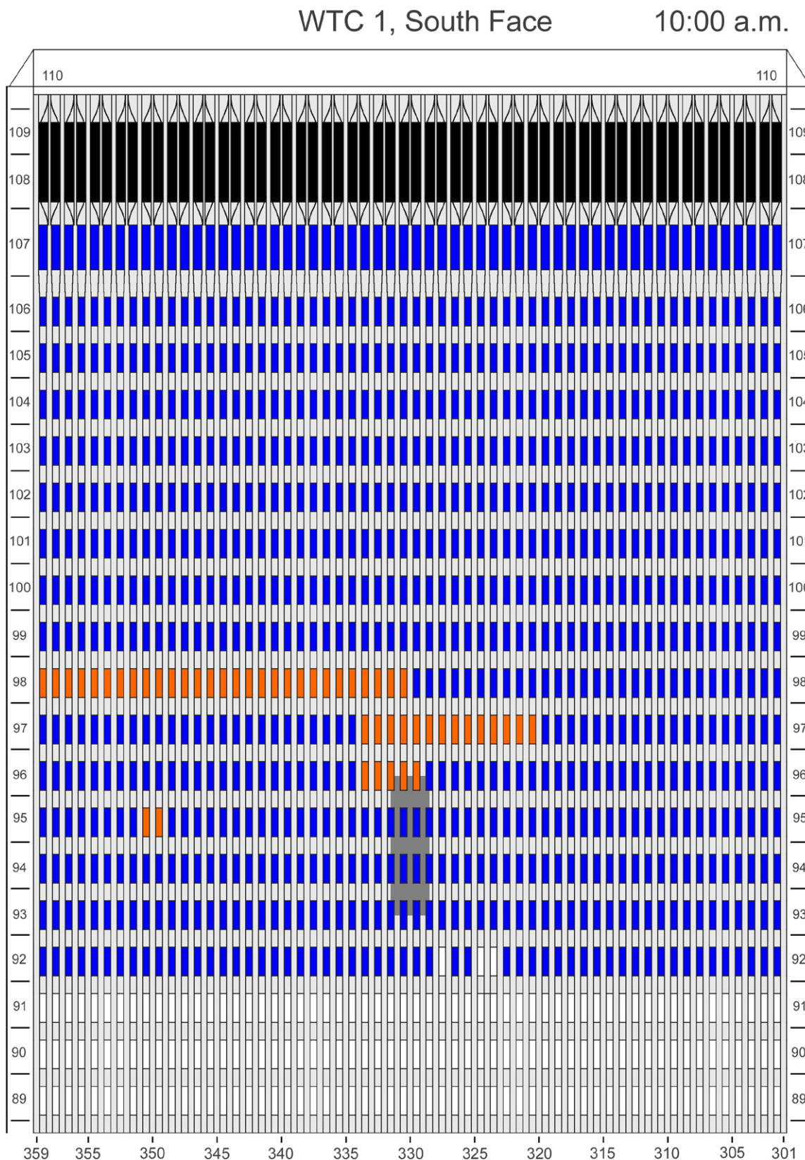
Figure E-37. Diagram of the south face of WTC 1 for floors 89 to 110 at 10:00 a.m. showing the condition of windows and locations of fires.
