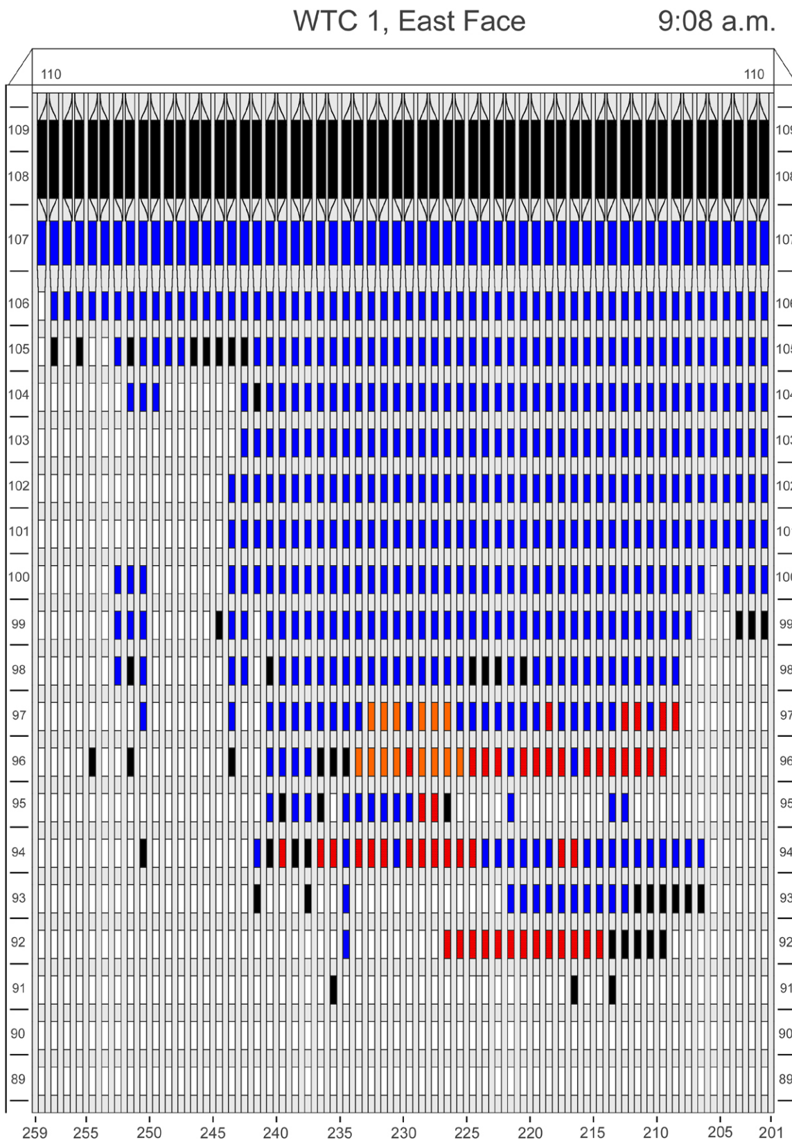
Figure D-13. Diagram of the east face of WTC 1 for floors 89 to 110 at 9:08 a.m. showing the condition of windows and locations of fires.
