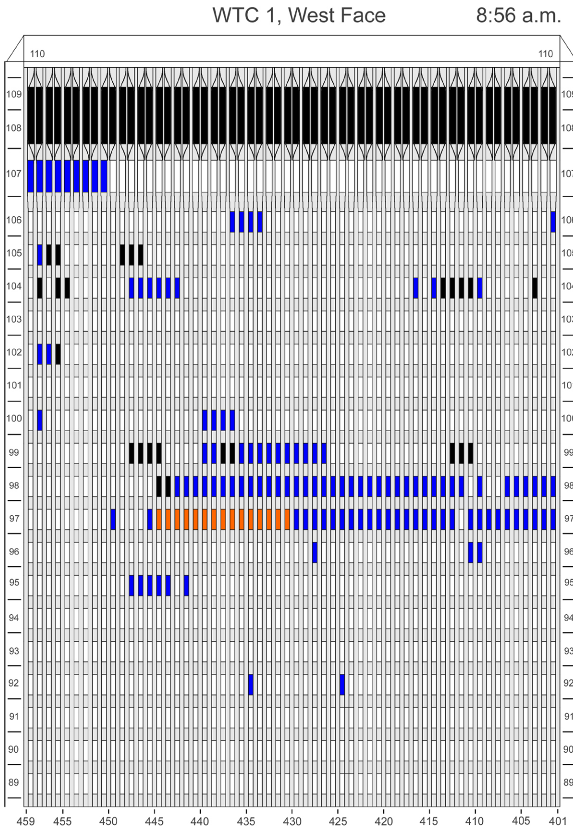
Figure F-11. Diagram of the west face of WTC 1 for floors 89 to 110 at 8:56 a.m showing the condition of windows and locations of fires.
