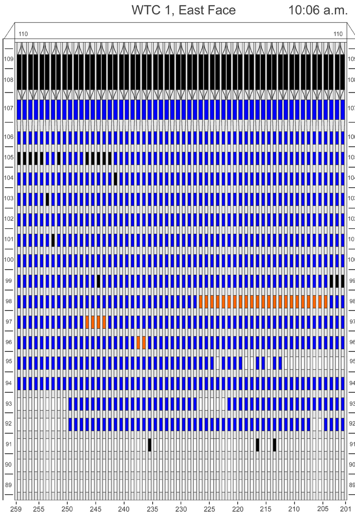
Figure D-41. Diagram of the east face of WTC 1 for floors 89 to 110 at 10:06 a.m. showing the condition of windows and locations of fires.
