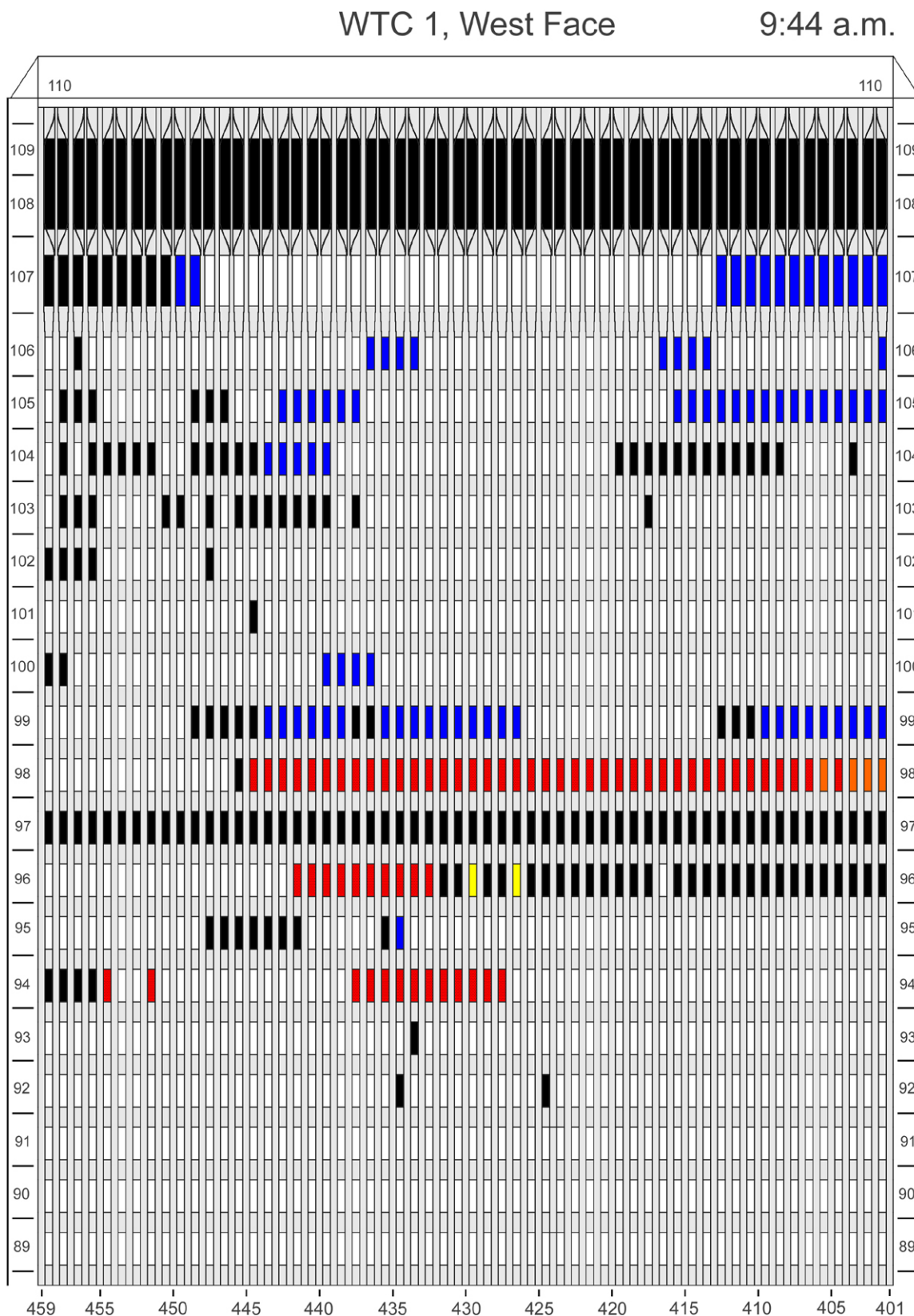
Figure F-41. Diagram of the west face of WTC 1 for floors 89 to 110 at 9:44 a.m. showing the condition of windows and locations of fires.
