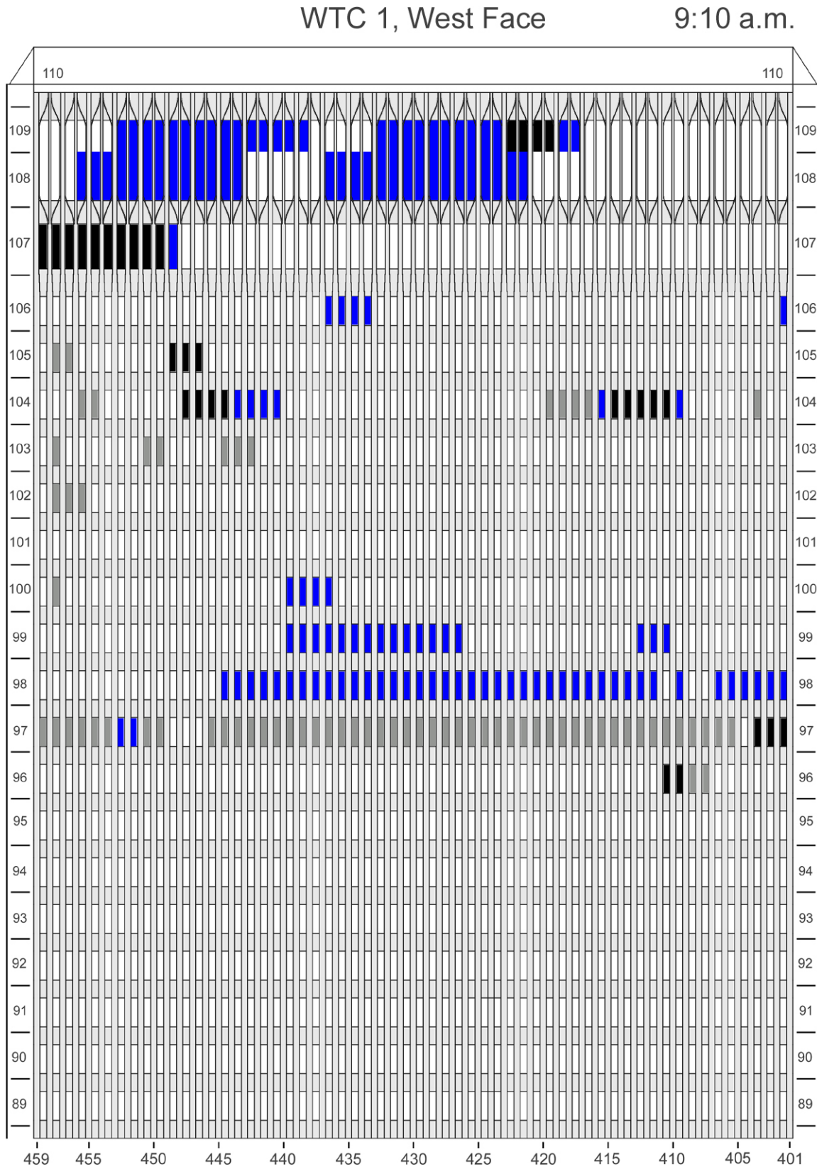
Figure F-26. Diagram of the west face of WTC 1 for floors 89 to 110 at 9:10 a.m. showing windows where smoke was observed and those that were hidden from view.
