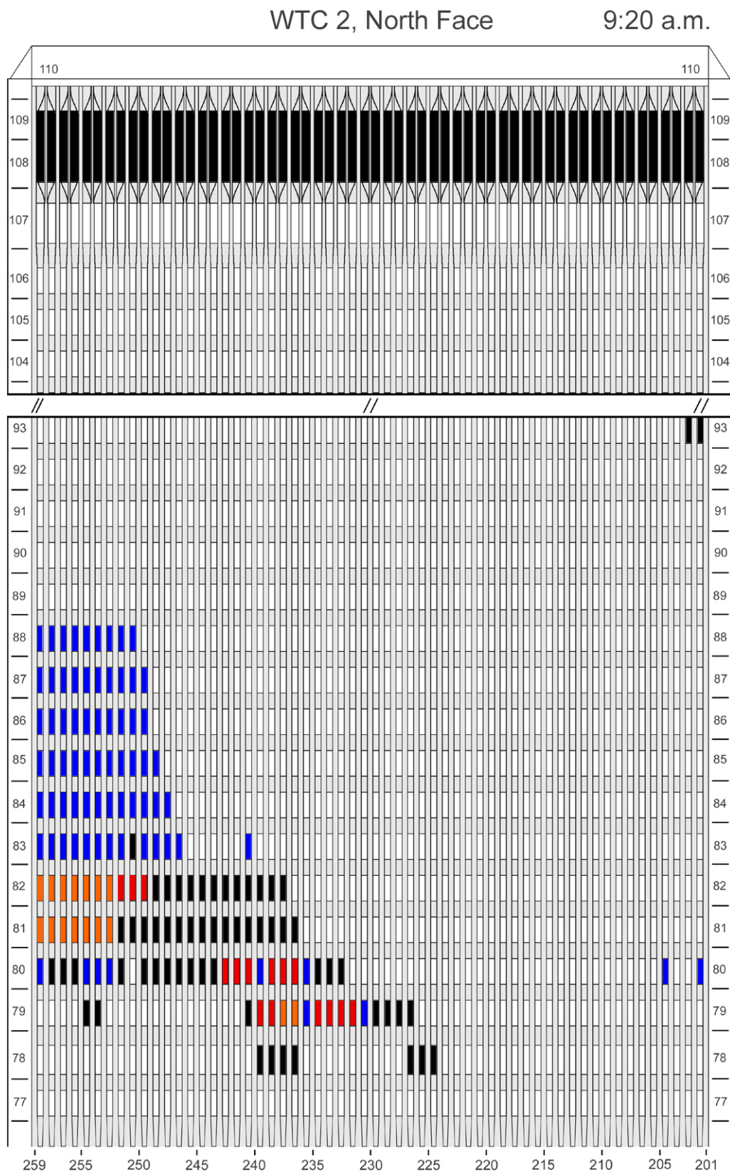
Figure G-19. Diagram of the north face of WTC 2 for floors 77 to 93 and floors 104 to 110 at 9:20 a.m. showing the condition of windows and locations of fires.
