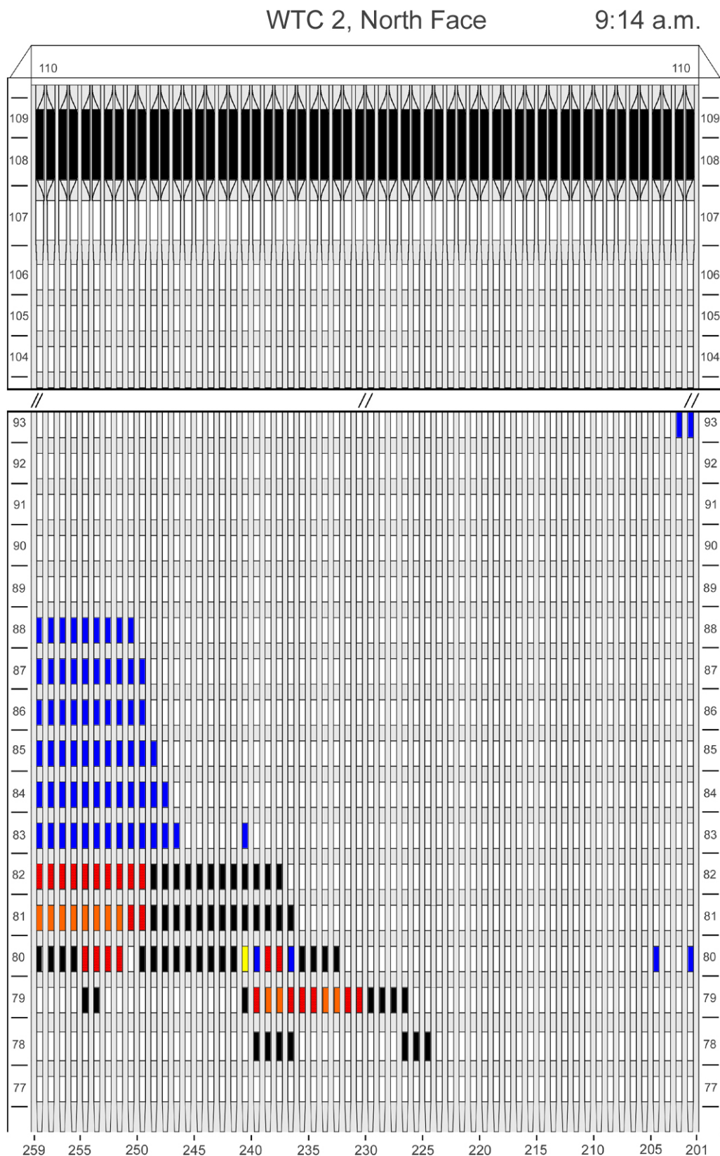
Figure G-13. Diagram of the north face of WTC 2 for floors 77 to 93 and floors 104 to 110 at 9:14 a.m. showing the condition of windows and locations of fires.
