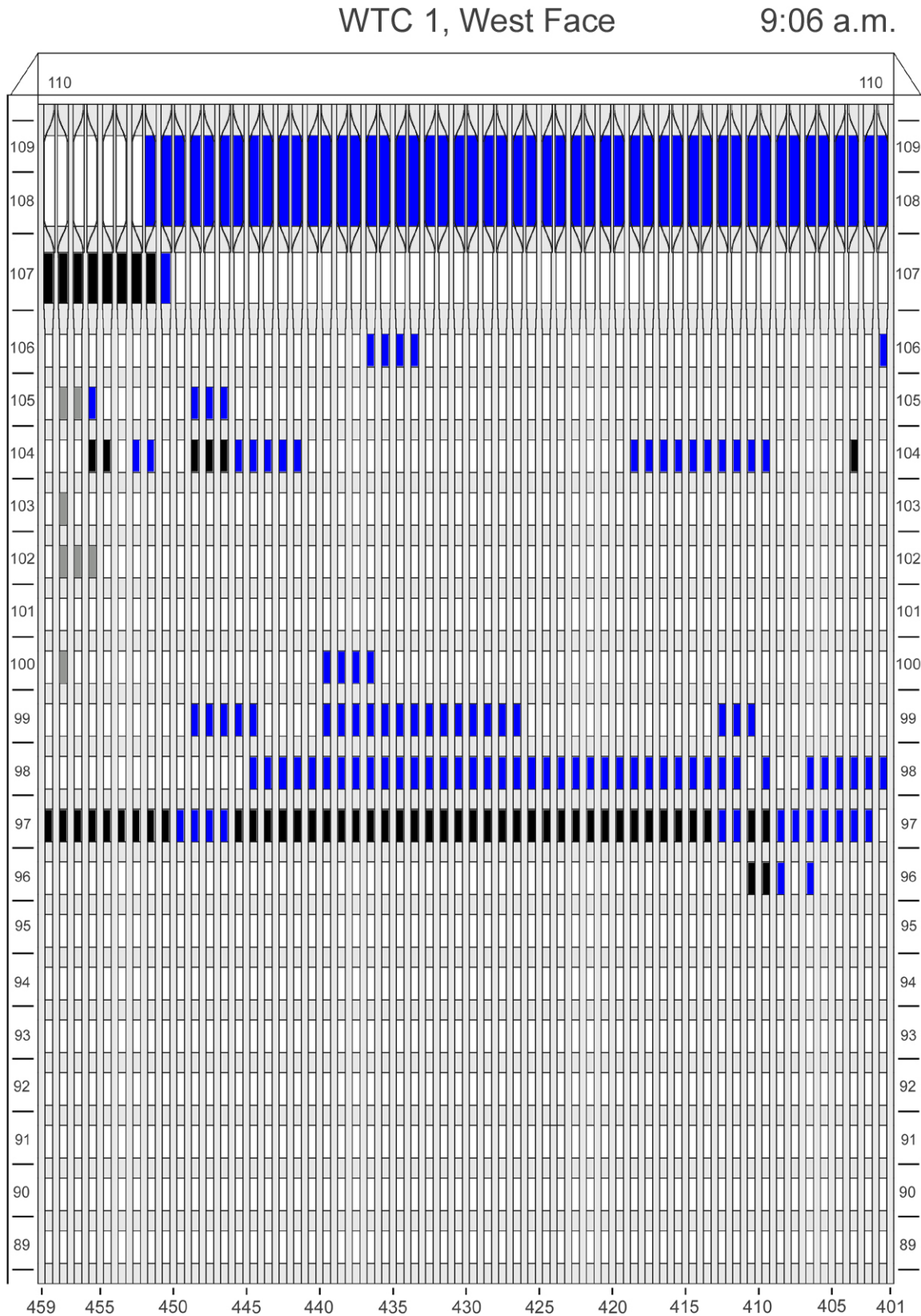
Figure F-22. Diagram of the west face of WTC 1 for floors 89 to 110 at 9:06 a.m. showing windows where smoke was observed and those that were hidden from view.
