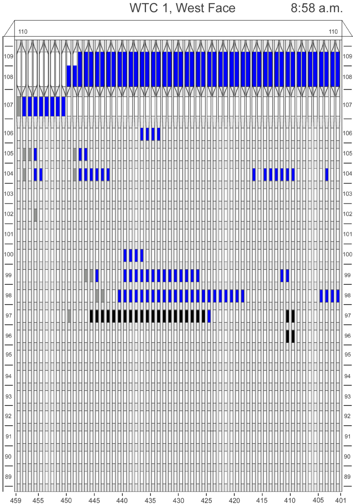
Figure F-14. Diagram of the west face of WTC 1 for floors 89 to 110 at 8:58 a.m. showing windows where smoke was observed and those that were hidden from view.
