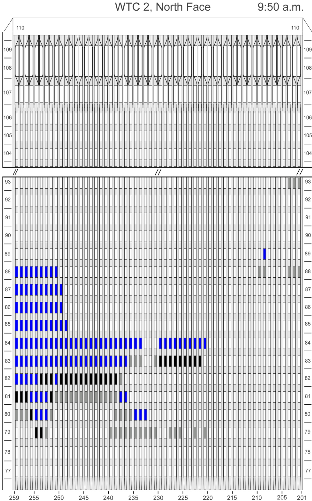
Figure G-50. Diagram of the north face of WTC 2 for floors 77 to 93 and floors 104 to 110 at 9:50 a.m. showing windows where smoke was observed and those hidden from view.
