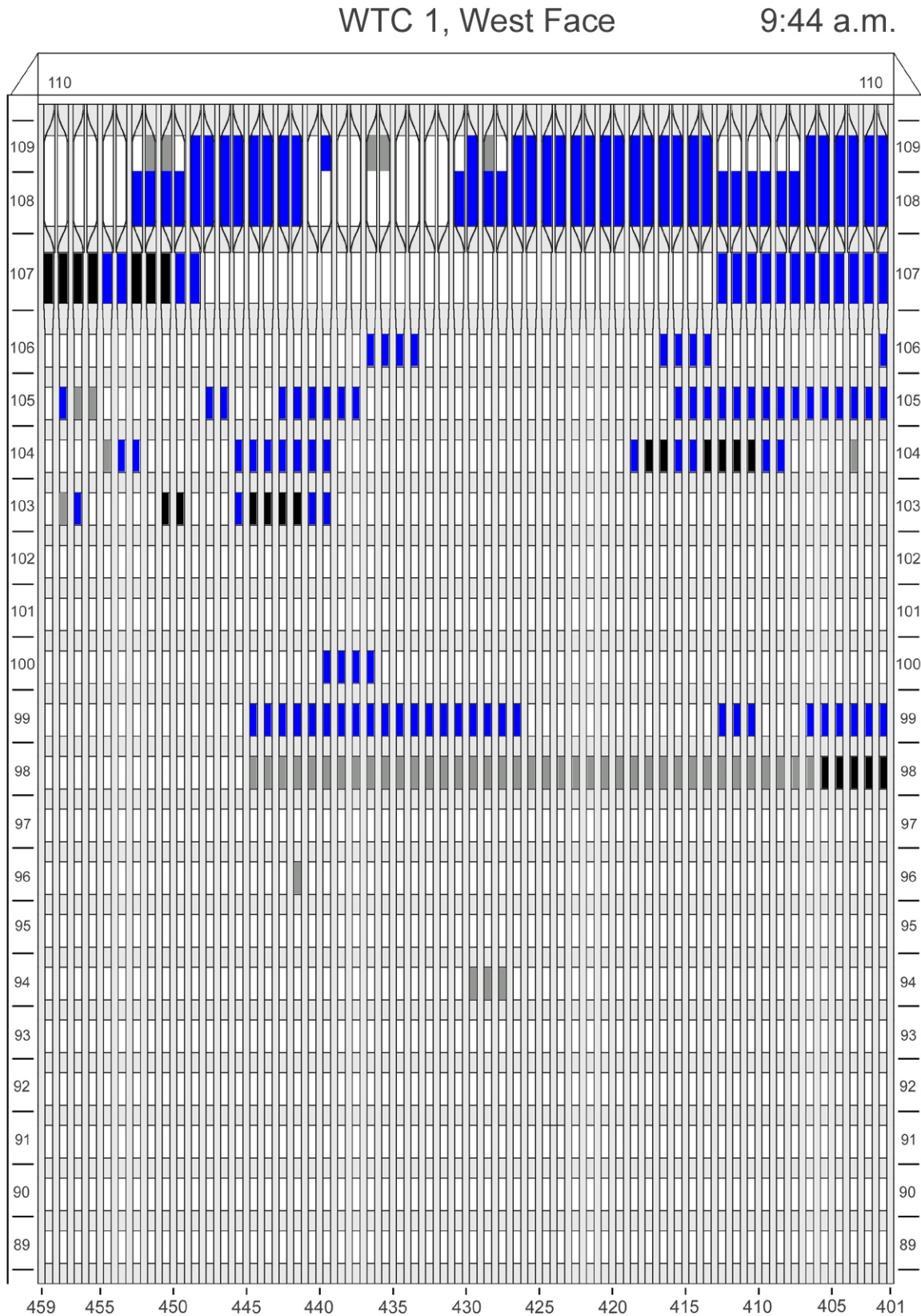
Figure F-42. Diagram of the west face of WTC 1 for floors 89 to 110 at 9:44 a.m. showing windows where smoke was observed and those that were hidden from view.
