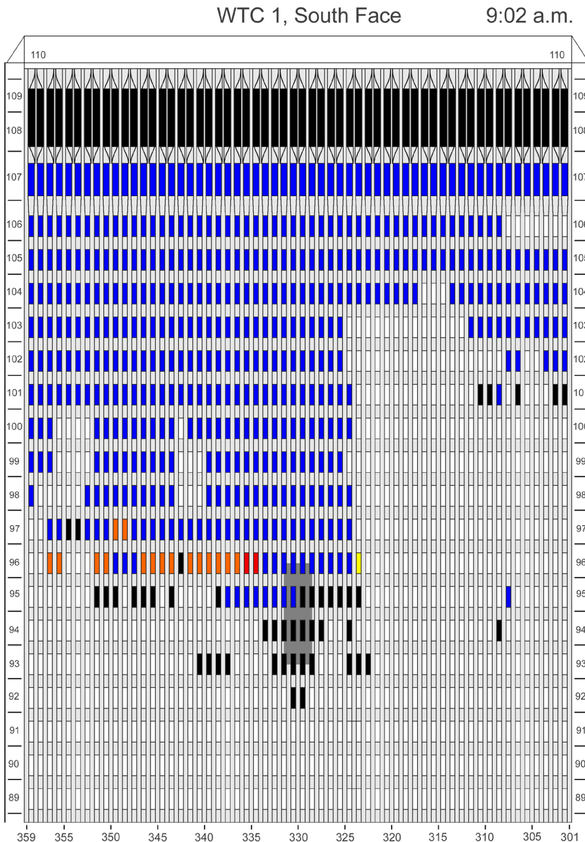
Figure E-9. Diagram of the south face of WTC 1 for floors 89 to 110 at 9:02 a.m. showing the condition of windows and locations of fires.
