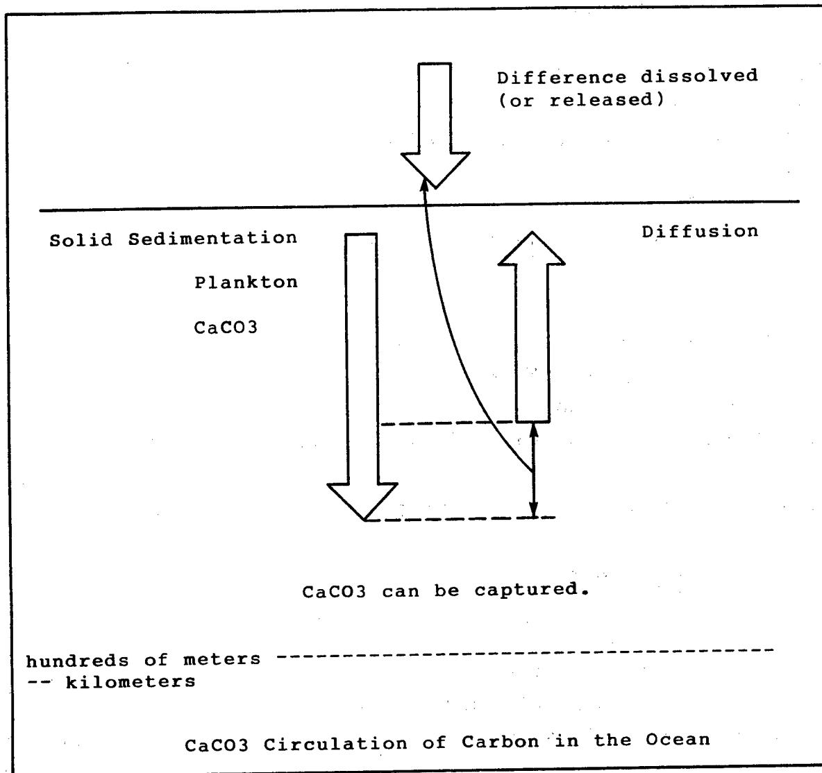
Figure 8-1 Circulation of Carbon in the Ocean
