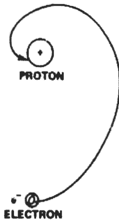
Figure 6. Classical electromagnetic prediction.
