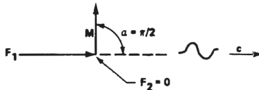
Figure 5. The situation where \alpha = \pi/2 .
