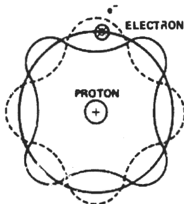
Figure 8. Fourth energy level of the hydrogen atom.
